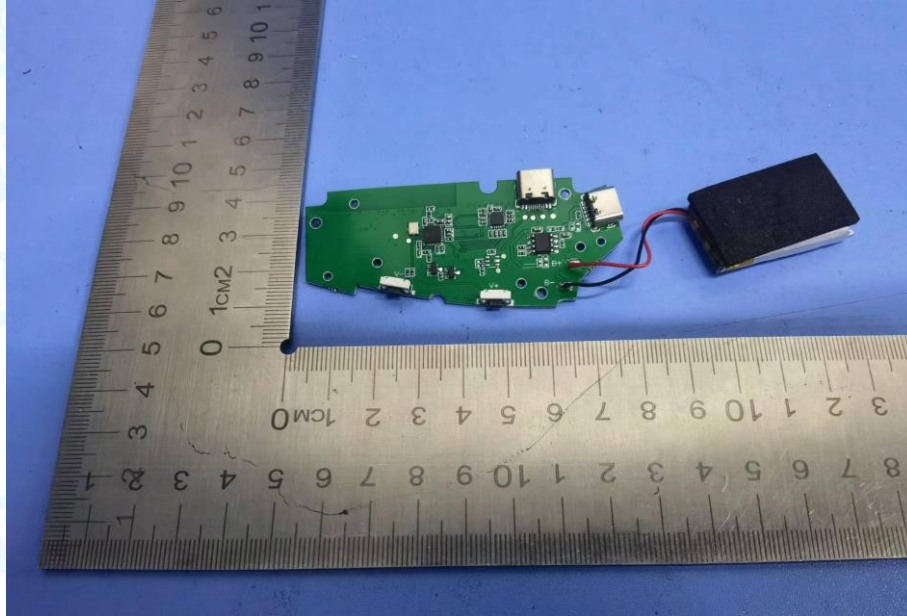
Photo 9 Appearance of PCB & Battery
