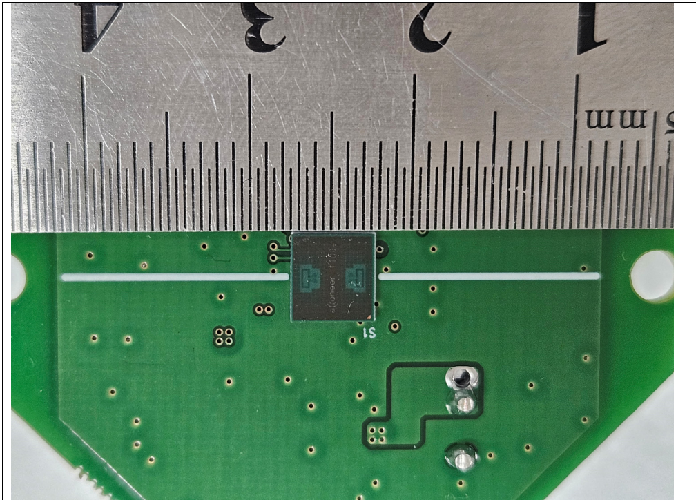
mmW chip and Antenna
