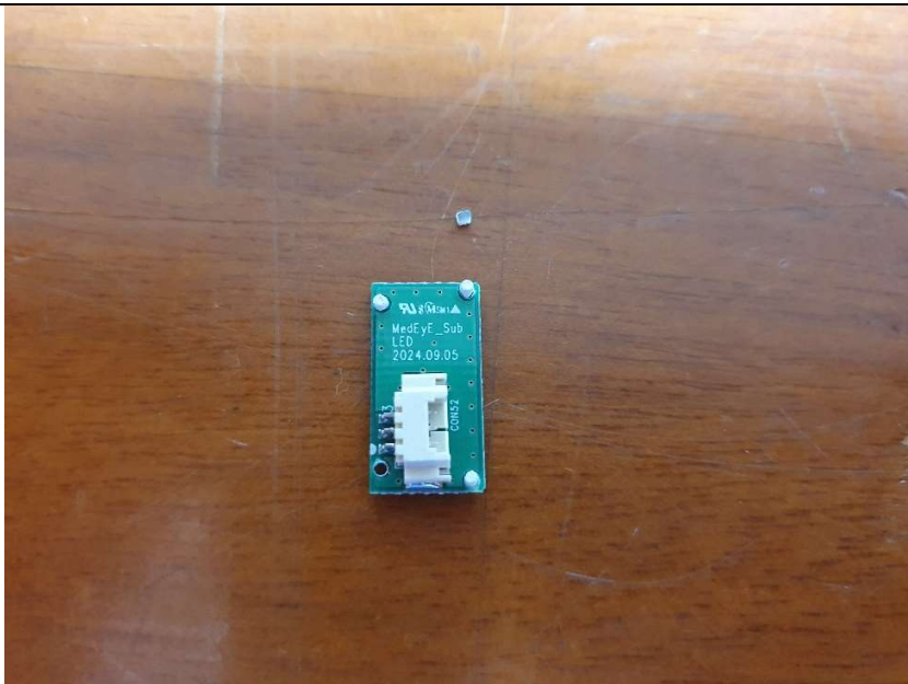
[Rear View of Sub LED board]
