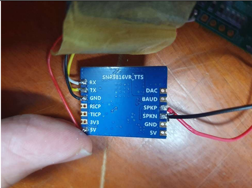
[Rear View of Module]
