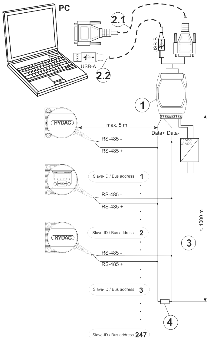
Fig. 18: Connecting / reading out ContaminationSensor via RS485
