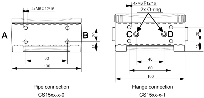
Fig. 5: Unit dimensions CS152x-x-x
