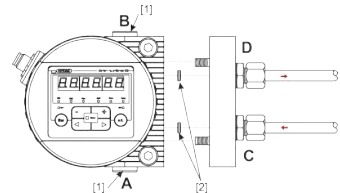
Fig. 11: Flange connection using the example of CS1x2x.
