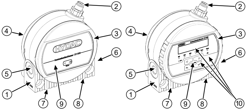
Fig. 7: Components and operating units
