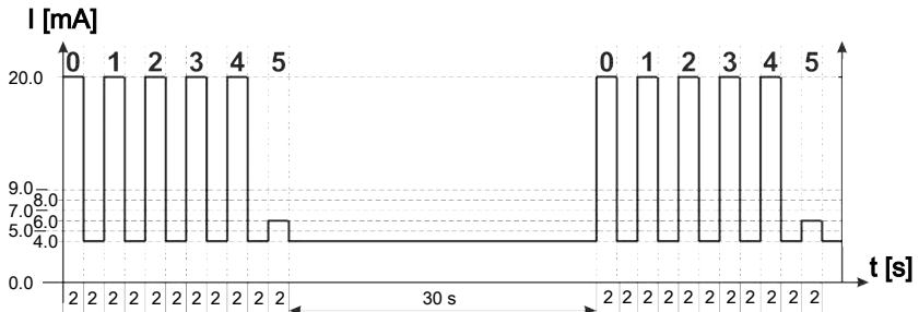
Fig. 41: Example: status of analogue signal 5
