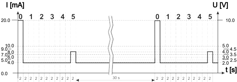
Fig. 24: Example: HDA signal out put of signal 1-4 in accordance with status 5
