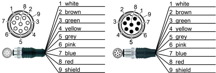
Fig. 45: Colour coding example: M12x1 socket / connector, A coded, 8 pin, shielded
