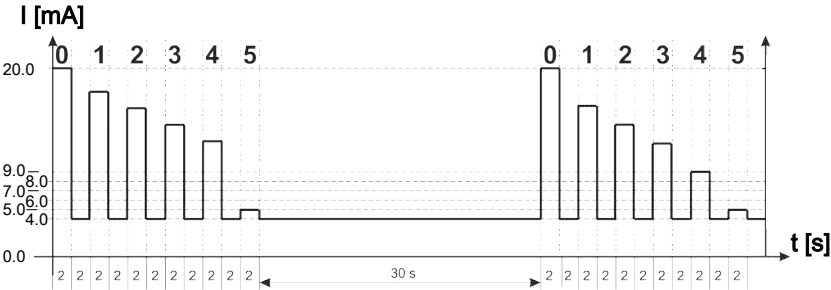
Fig. 40: Example: HDA.NAS analogue output
