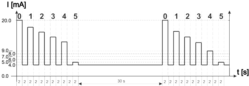
Fig. 34: Example: HDA.ISO analogue output
