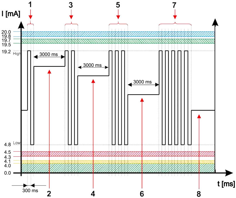
Fig. 21: Example: Analogue output signal SAE+T
