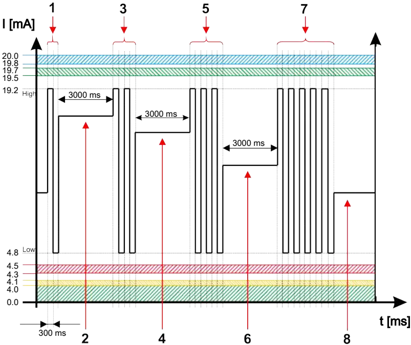
Fig. 27: Example: Analogue output signal ISO+T
