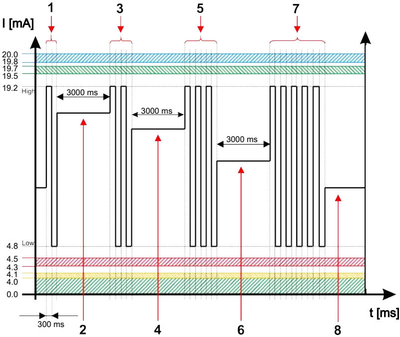
Fig. 33: Example: Analogue output signal ISO+T
