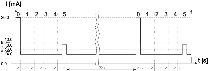
Fig. 42: Example: HDA signal output of signal 1-4 in accordance with status 5
