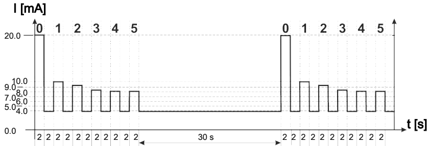
Fig. 36: Example: HDA signal output of signal 1-4 in accordance with status 5
