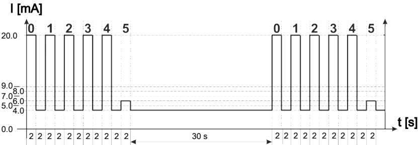
Fig. 43: Example: status of analogue signal 5
