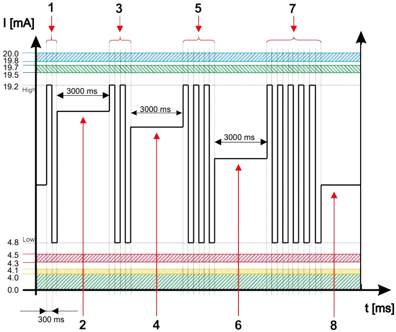
Fig. 39: Example: Analogue output signal NAS+T
