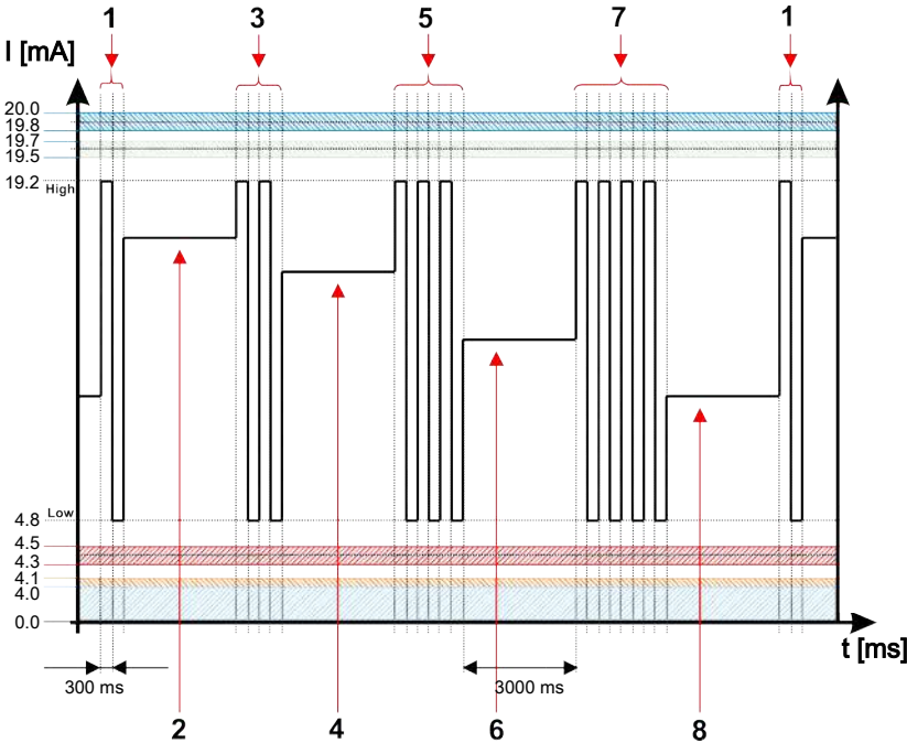
Fig. 37: Example: Analogue output signal NAS classes 2-5 µm / 5-15 µm / 15-25 µm / ≥ 25 µm, time-coded
