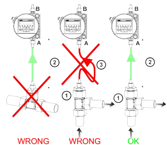
Fig. 13: Finding a measuring point in the hydraulic system
