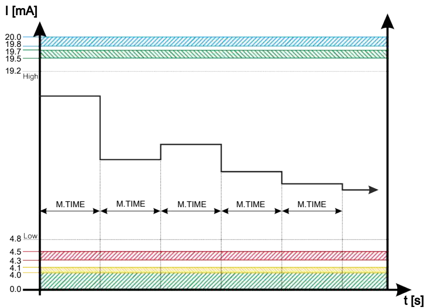
Fig. 20: Example: Analogue output signal class SAE A / SAE B / SAE C or SAE D
