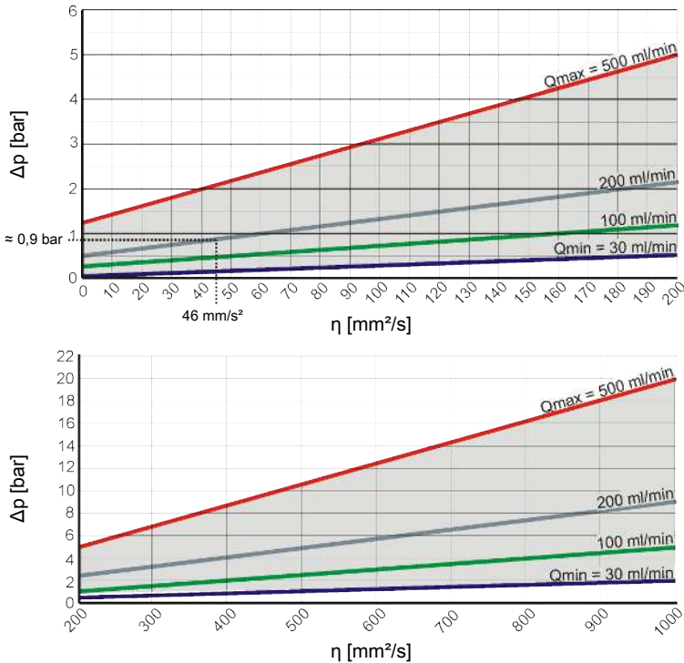
Fig. 12: Flow rate, differential pressure and viscosity characteristics
