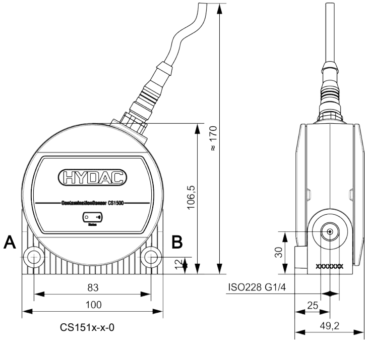
Fig. 4: Unit dimensions CS151x-x-x
