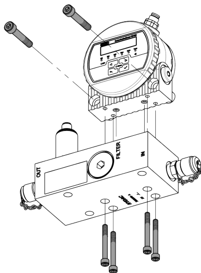
Fig. 9: Mounting on a sub plate with flange connection
