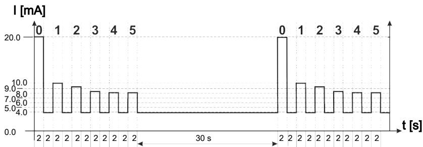
Fig. 30: Example: HDA signal output of signal 1-4 in accordance with status 5
