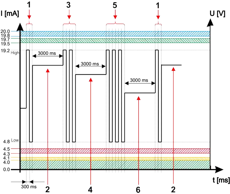
Fig. 26: Example: Analogue output signal ISO code, time-coded
