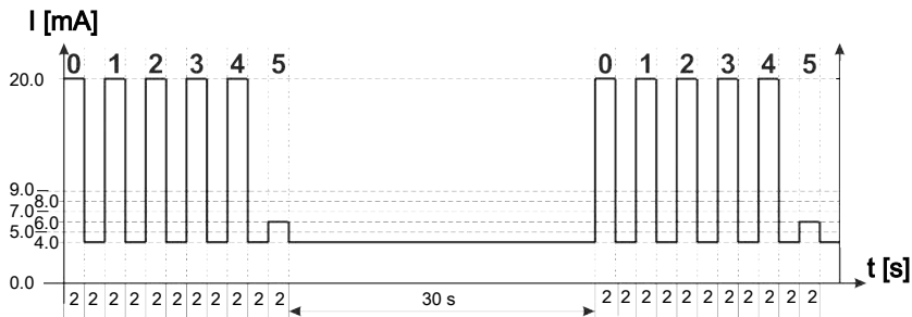
Fig. 29: Example: status of analogue signal 5
