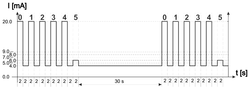
Fig. 35: Example: status of analogue signal 5
