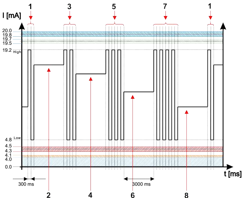
Fig. 19: Example: Analogue output signal SAE classes A/B/C/D, time-coded
