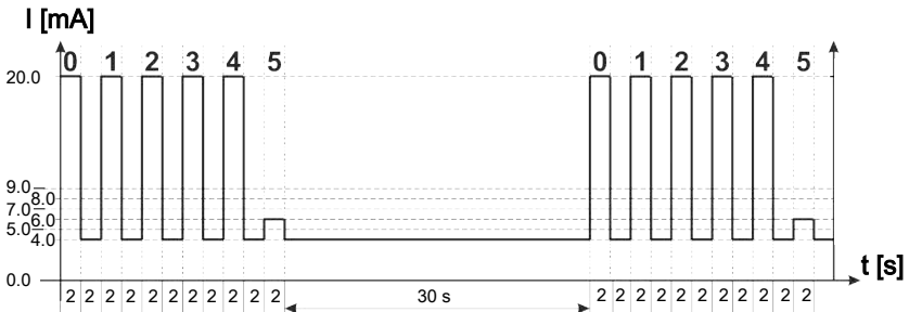
Fig. 23: Example: status of analogue signal 5
