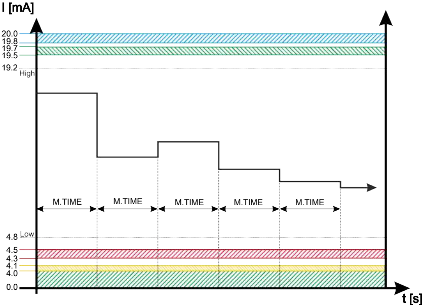
Fig. 38: Example: Analogue output signal class NAS 2 / NAS 5 / NAS 15 or NAS 25
