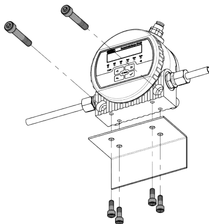
Fig. 8: Mounting on a wall or bracket
