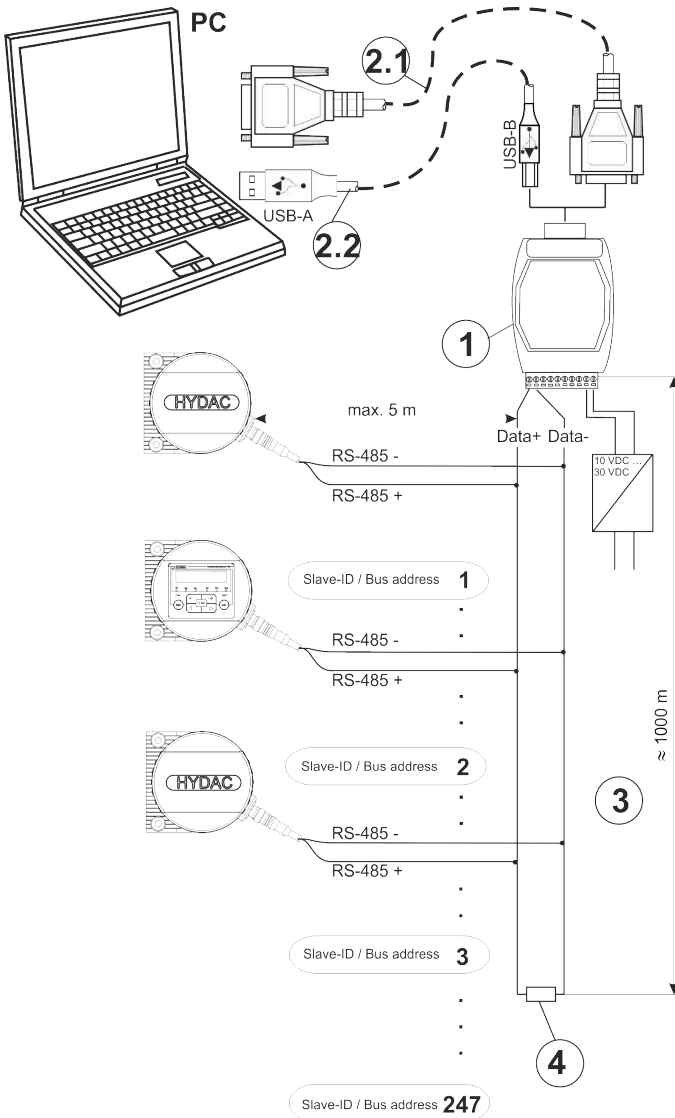
Fig. 14: Connection example CS15xx-1-...
