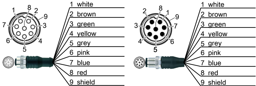
Socket Male connector Fig. 18: Colour coding example: M12x1 socket / connector, A coded, 8 pin, shielded
