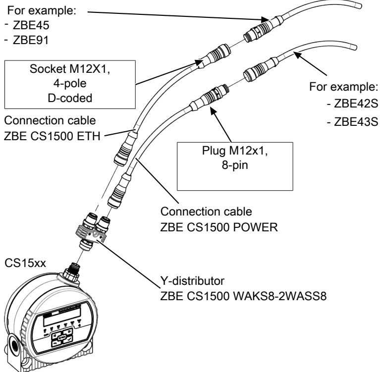
Fig. 14: Connection example CS15xx-0-...
