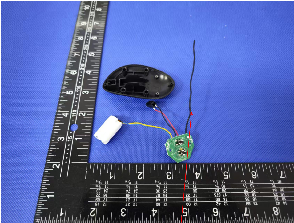
Internal antenna
