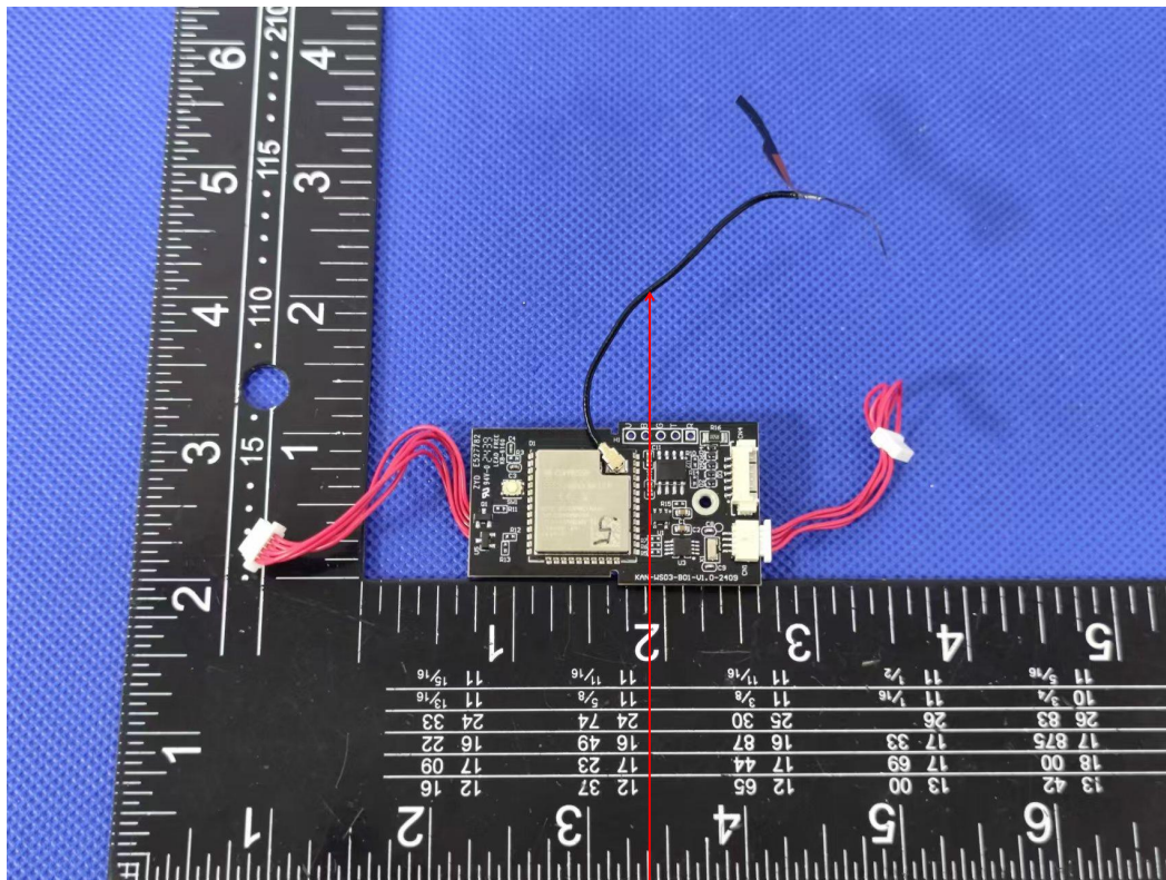
FPC antenna
