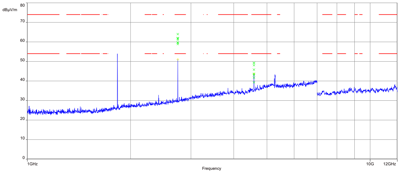
Plot 2: TX mode 916.0 MHz, 2m cable length,, 1 GHz – 12 GHz, horizontal &amp; vertical polarisation
