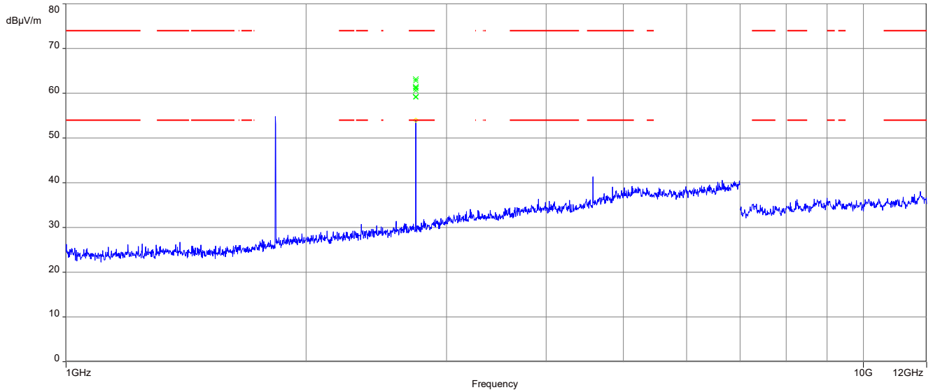
Plot 1: TX mode 915.4 MHz, 2m cable length, 1 GHz – 12 GHz, horizontal &amp; vertical polarisation
