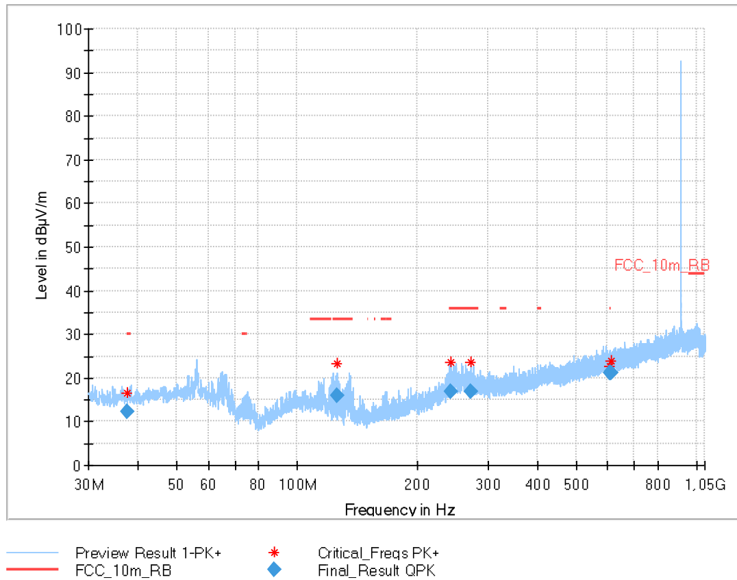
Plot 2: TX mode 916.0 MHz, 30 MHz – 1 GHz, horizontal &amp; vertical polarisation
