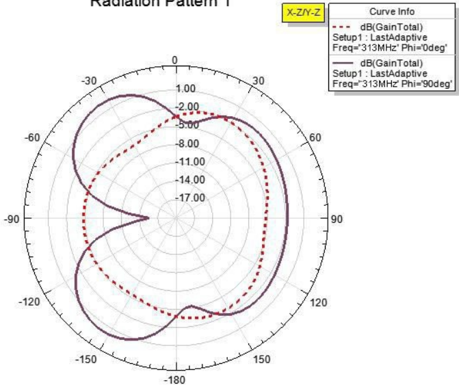
Radiation Pattern 1
