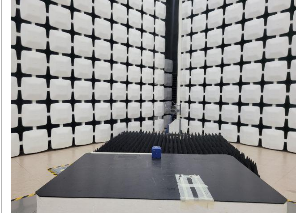
Radiated Emission (Above 1 GHz)_Front
