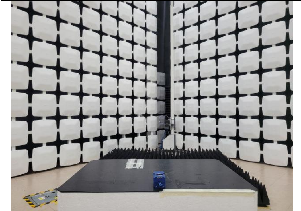
Radiated Emission (Above 1 GHz)_Rear
