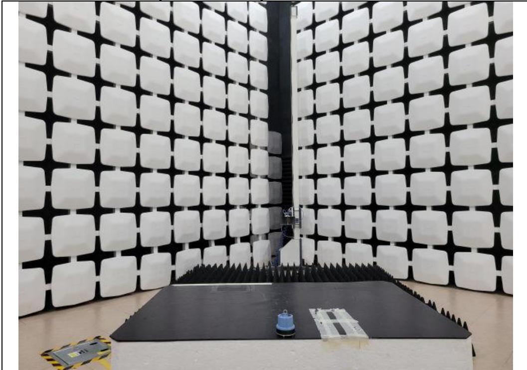
Radiated Emission (Above 1 GHz) Normal Mode Rear
