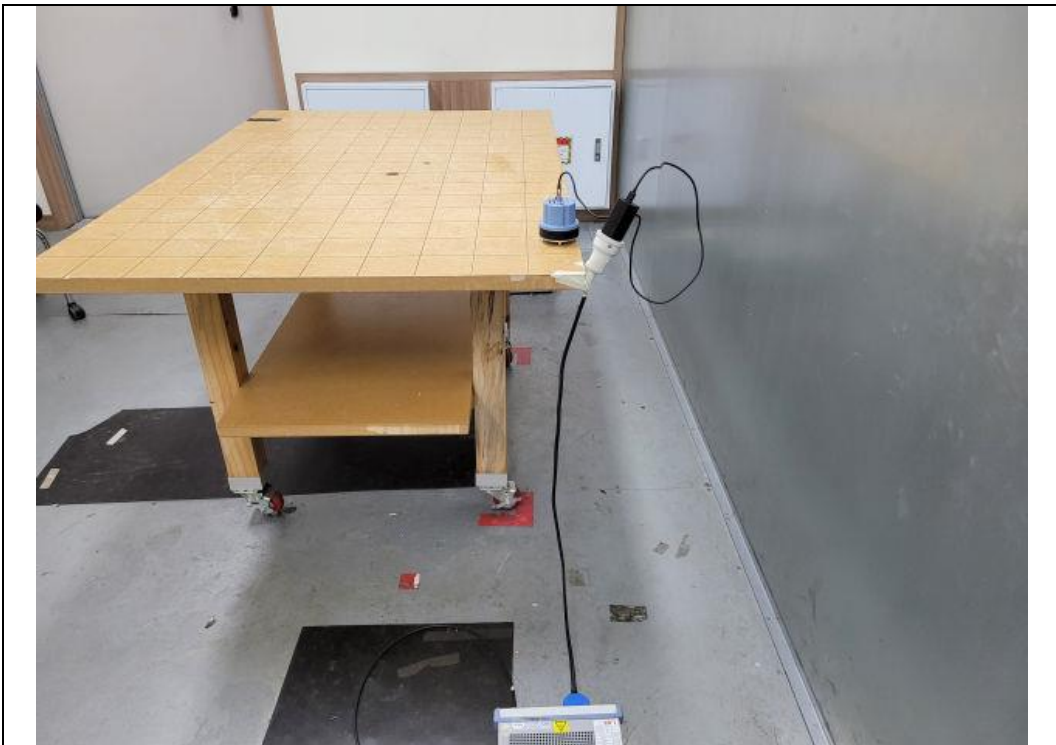
Conducted Emission_Charge+Operating Mode Rear
