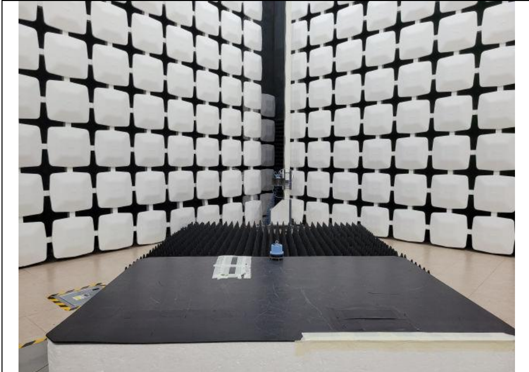
Radiated Emission (Above 1 GHz) Normal Mode Front
