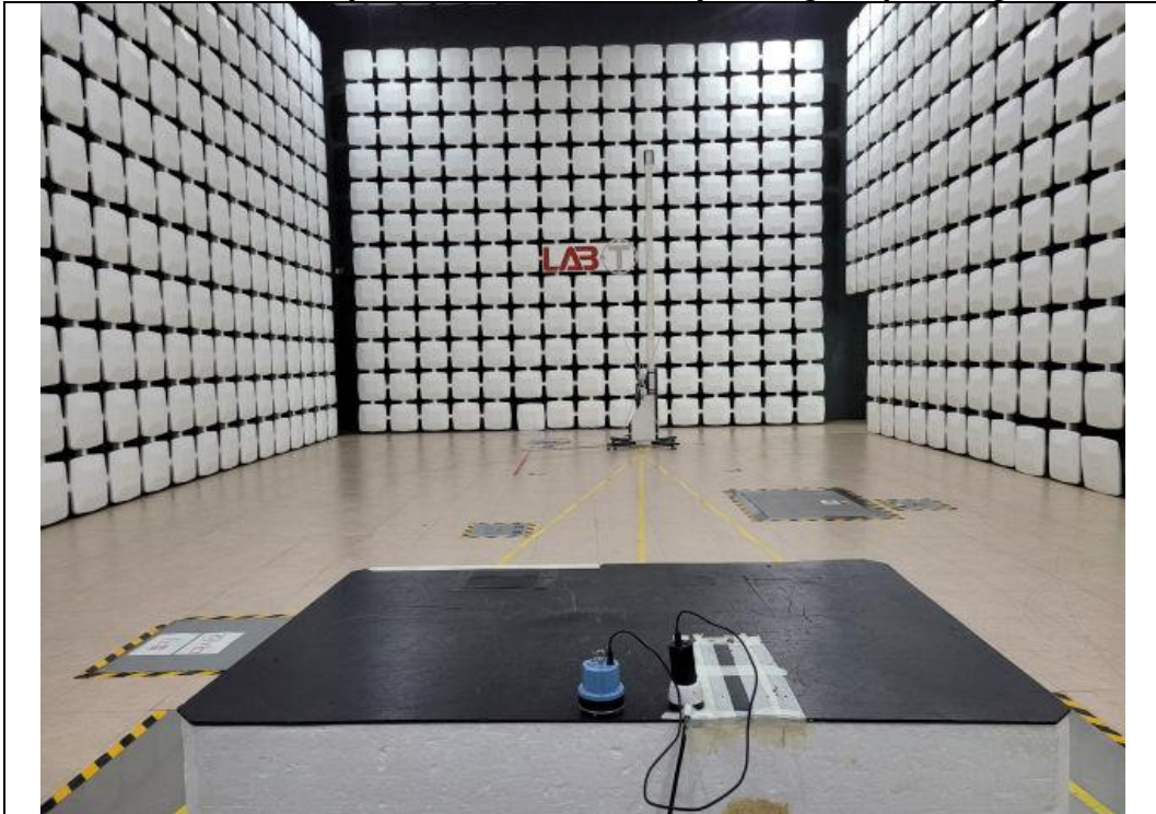
Radiated Emission (30 MHz to 1 000 MHz)_ Charge+Operating Mode Rear
