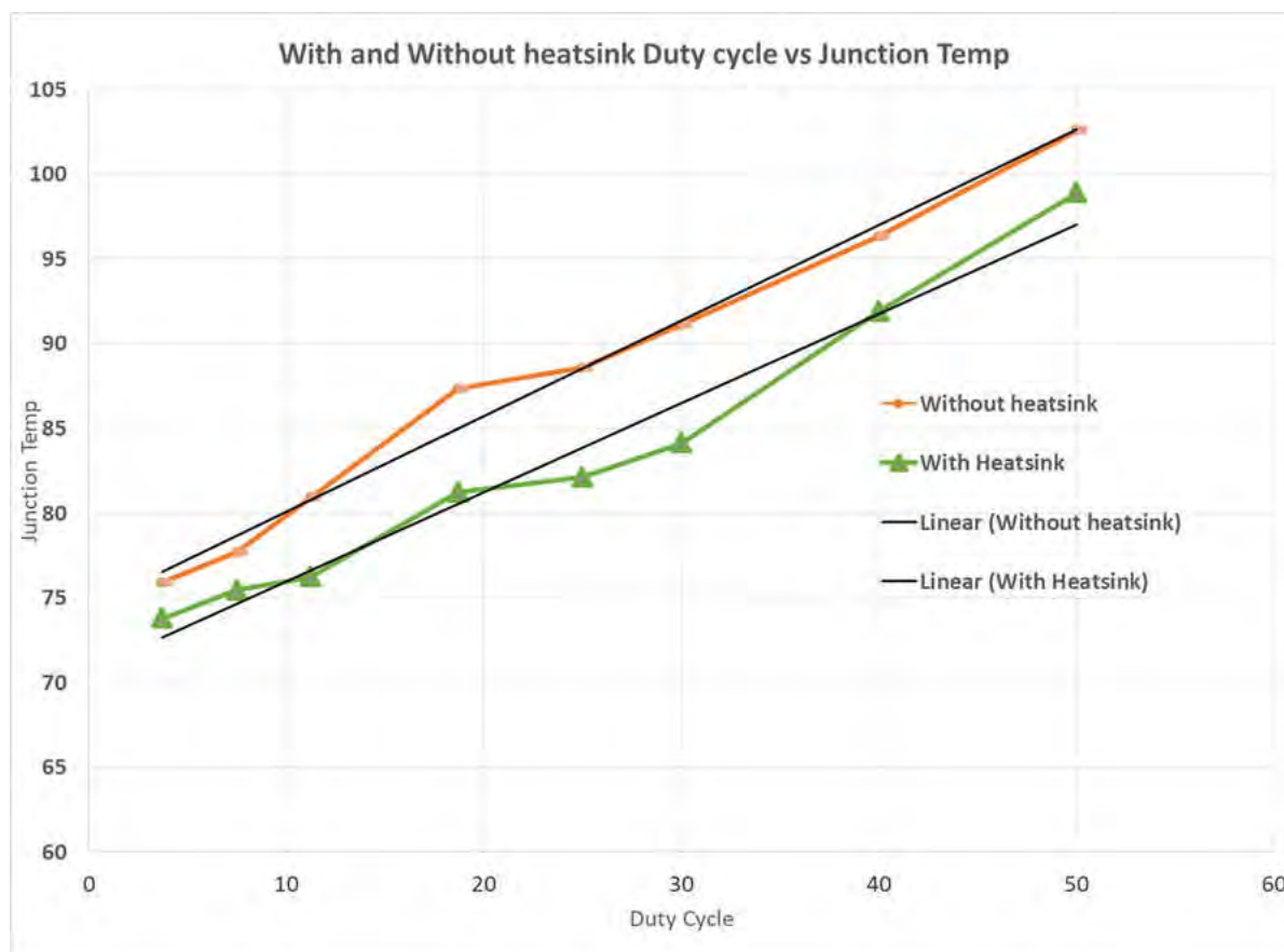
Figure 4-4. Duty Cycle versus Junction Temperature
