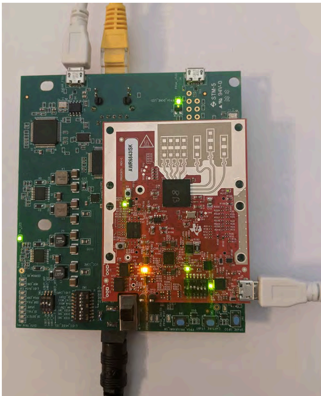
Figure 3-22. DCA1000EVM mode
