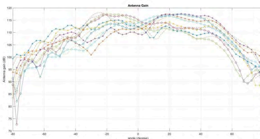
Figure 7-6. Measured Elevation Radiation Pattern for All Tx to Rx Pairs (All 12 Virtual Antenna Pairs Included)
