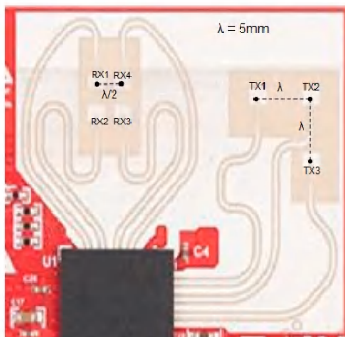
Figure 3-17. IWR6843ISK-ODS antenna placement MIMO array
