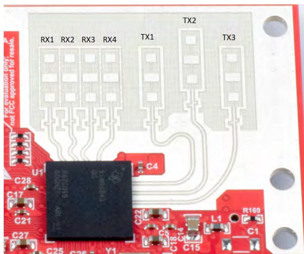
Figure 6-7. PCB Antennas
