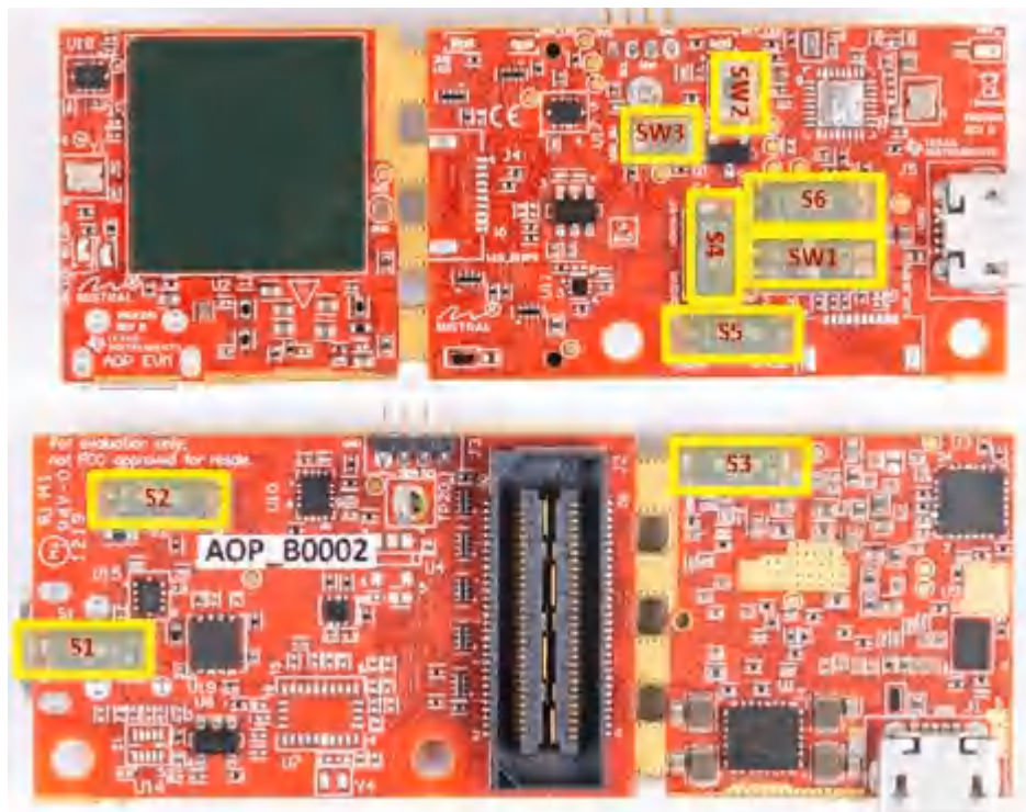
Figure 7-7. IWR6843AOPEVM Switches
