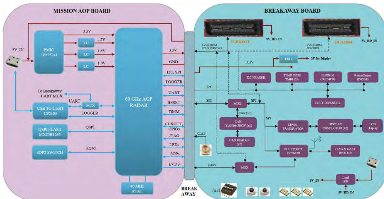
Figure 4-3. Block Diagram of the xWR6843AOPEVM
