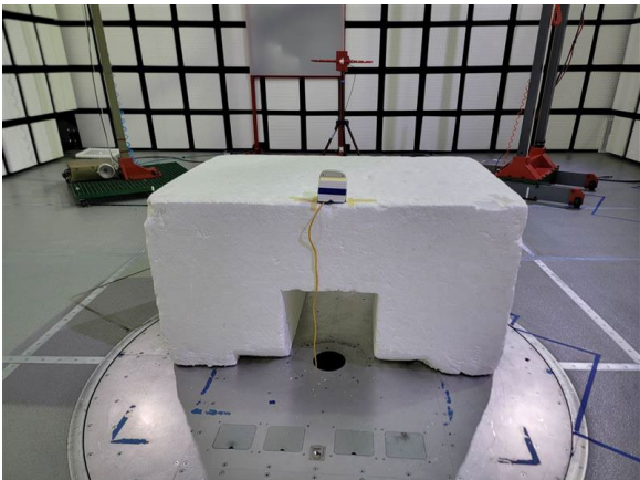
Back – rx antenna flat
