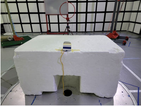
Back – rx antenna at 0 Deg
