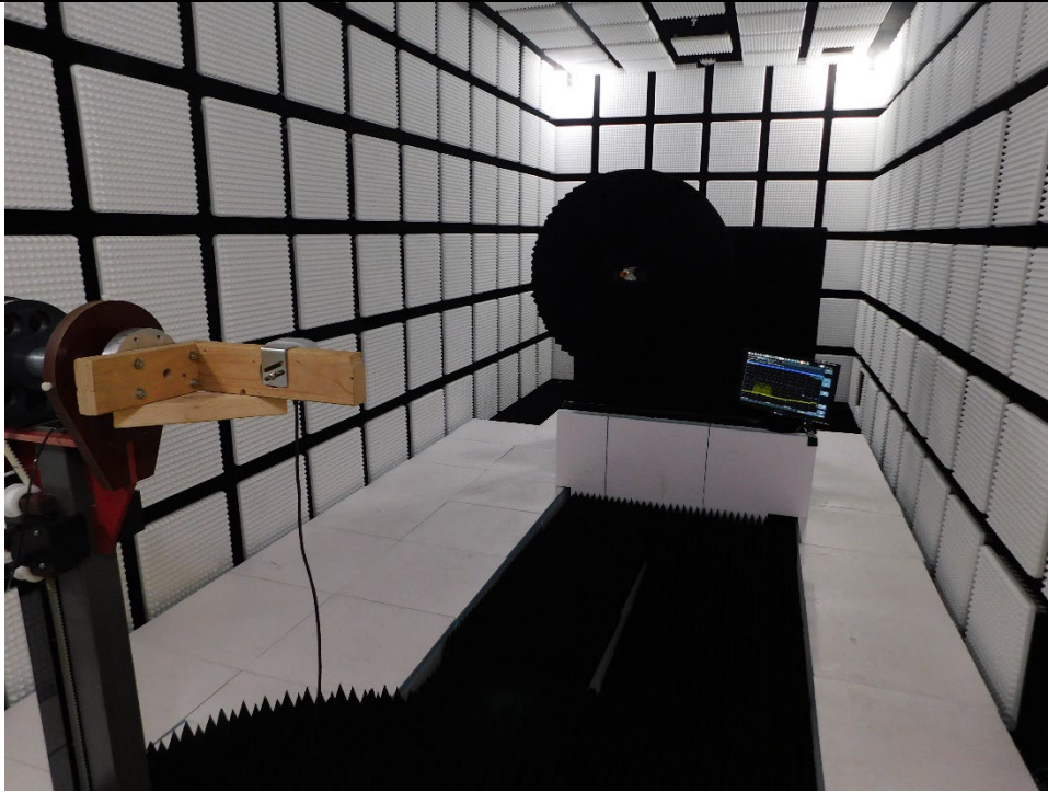
Above 18 GHz Back
