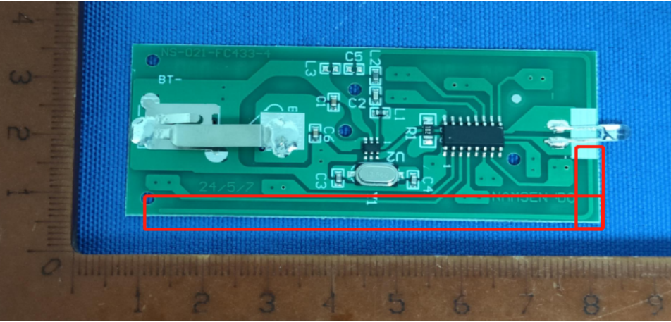
Antenna size: 68mm*15mm
