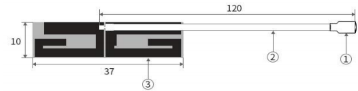
Antenna Photo & Length (mm)
