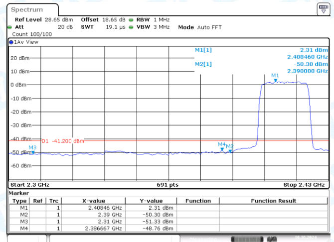
11AX20MIMO-Ant2-2412-PASS
