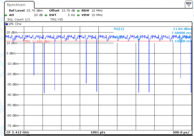
NTVN-11AX20MIMO-Ant2-2412
