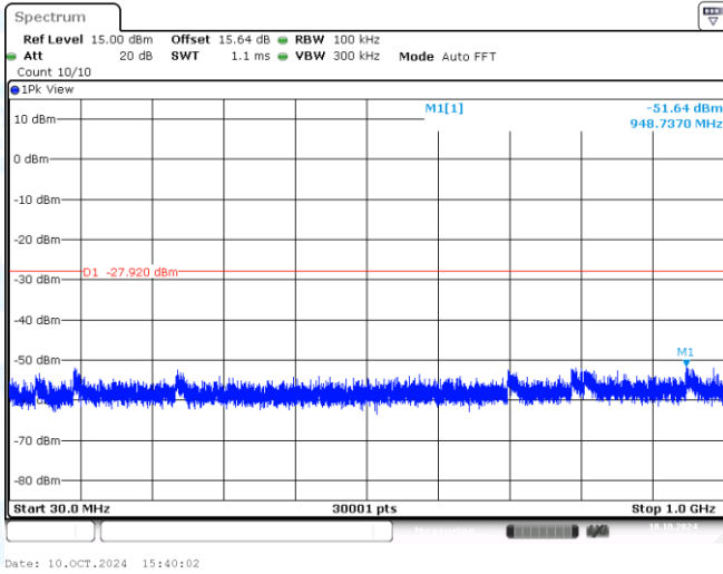
11AX20MIMO-Ant1-2462-30~1000-PASS
