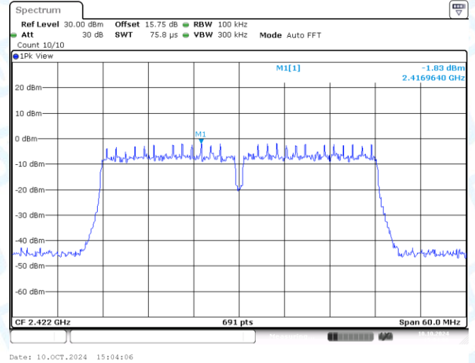
11N40MIMO-Ant2-2422-0~Reference-PASS
