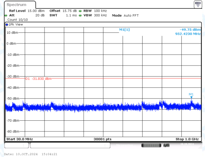
11N40MIMO-Ant2-2422-30~1000-PASS
