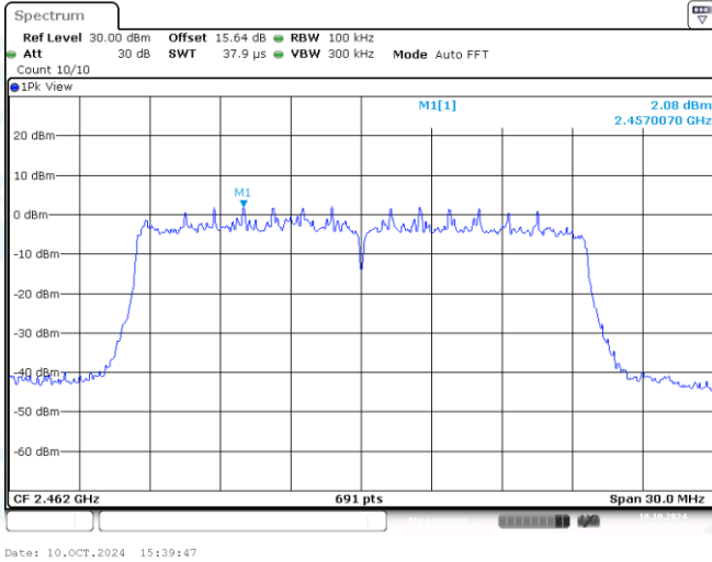
11AX20MIMO-Ant1-2462-0~Reference-PASS
