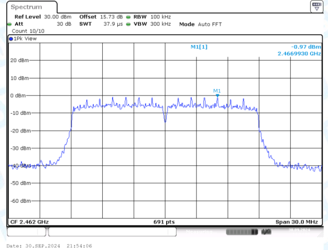
11N20MIMO-Ant2-2462-0~Reference-PASS
