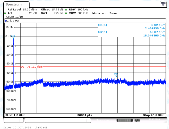
11AX40MIMO-Ant2-2422-1000~26500-PASS
