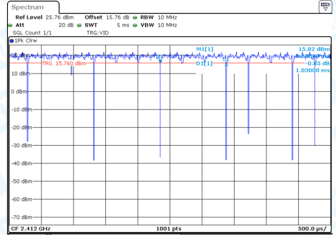
NTNV-11G-CDD-Ant2-2412
