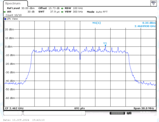
11AX20MIMO-Ant2-2462-0~Reference-PASS
