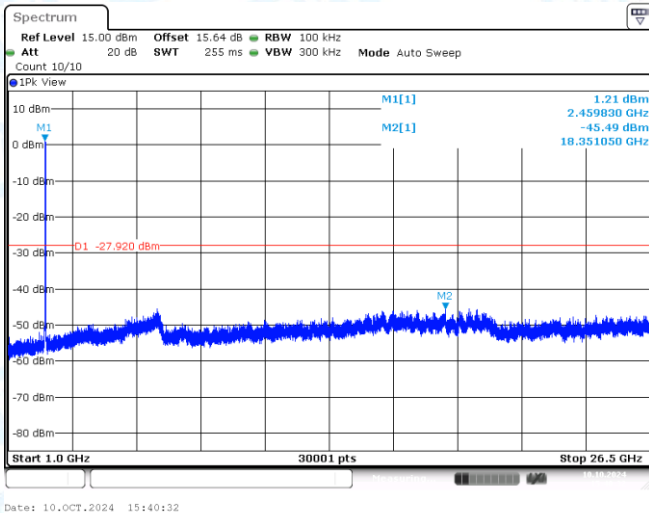
11AX20MIMO-Ant1-2462-1000~26500-PASS
