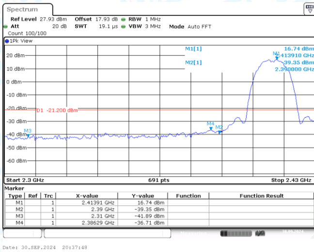
11B-CDD-Ant1-2412-PASS
