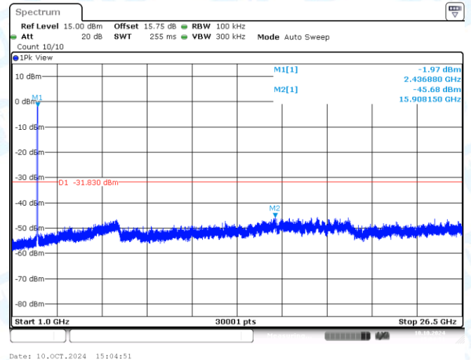
11N40MIMO-Ant2-2422-1000~26500-PASS
