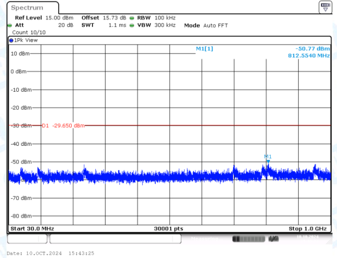
11AX20MIMO-Ant2-2462-30~1000-PASS
