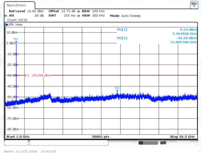
11AX20MIMO-Ant2-2462-1000~26500-PASS
