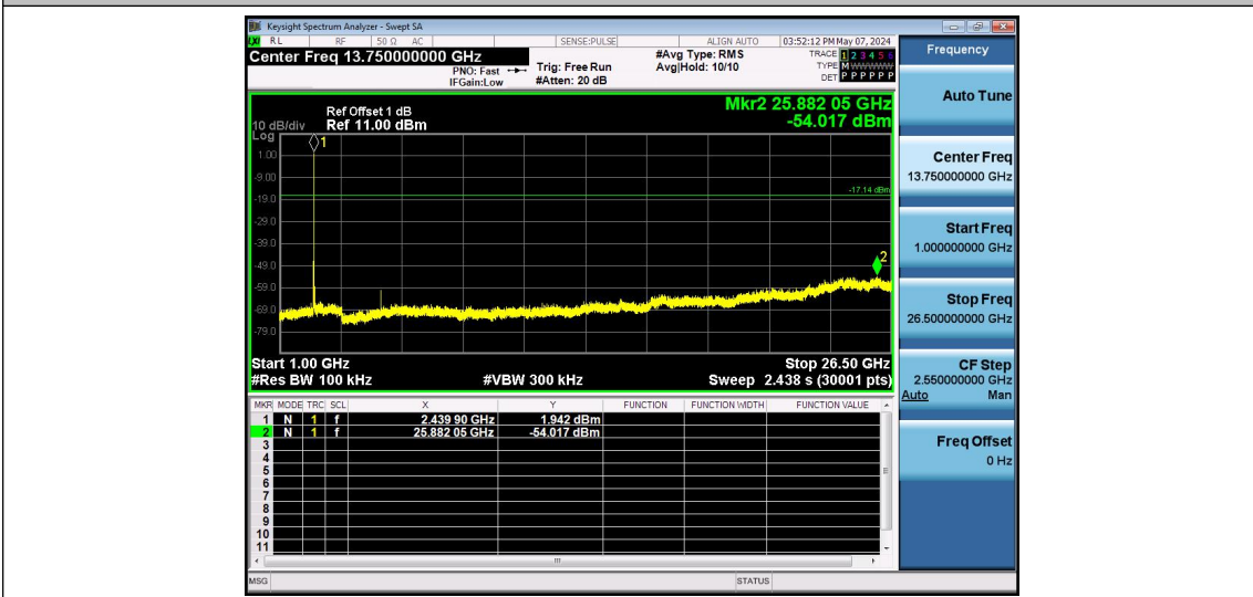
Zigbee-Ant1-2440-1000~26500-PASS
