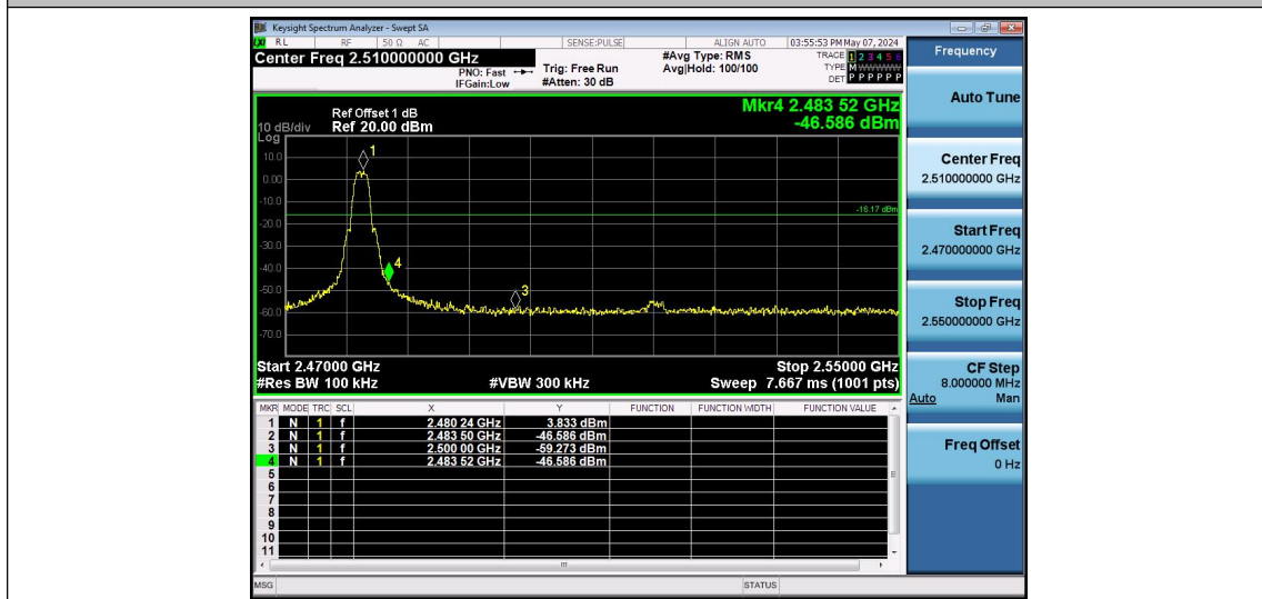
Zigbee-Ant1-2480-PASS
