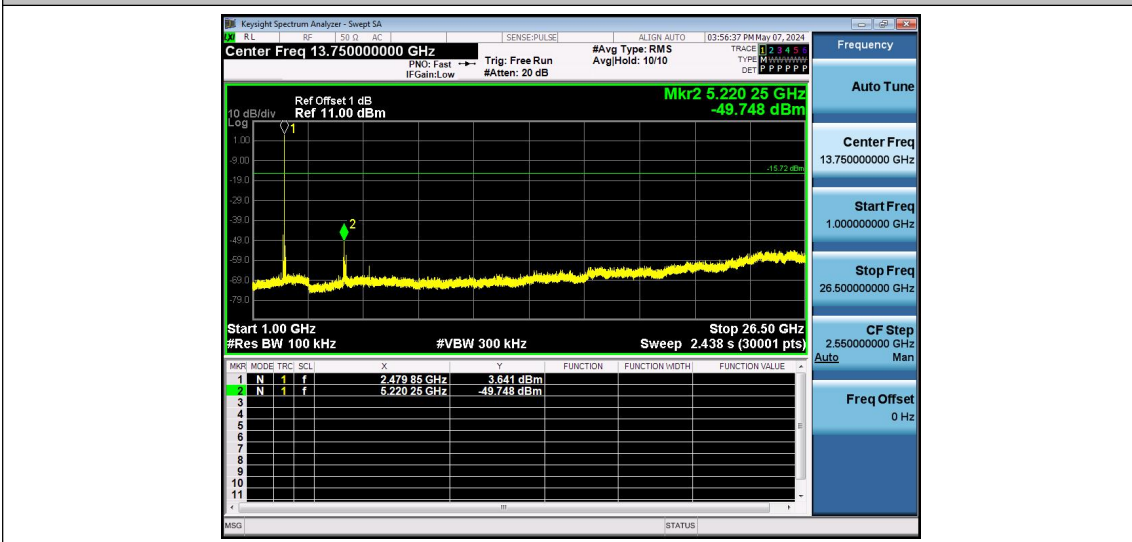
Zigbee-Ant1-2480-1000~26500-PASS
