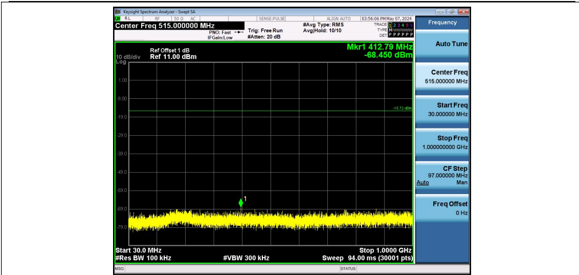
Zigbee-Ant1-2480-30~1000-PASS
