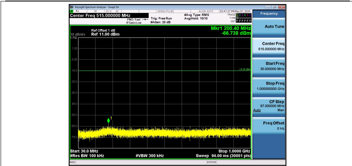
Zigbee-Ant1-2405-30~1000-PASS
