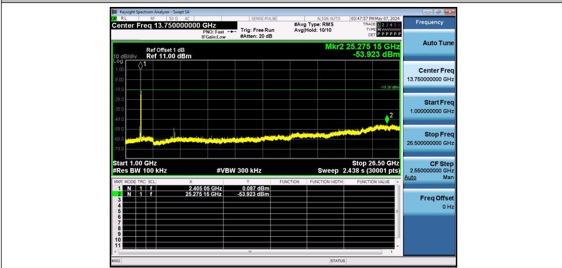
Zigbee-Ant1-2405-1000~26500-PASS
