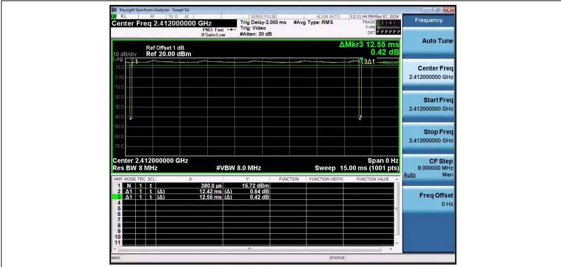
NTNV-11B-Ant1-2412
