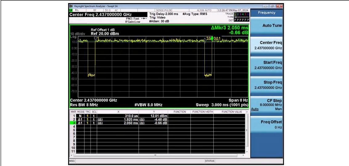
NTNV-11N20SISO-Ant1-2437
