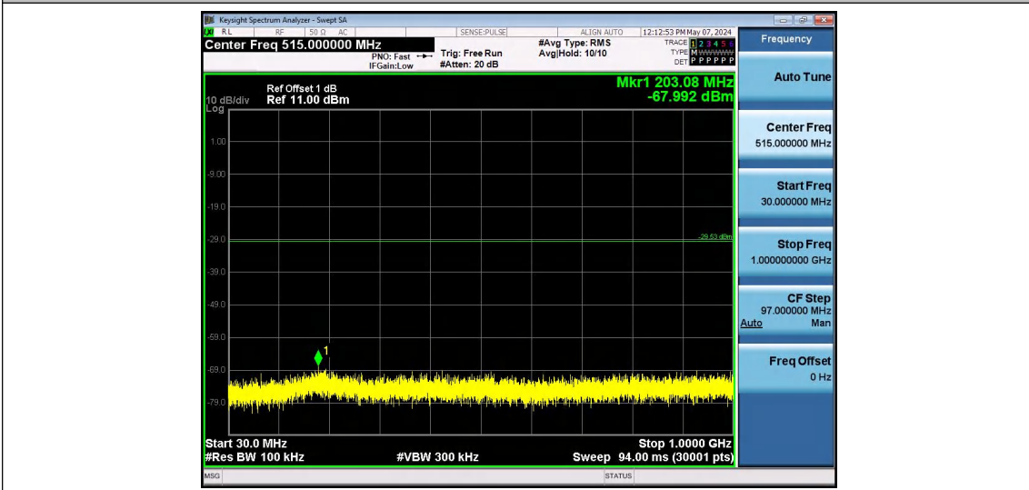
11B-Ant1-2412-30~1000-PASS
