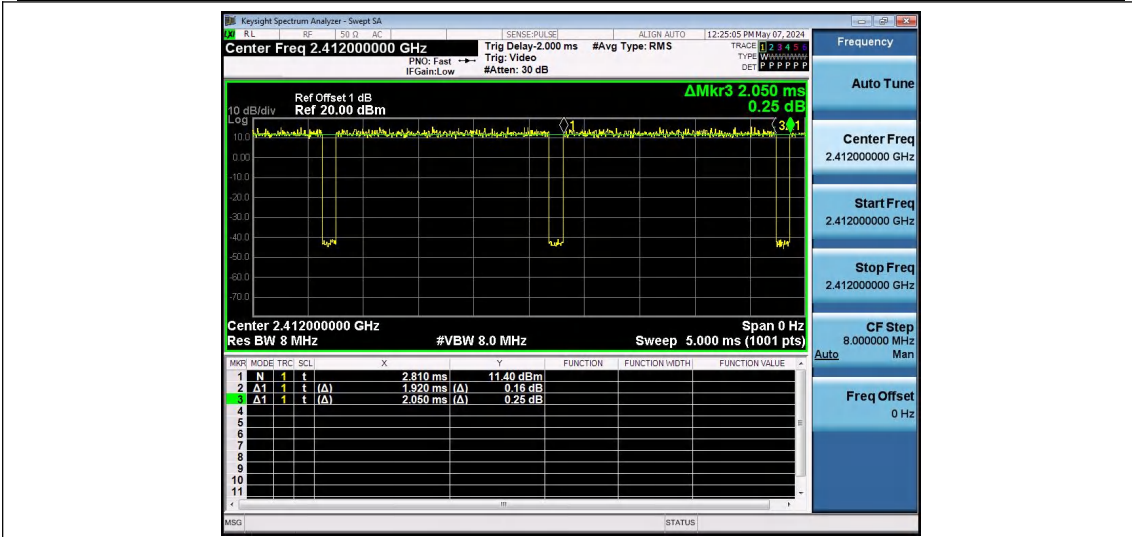
NTNV-11N20SISO-Ant1-2412
