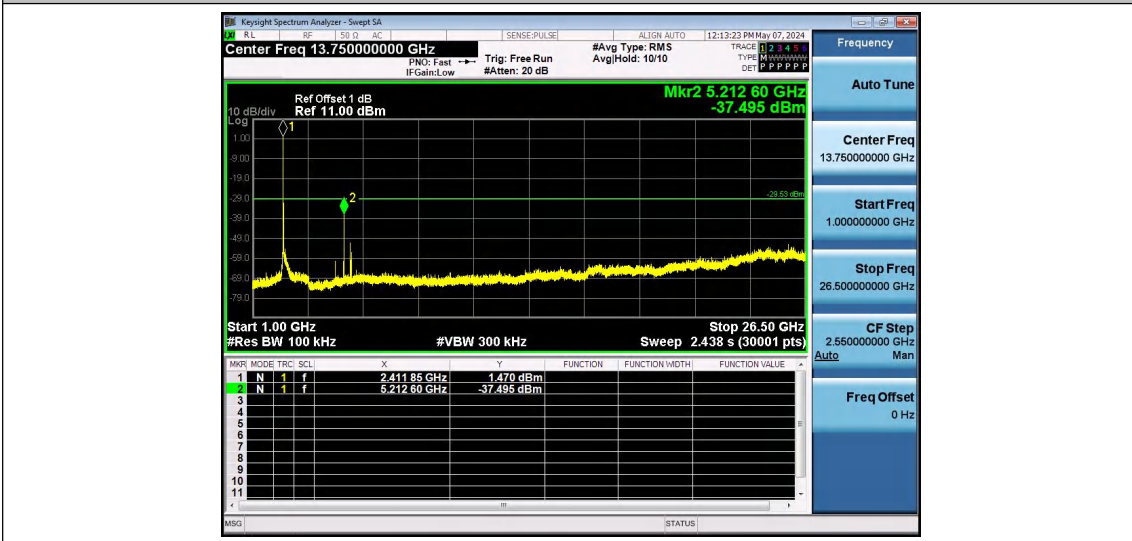
11B-Ant1-2412-1000~26500-PASS
