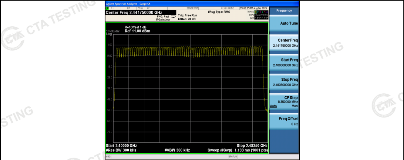
GFSK Modulation
