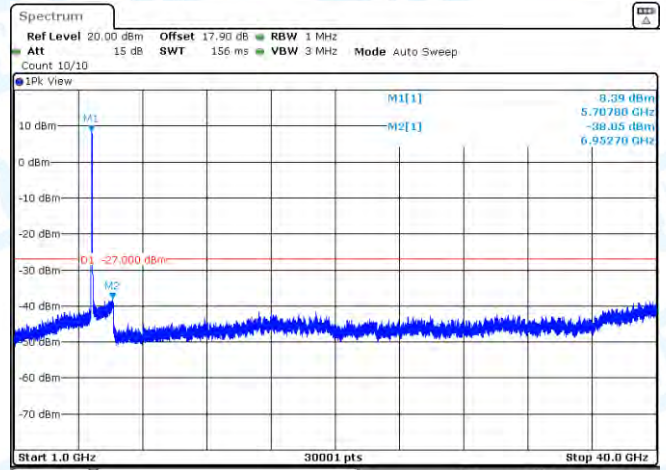
11N40MIMO-Ant1-5710-1000~40000-PASS
