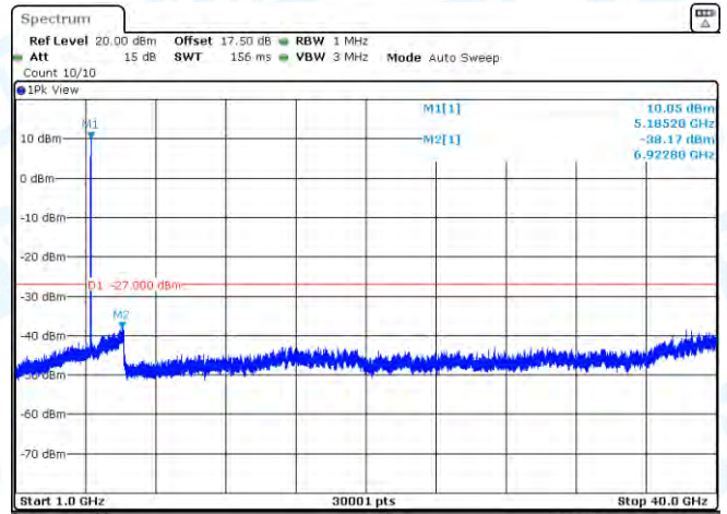
11AC20MIMO-Ant1-5180-1000~40000-PASS
