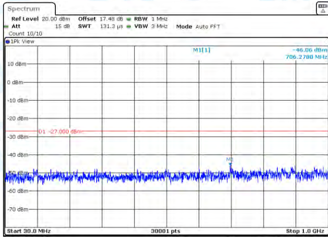
11AC40MIMO-Ant2-5190-30~1000-PASS
