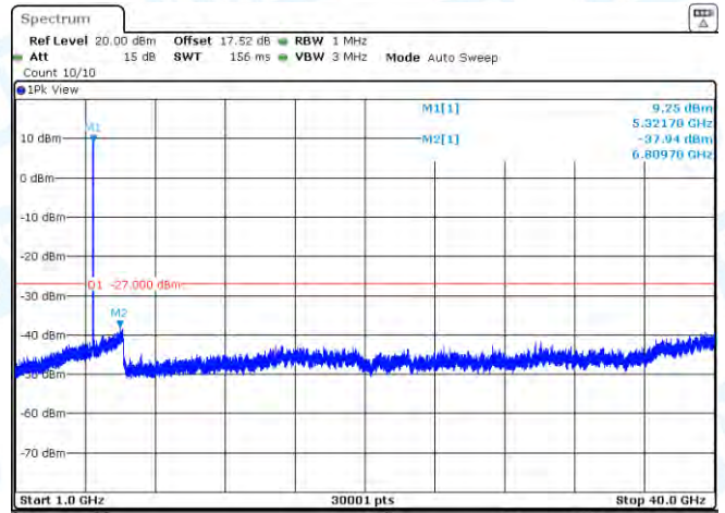
11N20MIMO-Ant1-5320-1000~40000-PASS
