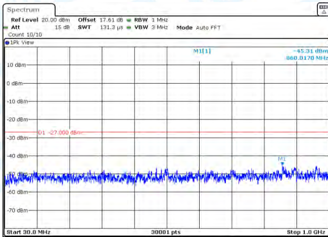
11AC40MIMO-Ant1-5510-30~1000-PASS
