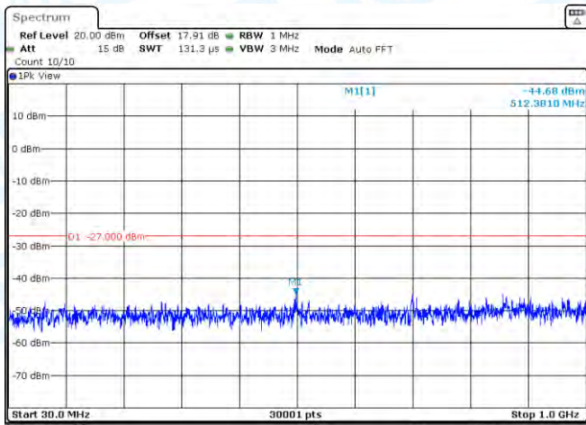
11AC20MIMO-Ant1-5700-30~1000-PASS
