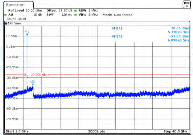
11AC20MIMO-Ant1-5720-1000~40000-PASS
