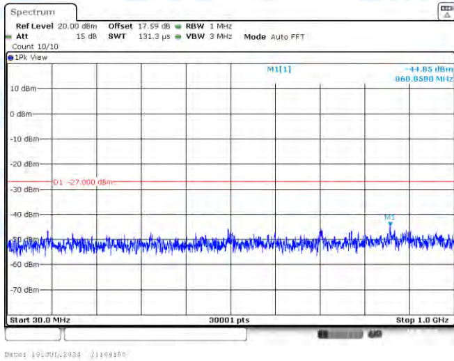
11N20MIMO-Ant1-5580-30~1000-PASS
