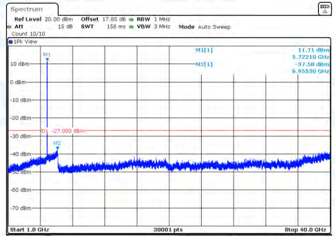
11N20MIMO-Ant2-5720-1000~40000-PASS
