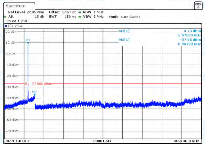
11N40MIMO-Ant1-5670-1000~40000-PASS
