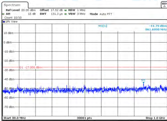
11AC40MIMO-Ant1-5270-30~1000-PASS
