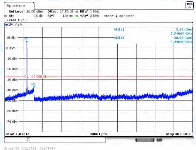
11AC80MIMO-Ant1-5530-1000~40000-PASS
