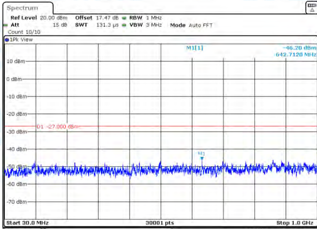
11AC20MIMO-Ant1-5260-30~1000-PASS
