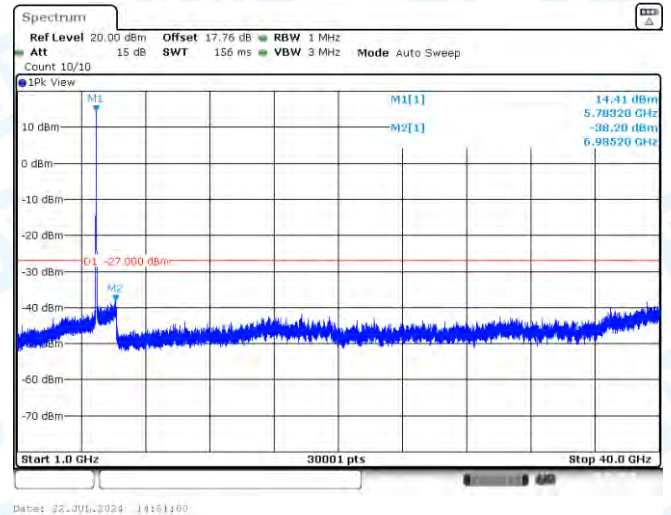
11N20MIMO-Ant2-5785-1000~40000-PASS
