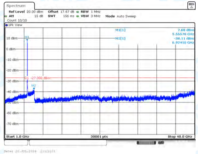
11AC40MIMO-Ant2-5550-1000~40000-PASS
