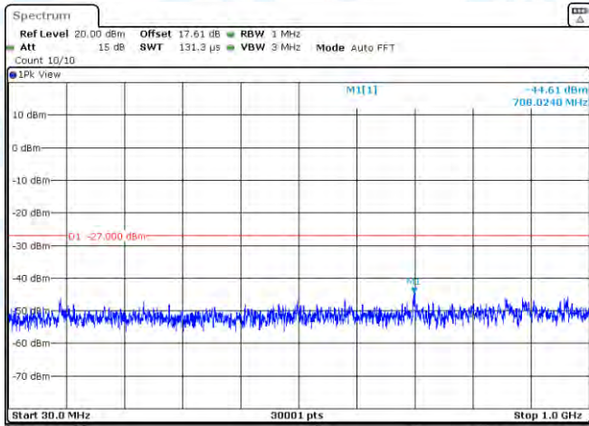
11N40MIMO-Ant1-5510-30~1000-PASS
