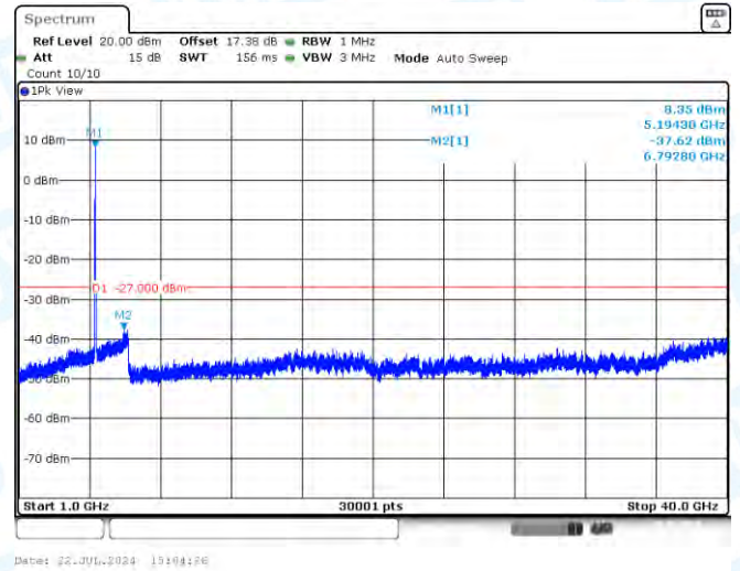
11N40MIMO-Ant1-5190-1000~40000-PASS
