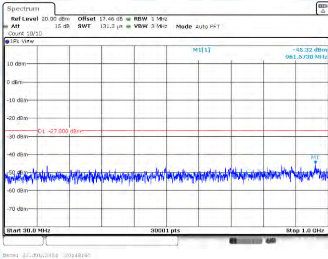
11AC80MIMO-Ant2-5210-30~1000-PASS
