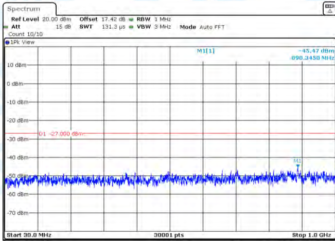
11AC20MIMO-Ant2-5260-30~1000-PASS
