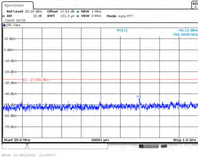
11AC80MIMO-Ant2-5290-30~1000-PASS
