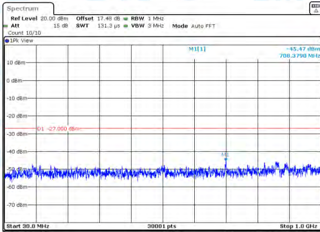
11AC20MIMO-Ant2-5200-30~1000-PASS
