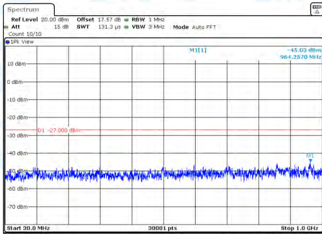
11N40MIMO-Ant1-5230-30~1000-PASS
