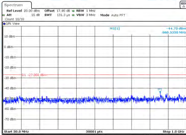
11AC40MIMO-Ant2-5670-30~1000-PASS
