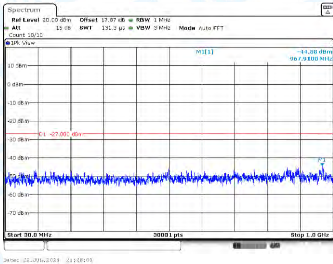
11AC40MIMO-Ant1-5670-30~1000-PASS
