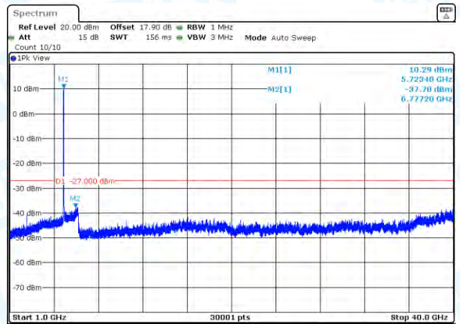
11N20MIMO-Ant2-5700-1000~40000-PASS
