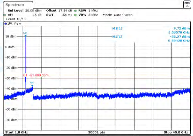
11N40MIMO-Ant1-5510-1000~40000-PASS
