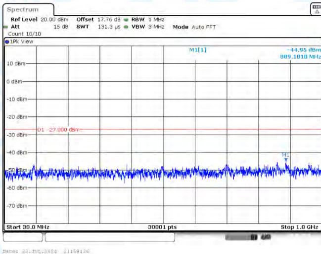
11AC80MIMO-Ant2-5610-30~1000-PASS
