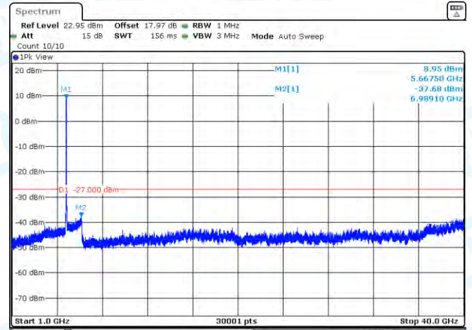
11AC40MIMO-Ant2-5670-1000~40000-PASS
