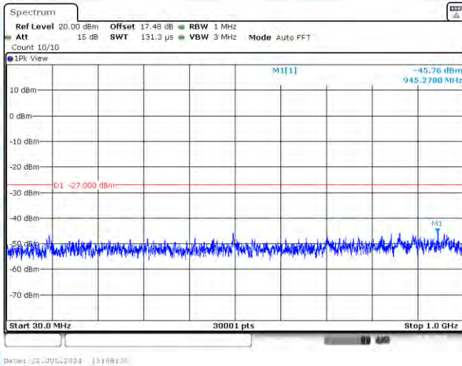
11N40MIMO-Ant2-5190-30~1000-PASS
