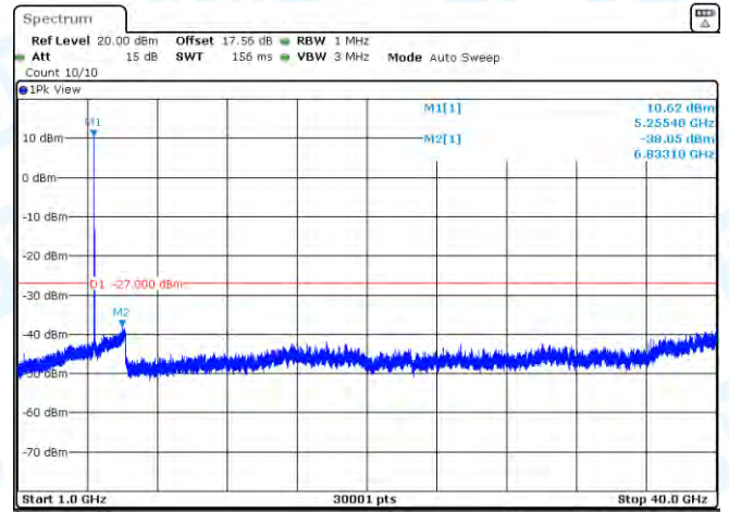
11AC20MIMO-Ant1-5260-1000~40000-PASS
