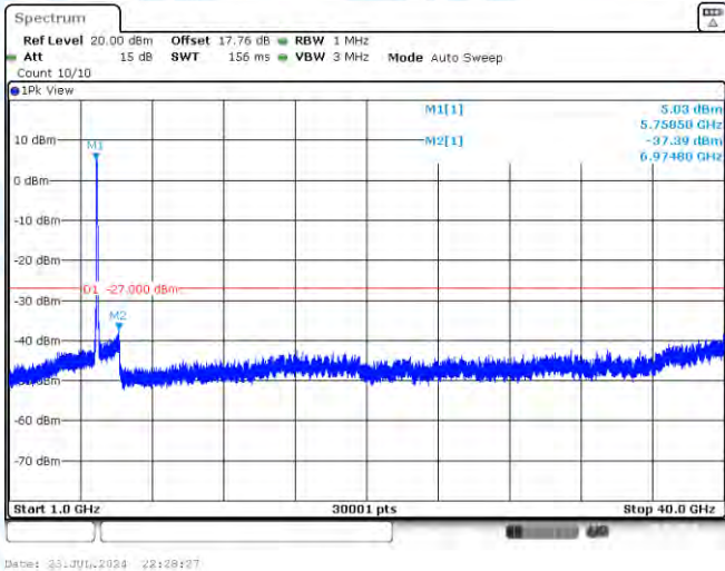
11AC80MIMO-Ant2-5775-1000~40000-PASS
