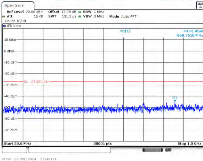
11AC80MIMO-Ant1-5610-30~1000-PASS
