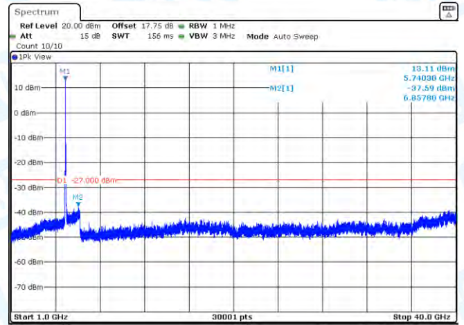
11AC20MIMO-Ant2-5720-1000~40000-PASS
