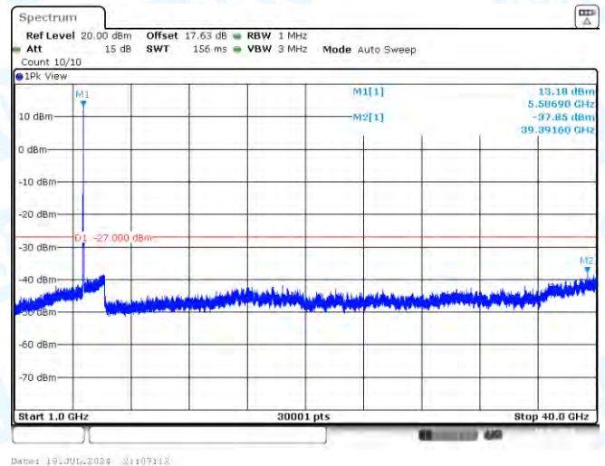
11N20MIMO-Ant2-5580-1000~40000-PASS
