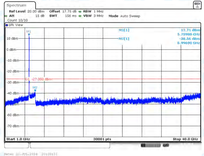
11AC40MIMO-Ant2-5755-1000~40000-PASS
