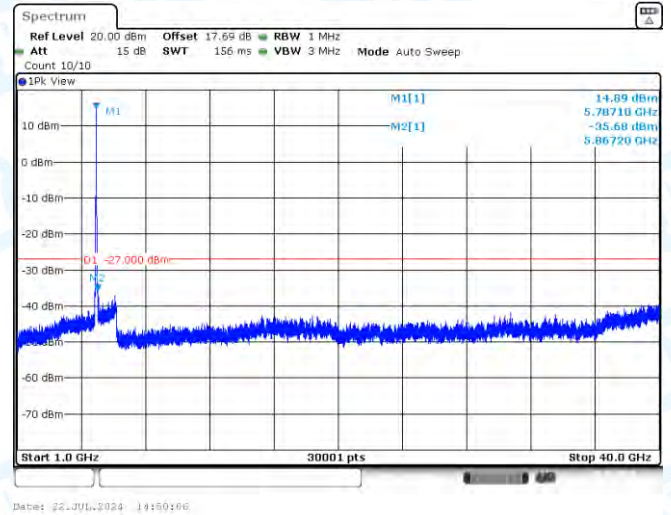
11N20MIMO-Ant1-5785-1000~40000-PASS
