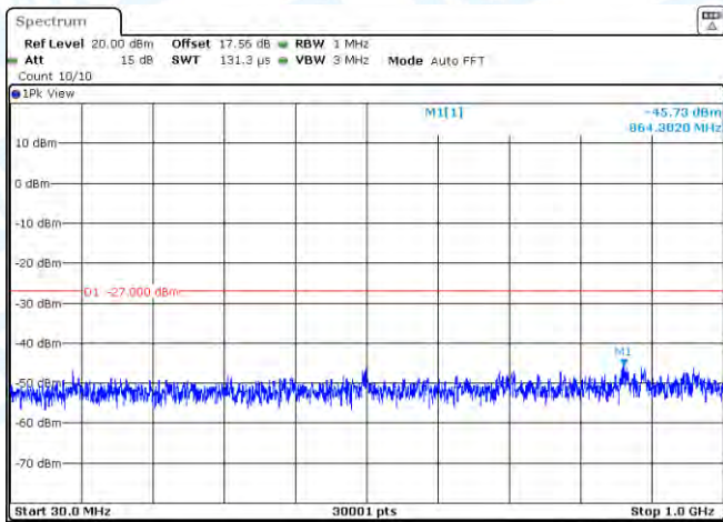
11N20MIMO-Ant2-5320-30~1000-PASS
