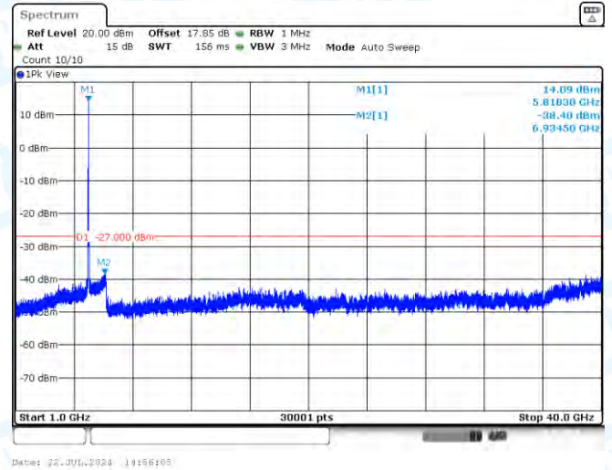
11N20MIMO-Ant2-5825-1000~40000-PASS
