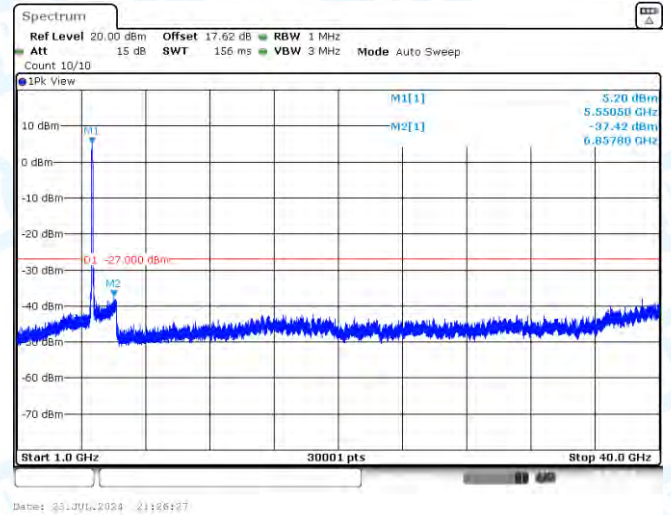
11AC80MIMO-Ant2-5530-1000~40000-PASS
