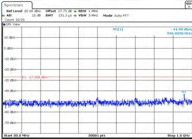
11N40MIMO-Ant2-5710-30~1000-PASS
