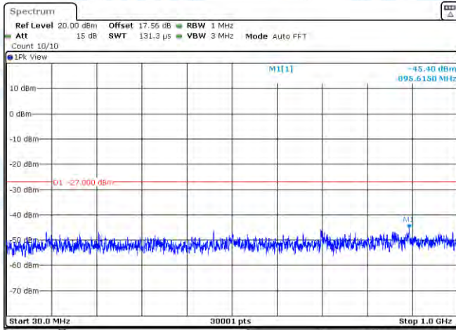
11AC20MIMO-Ant1-5500-30~1000-PASS
