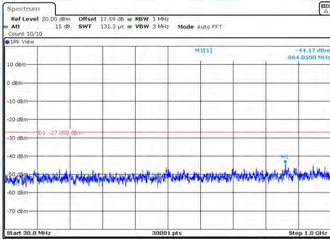
11AC20MIMO-Ant2-5500-30~1000-PASS
