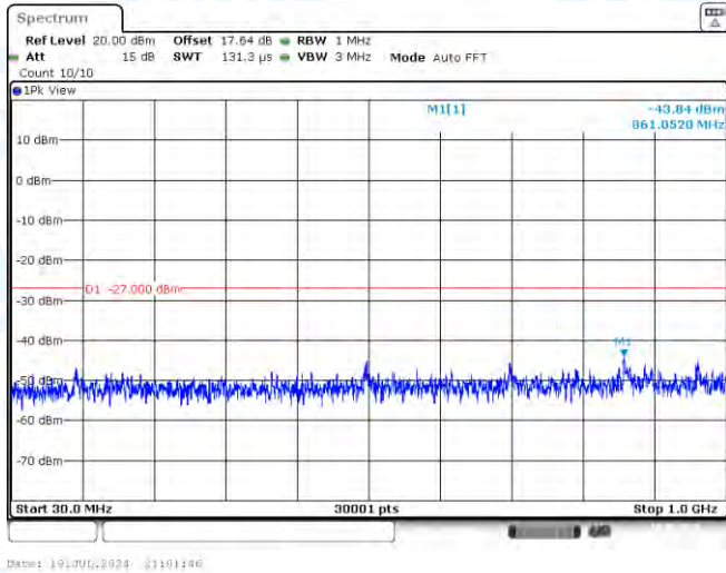
11N20MIMO-Ant2-5500-30~1000-PASS
