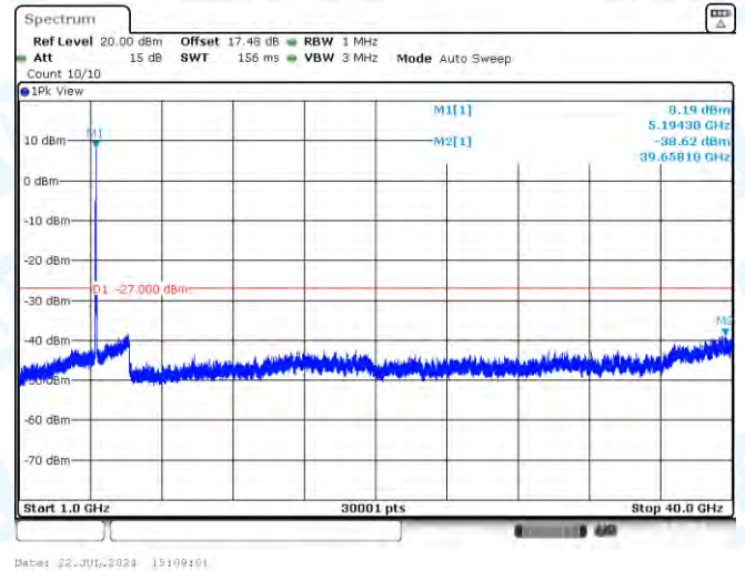
11N40MIMO-Ant2-5190-1000~40000-PASS
