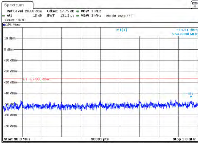
11N40MIMO-Ant2-5755-30~1000-PASS
