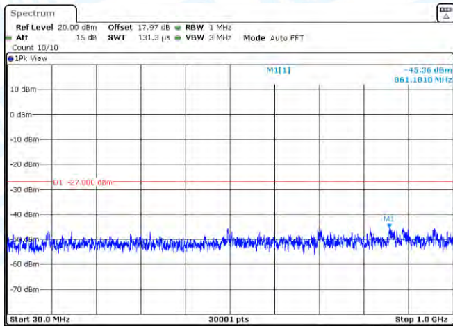
11N40MIMO-Ant1-5670-30~1000-PASS
