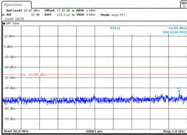
11AC20MIMO-Ant1-5180-30~1000-PASS
