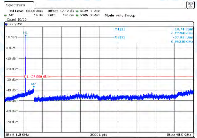
11AC20MIMO-Ant2-5260-1000~40000-PASS
