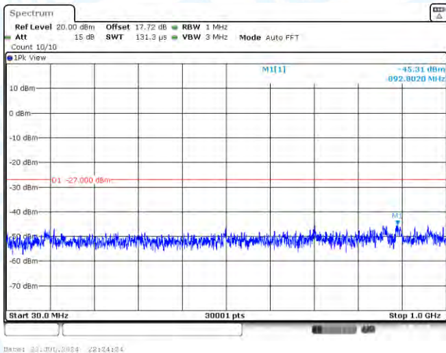
11AC80MIMO-Ant1-5775-30~1000-PASS
