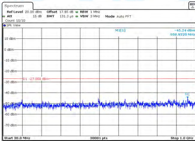
11AC40MIMO-Ant1-5710-30~1000-PASS
