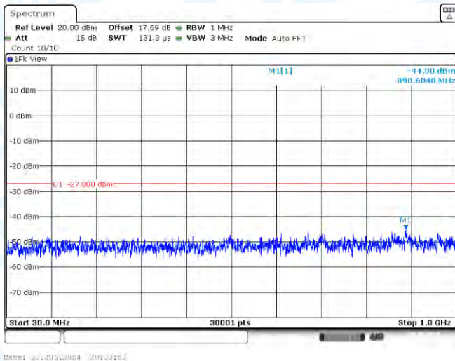
11AC40MIMO-Ant1-5795-30~1000-PASS
