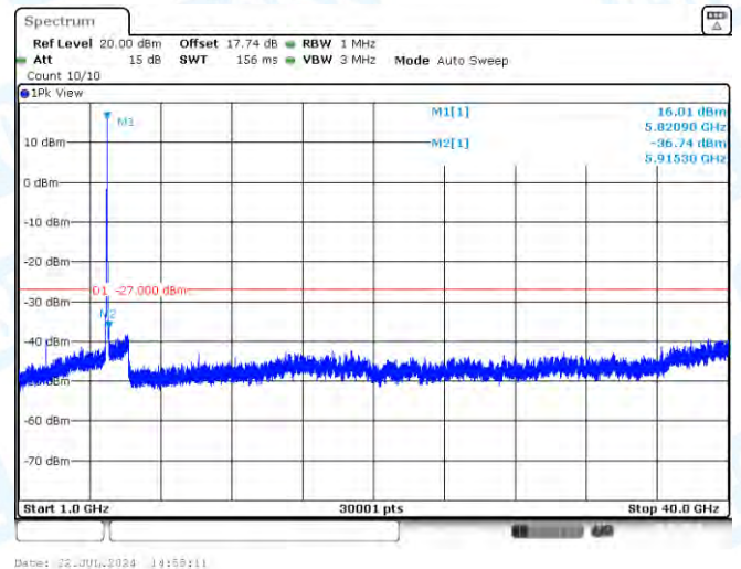
11N20MIMO-Ant1-5825-1000~40000-PASS
