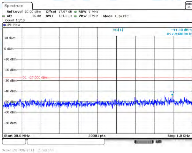
11AC40MIMO-Ant2-5550-30~1000-PASS
