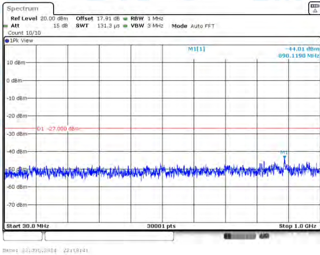
11AC80MIMO-Ant2-5690-30~1000-PASS
