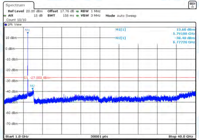
11AC20MIMO-Ant1-5785-1000~40000-PASS
