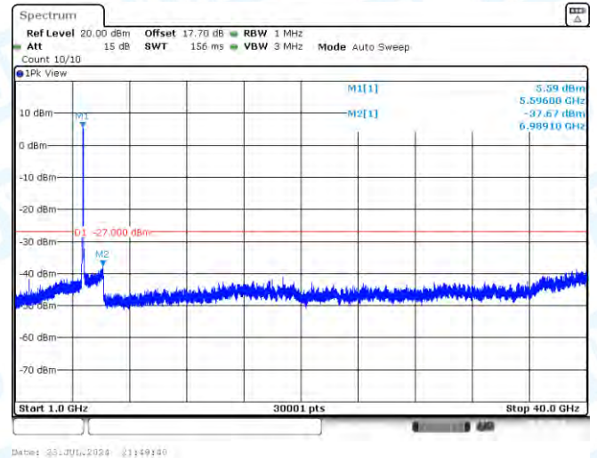
11AC80MIMO-Ant1-5610-1000~40000-PASS
