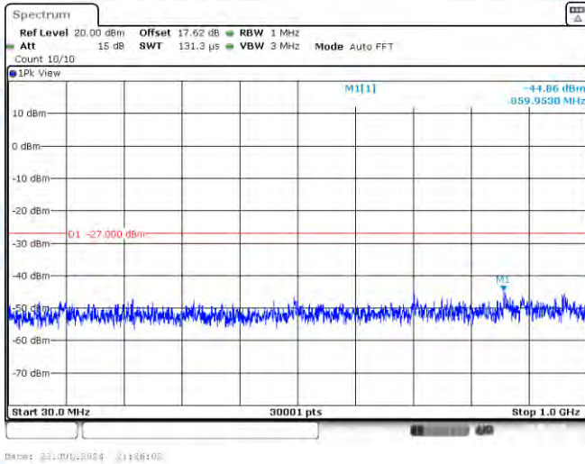
11AC80MIMO-Ant2-5530-30~1000-PASS
