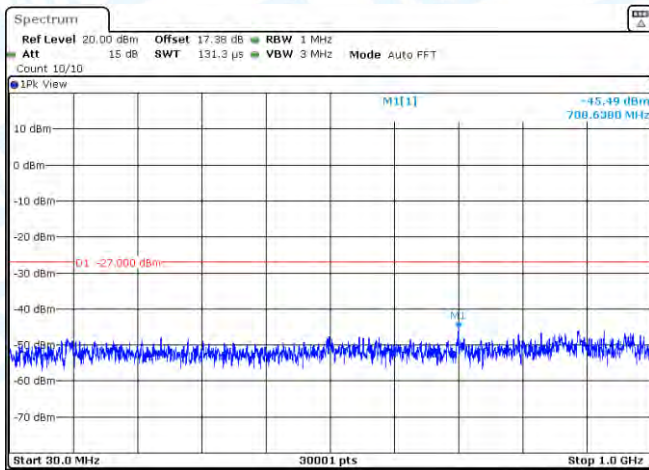
11AC20MIMO-Ant2-5825-30~1000-PASS
