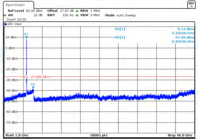
11N40MIMO-Ant2-5550-1000~40000-PASS
