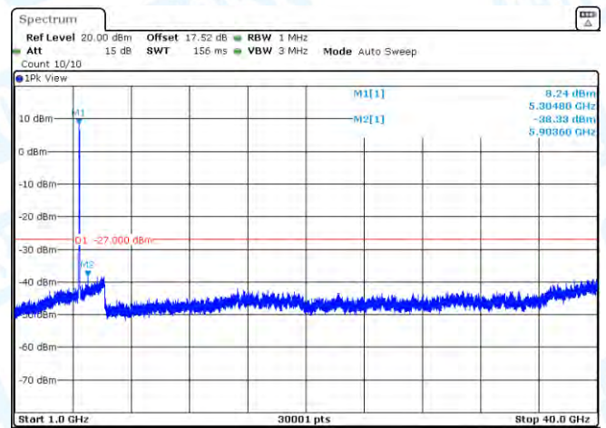
11N40MIMO-Ant1-5310-1000~40000-PASS
