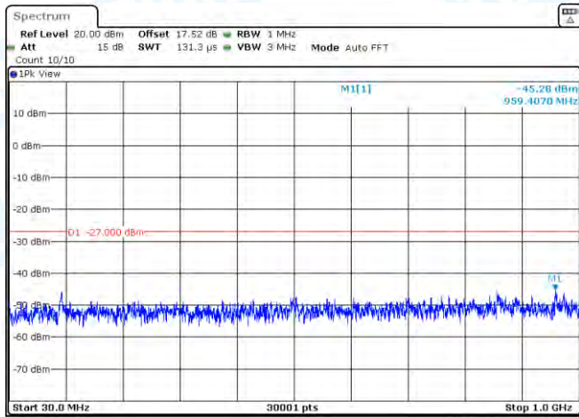
11AC20MIMO-Ant2-5280-30~1000-PASS
