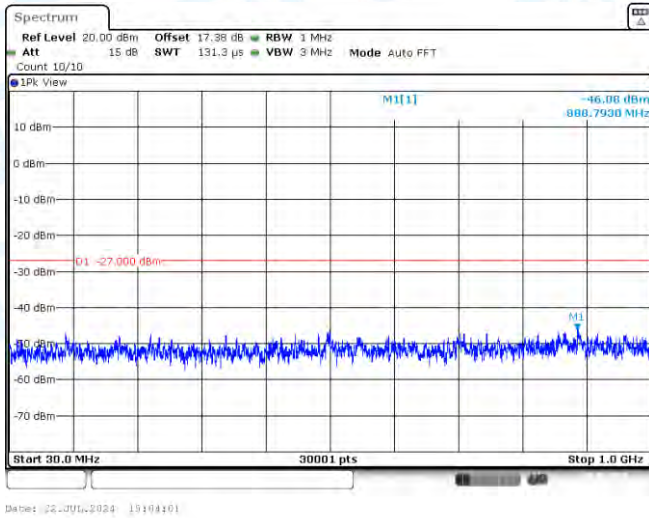
11N40MIMO-Ant1-5190-30~1000-PASS
