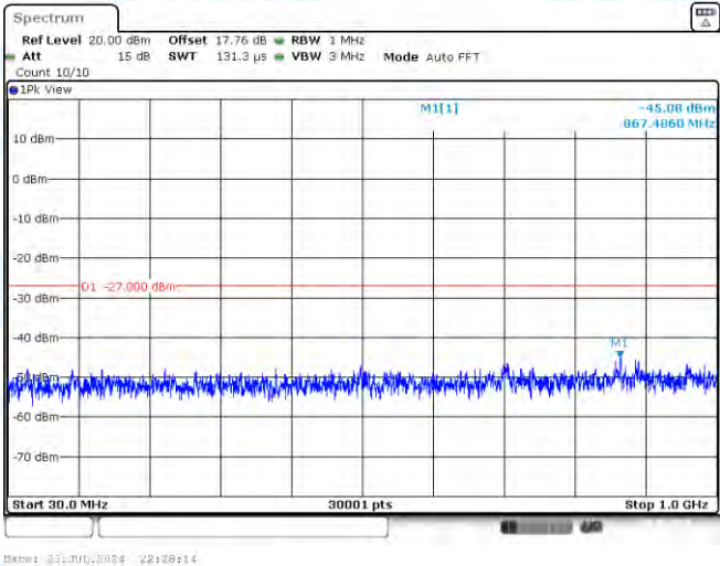
11AC80MIMO-Ant2-5775-30~1000-PASS
