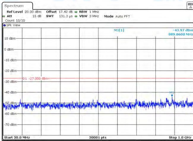
11N20MIMO-Ant2-5260-30~1000-PASS
