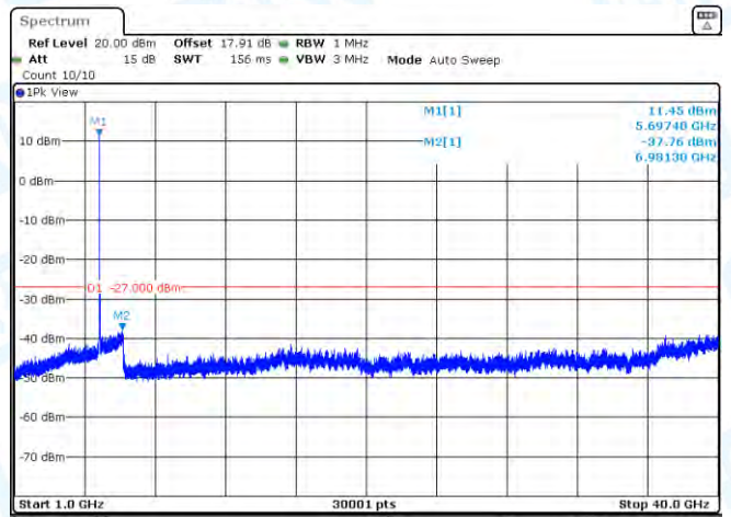
11AC20MIMO-Ant1-5700-1000~40000-PASS
