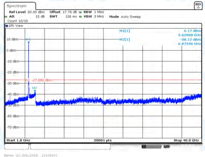
11AC80MIMO-Ant2-5610-1000~40000-PASS
