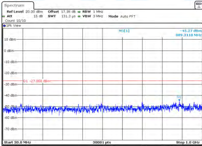
11AC20MIMO-Ant2-5180-30~1000-PASS
