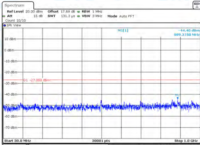
11AC20MIMO-Ant2-5745-30~1000-PASS
