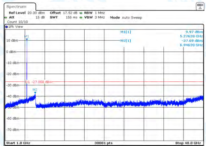
11N20MIMO-Ant1-5280-1000~40000-PASS
