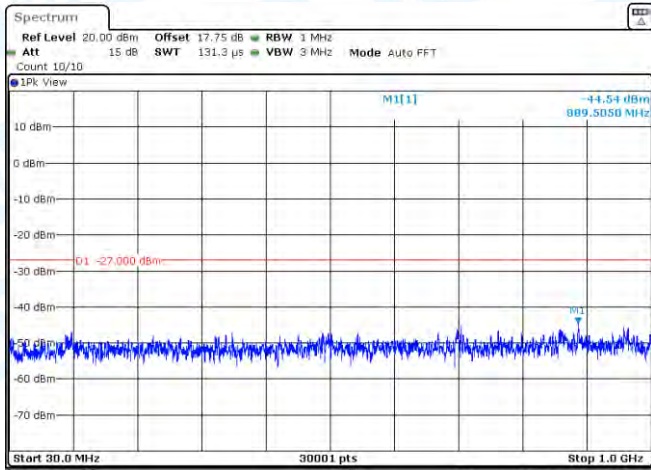
11AC20MIMO-Ant2-5720-30~1000-PASS
