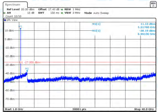
11AC20MIMO-Ant2-5280-1000~40000-PASS
