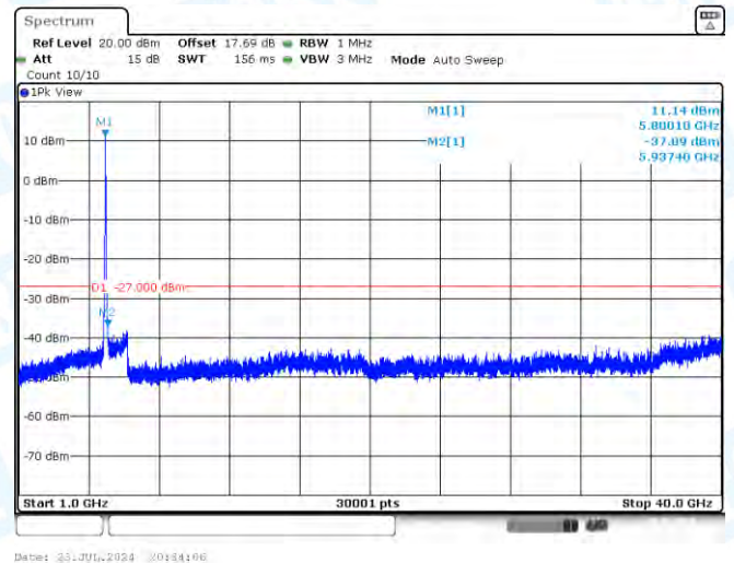
11AC40MIMO-Ant1-5795-1000~40000-PASS
