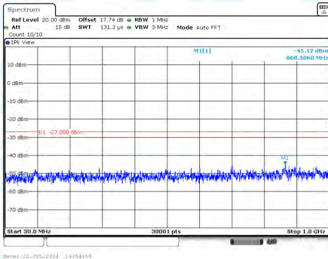
11N20MIMO-Ant1-5825-30~1000-PASS
