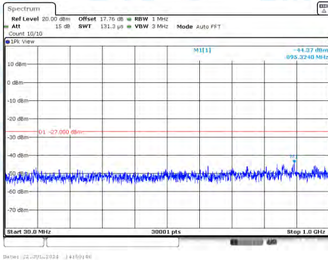
11N20MIMO-Ant2-5785-30~1000-PASS
