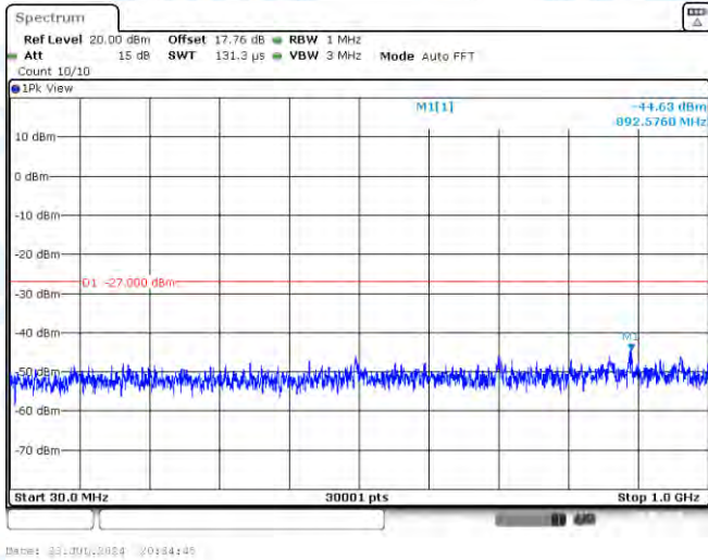
11AC40MIMO-Ant2-5795-30~1000-PASS
