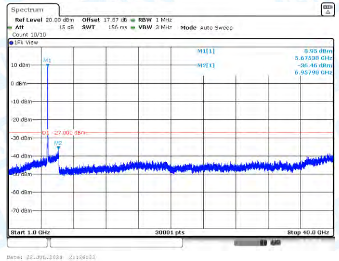
11AC40MIMO-Ant1-5670-1000~40000-PASS
