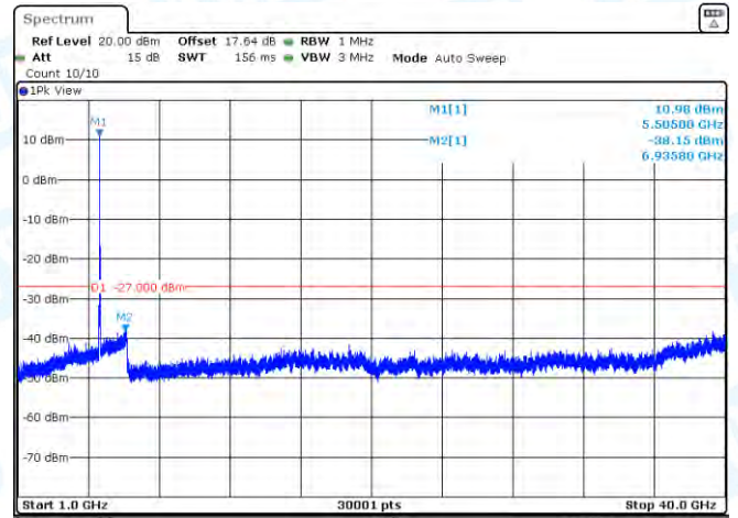
11AC20MIMO-Ant1-5500-1000~40000-PASS
