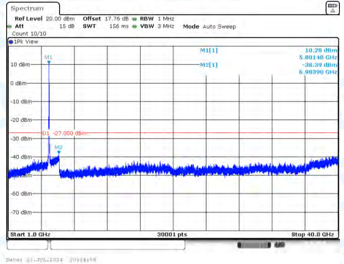
11AC40MIMO-Ant2-5795-1000~40000-PASS
