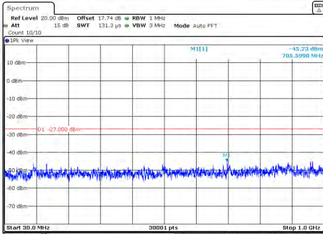
11AC20MIMO-Ant1-5825-30~1000-PASS
