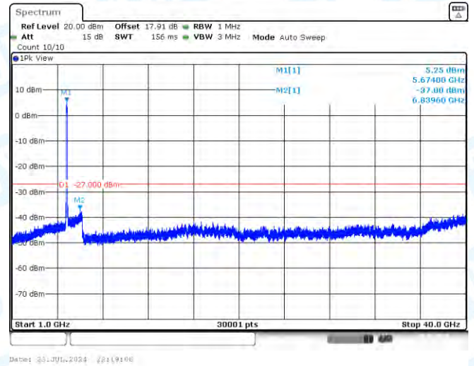
11AC80MIMO-Ant2-5690-1000~40000-PASS
