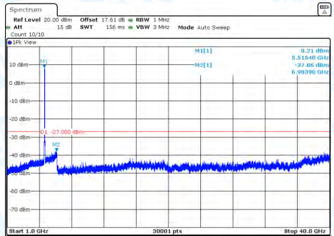
11AC40MIMO-Ant1-5510-1000~40000-PASS
