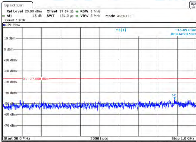
11AC40MIMO-Ant2-5310-30~1000-PASS
