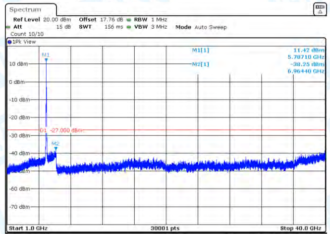
11N40MIMO-Ant1-5795-1000~40000-PASS
