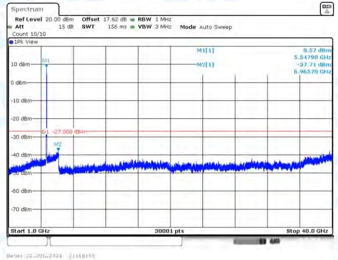
11AC40MIMO-Ant1-5550-1000~40000-PASS
