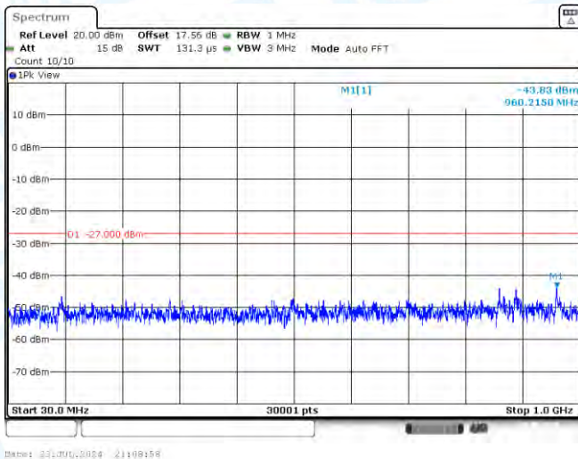
11AC80MIMO-Ant1-5530-30~1000-PASS
