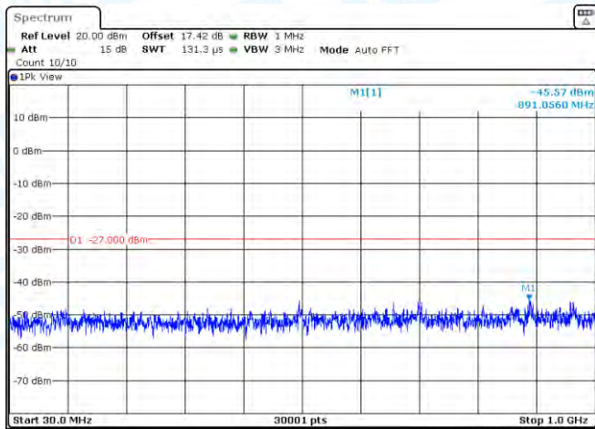
11N40MIMO-Ant2-5230-30~1000-PASS
