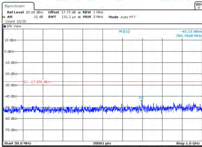
11N20MIMO-Ant2-5720-30~1000-PASS
