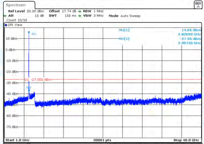
11AC20MIMO-Ant1-5825-1000~40000-PASS
