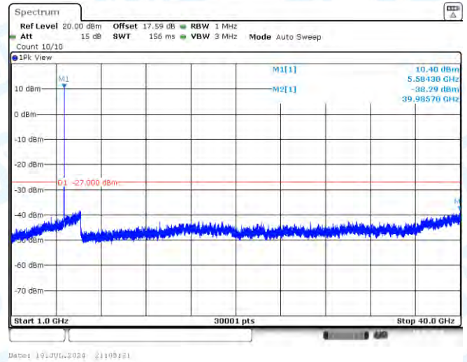
11N20MIMO-Ant1-5580-1000~40000-PASS
