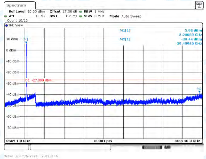
11AC80MIMO-Ant1-5210-1000~40000-PASS
