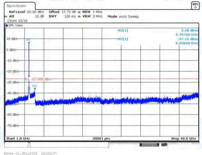
11AC80MIMO-Ant1-5775-1000~40000-PASS
