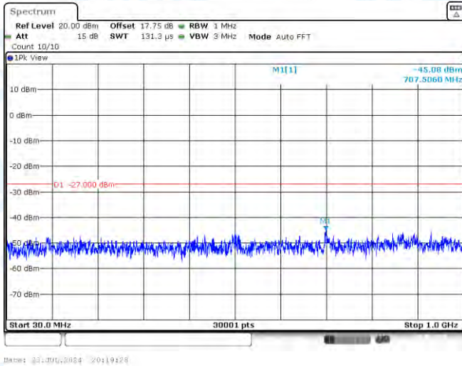
11AC40MIMO-Ant1-5755-30~1000-PASS
