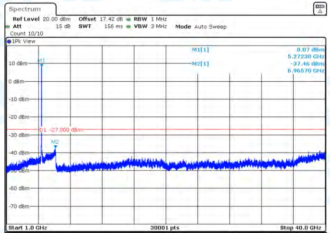
11AC40MIMO-Ant1-5270-1000~40000-PASS
