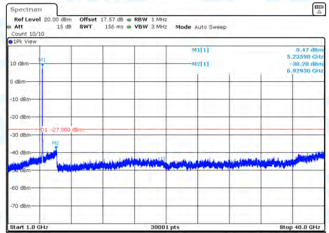
11N40MIMO-Ant1-5230-1000~40000-PASS
