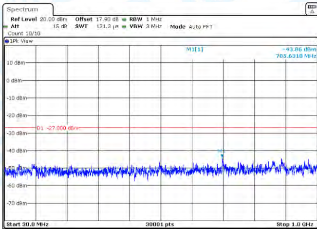
11N20MIMO-Ant2-5700-30~1000-PASS
