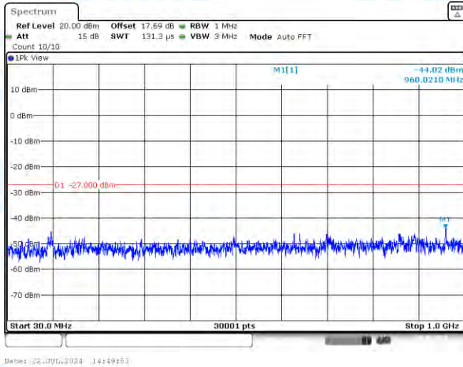
11N20MIMO-Ant1-5785-30~1000-PASS
