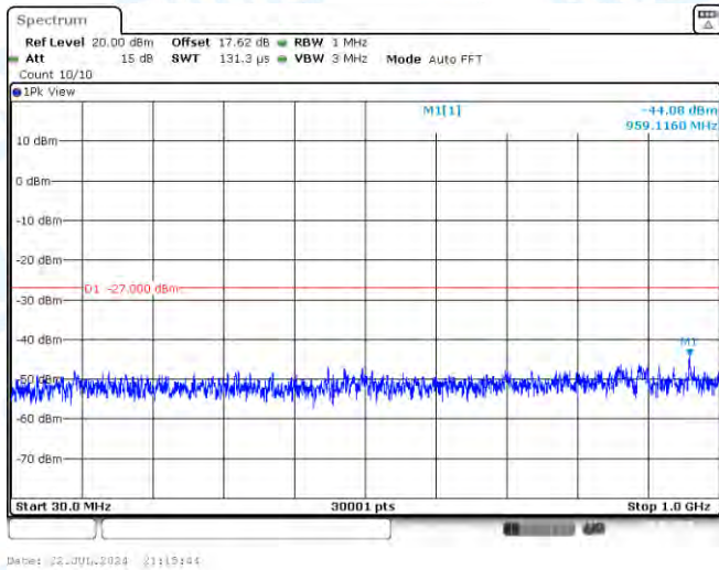
11AC40MIMO-Ant1-5550-30~1000-PASS
