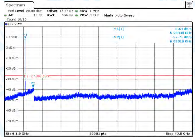
11AC40MIMO-Ant1-5230-1000~40000-PASS
