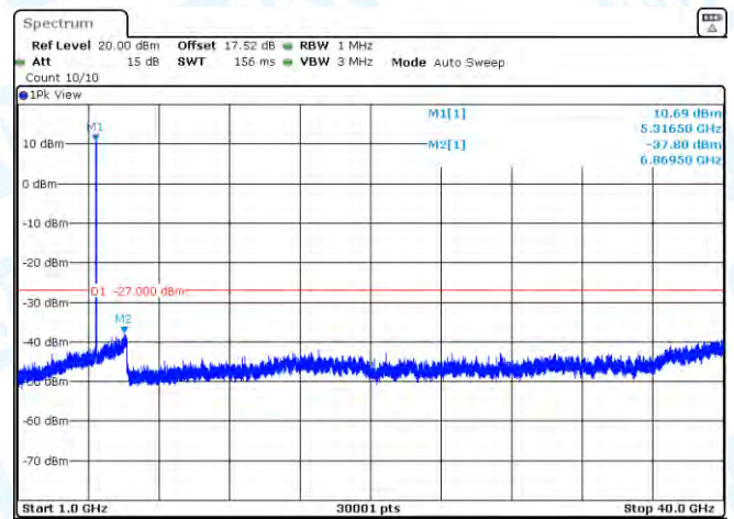
11AC20MIMO-Ant1-5320-1000~40000-PASS
