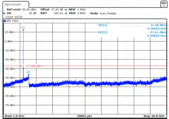
11N20MIMO-Ant1-5700-1000~40000-PASS
