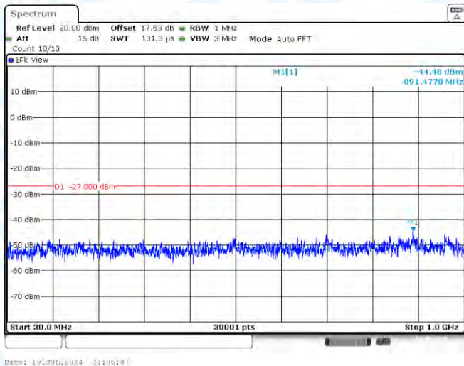
11N20MIMO-Ant2-5580-30~1000-PASS
