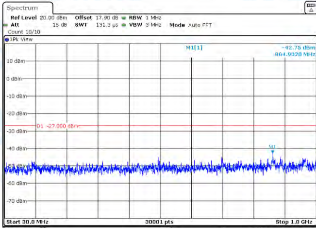
11N20MIMO-Ant1-5700-30~1000-PASS
