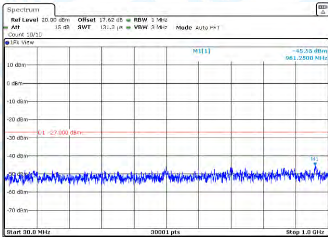
11N40MIMO-Ant2-5510-30~1000-PASS
