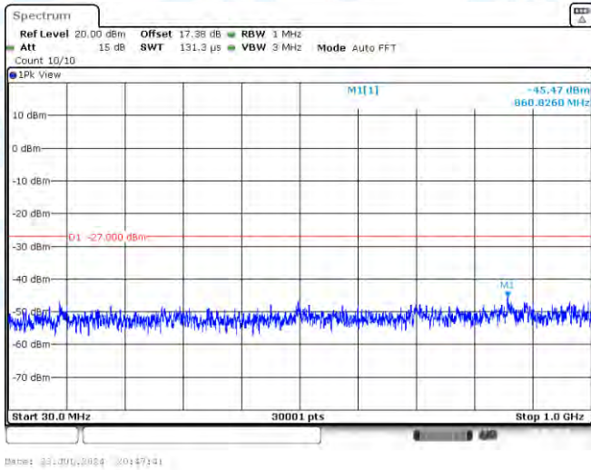
11AC80MIMO-Ant1-5210-30~1000-PASS
