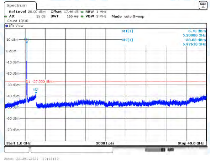
11AC80MIMO-Ant2-5210-1000~40000-PASS
