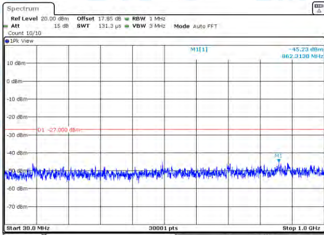
11N40MIMO-Ant1-5710-30~1000-PASS
