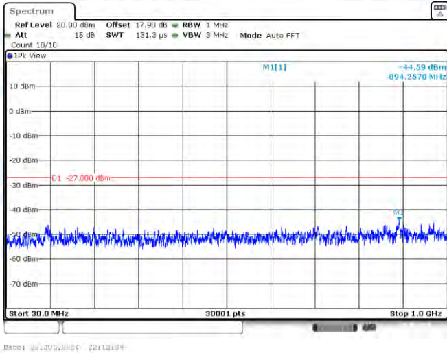
11AC80MIMO-Ant1-5690-30~1000-PASS
