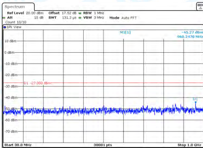
11N40MIMO-Ant1-5310-30~1000-PASS
