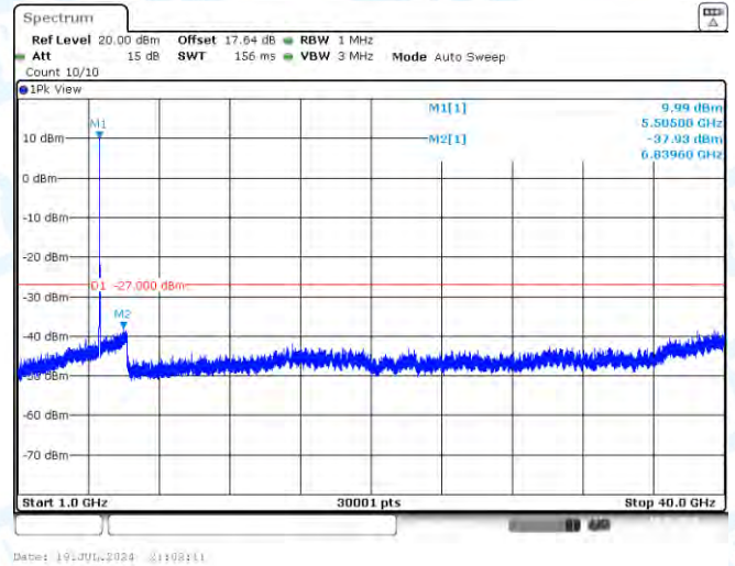
11N20MIMO-Ant2-5500-1000~40000-PASS
