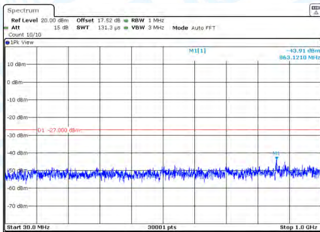
11N20MIMO-Ant1-5280-30~1000-PASS
