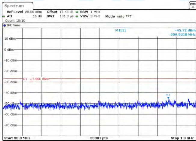
11AC40MIMO-Ant2-5270-30~1000-PASS
