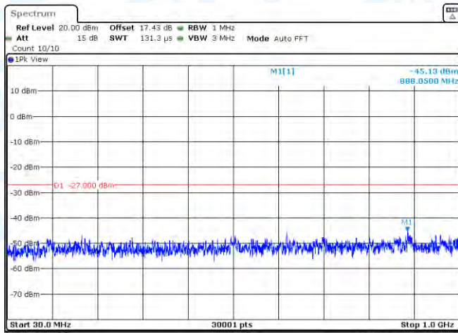
11N40MIMO-Ant2-5270-30~1000-PASS
