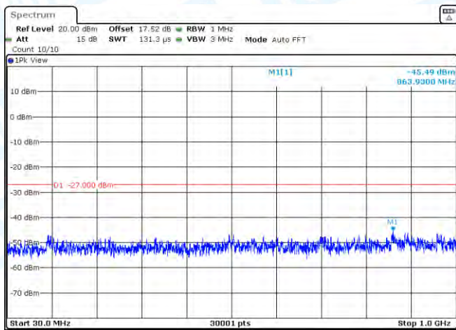
11AC20MIMO-Ant1-5320-30~1000-PASS
