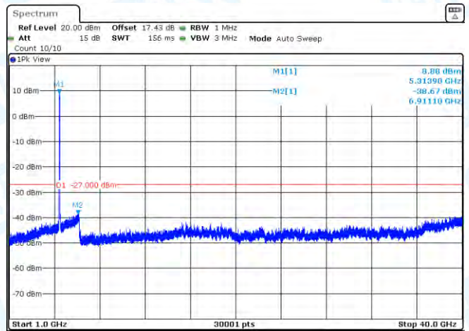
11AC40MIMO-Ant2-5270-1000~40000-PASS
