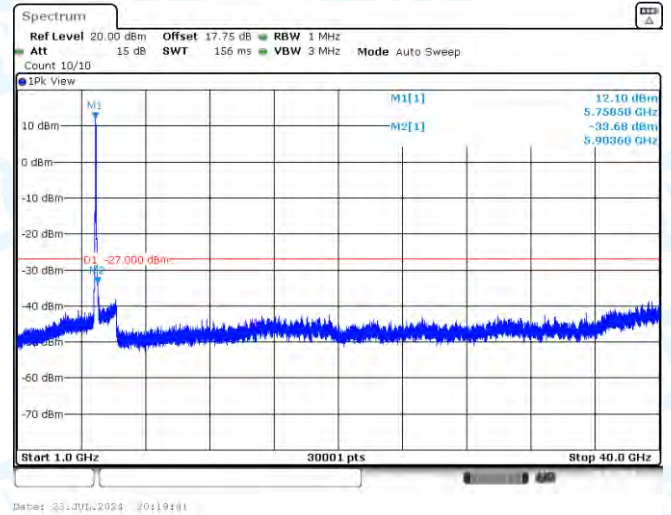
11AC40MIMO-Ant1-5755-1000~40000-PASS
