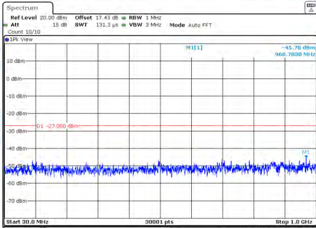
11N20MIMO-Ant1-5320-30~1000-PASS
