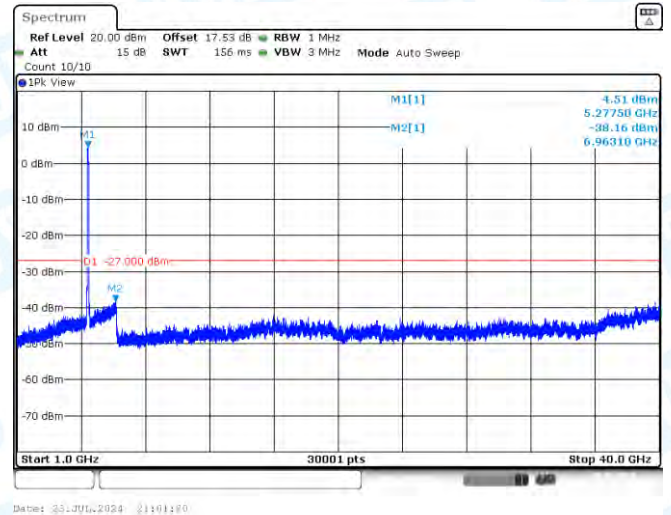
11AC80MIMO-Ant2-5290-1000~40000-PASS
