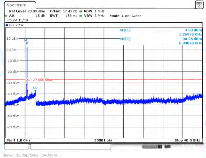
11AC80MIMO-Ant1-5290-1000~40000-PASS
