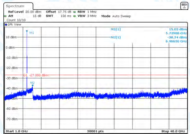
11N20MIMO-Ant1-5745-1000~40000-PASS
