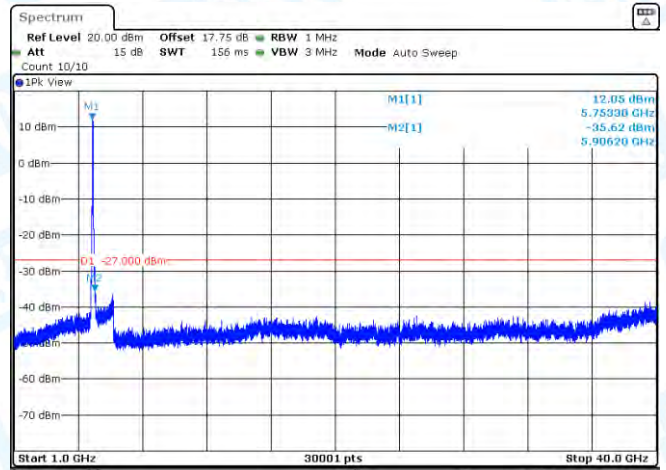
11N40MIMO-Ant2-5710-1000~40000-PASS
