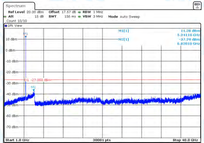
11AC20MIMO-Ant1-5240-1000~40000-PASS
