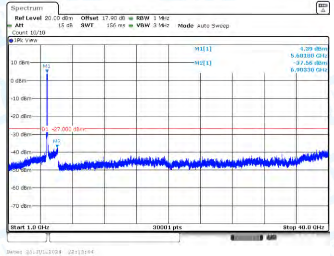
11AC80MIMO-Ant1-5690-1000~40000-PASS
