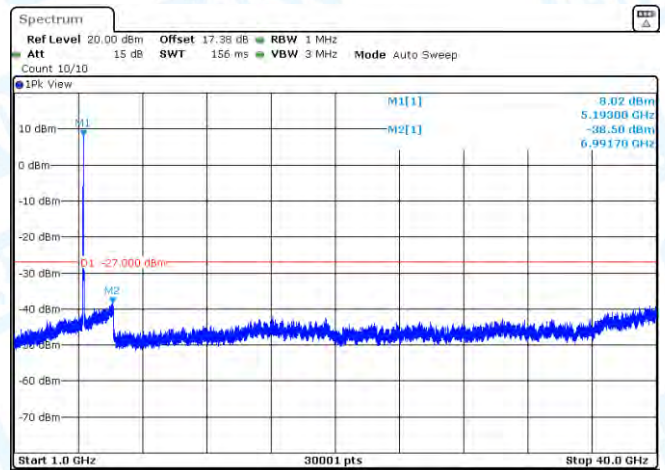
11AC20MIMO-Ant2-5825-1000~40000-PASS
