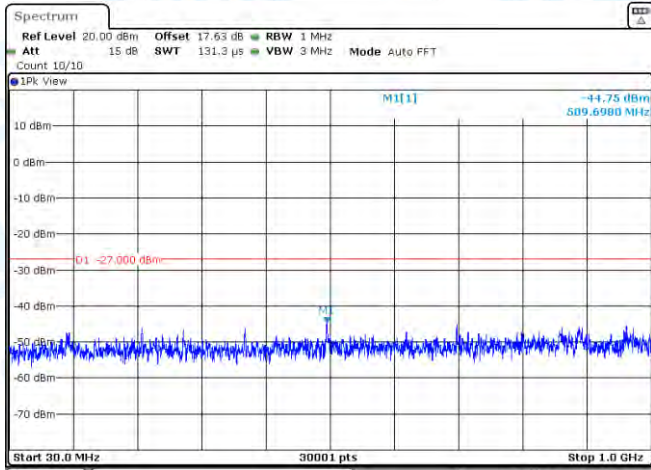
11AC20MIMO-Ant2-5580-30~1000-PASS
