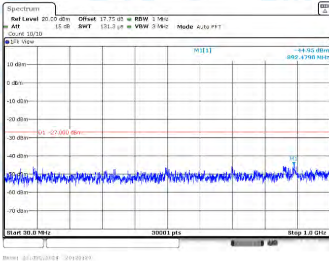
11AC40MIMO-Ant2-5755-30~1000-PASS
