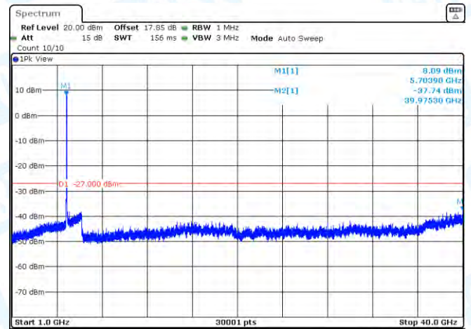
11AC40MIMO-Ant1-5710-1000~40000-PASS
