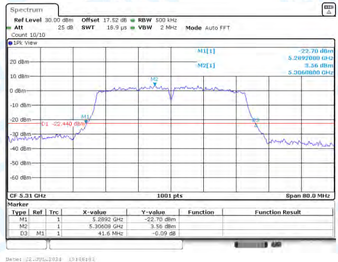
11N40MIMO-Ant2-5310
