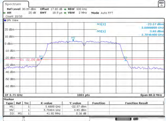
11N40MIMO-Ant2-5710
