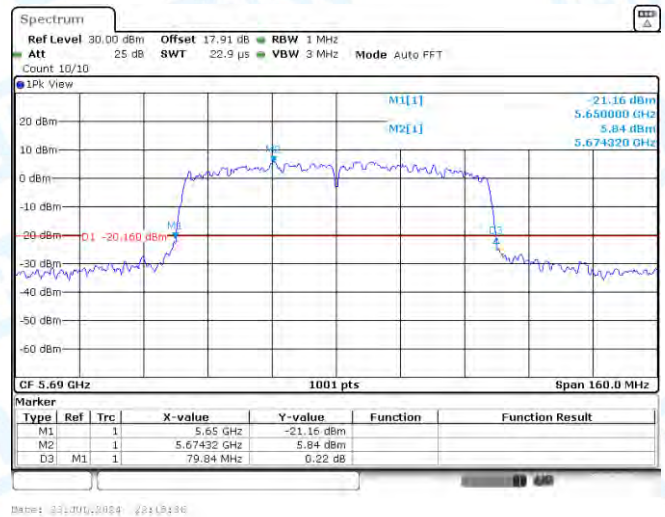
11AC80MIMO-Ant2-5690
