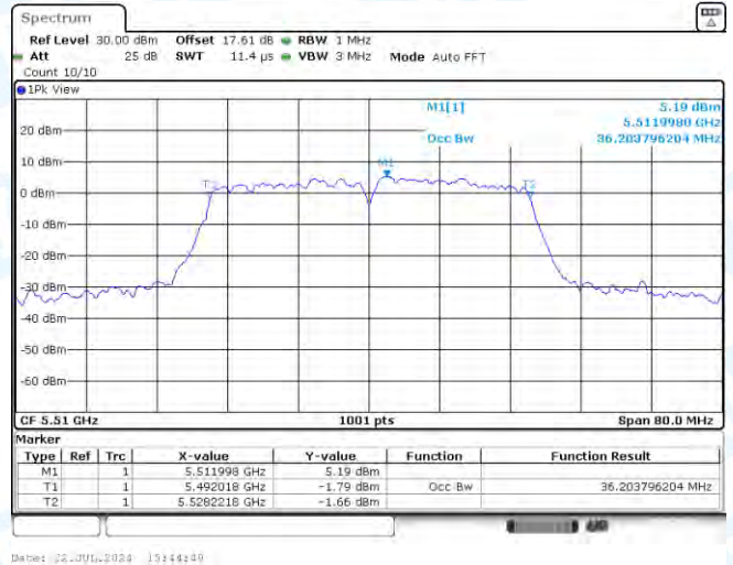
11N40MIMO-Ant2-5510
