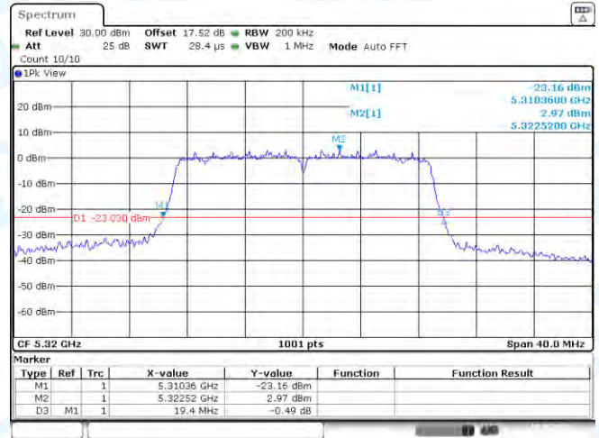
11N20MIMO-Ant2-5320
