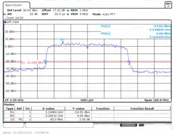
11AC80MIMO-Ant2-5290
