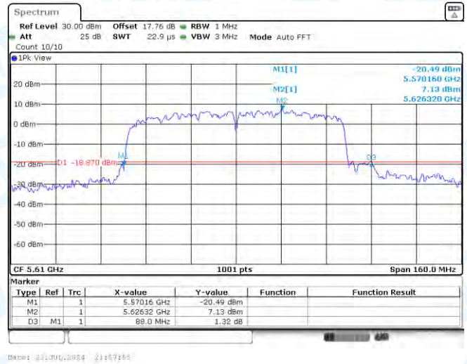
11AC80MIMO-Ant2-5610
