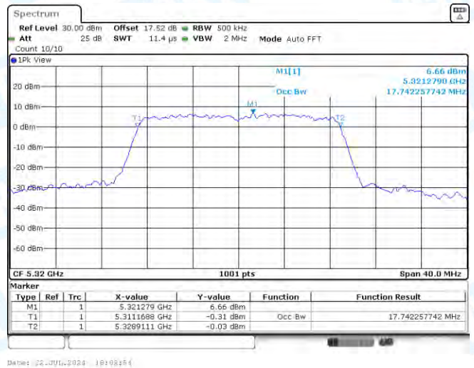
11AC20MIMO-Ant2-5320
