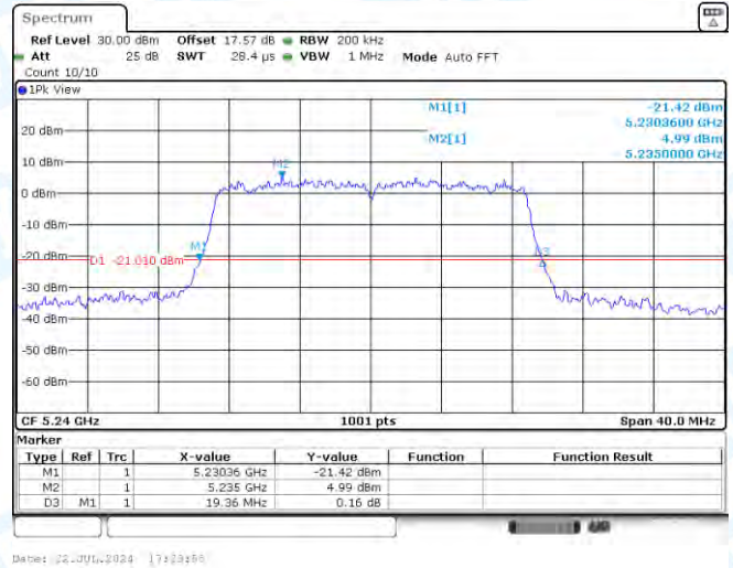
11AC20MIMO-Ant2-5240
