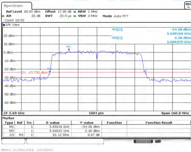
11AC80MIMO-Ant1-5690
