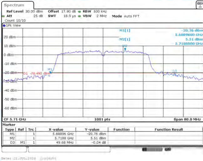
11AC40MIMO-Ant1-5710
