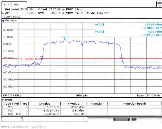
11AC80MIMO-Ant1-5610
