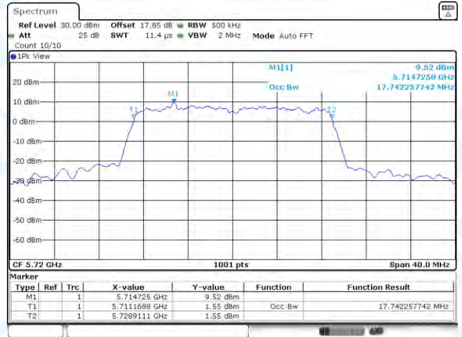
11AC20MIMO-Ant2-5720
