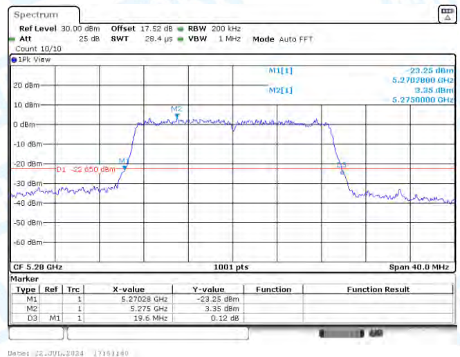
11AC20MIMO-Ant2-5280
