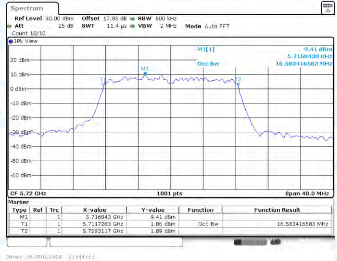
11A-Ant2-5720
