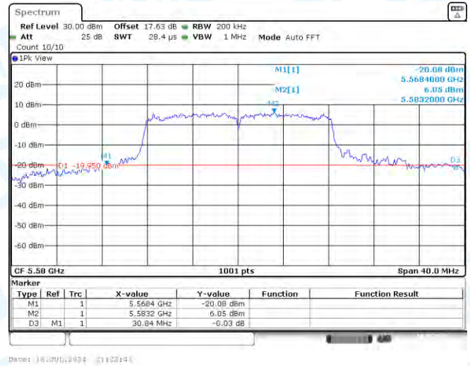
11A-Ant2-5580
