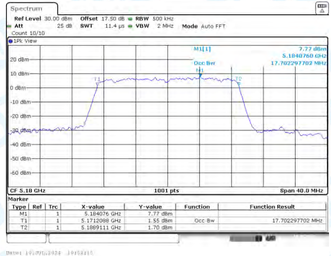
11N20MIMO-Ant2-5180
