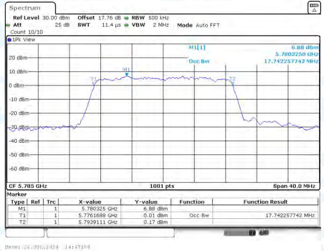
11N20MIMO-Ant2-5785
