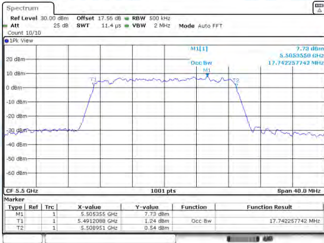
11AC20MIMO-Ant1-5500
