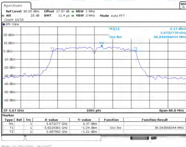
11N40MIMO-Ant1-5670
