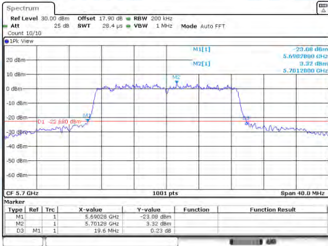
11AC20MIMO-Ant1-5700
