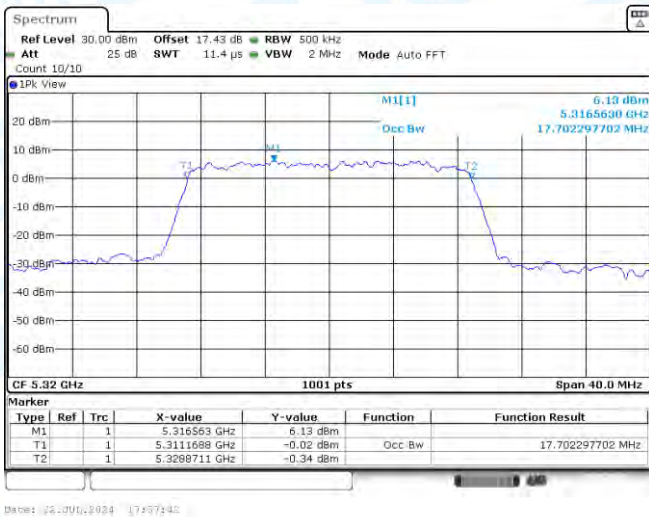
11AC20MIMO-Ant1-5320
