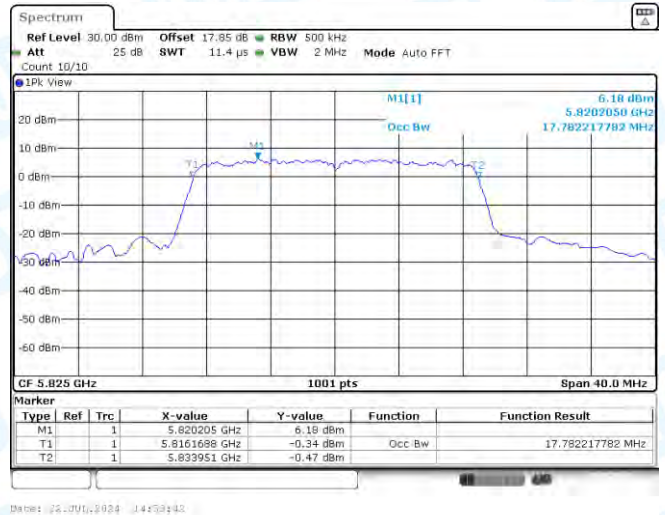
11N20MIMO-Ant2-5825
