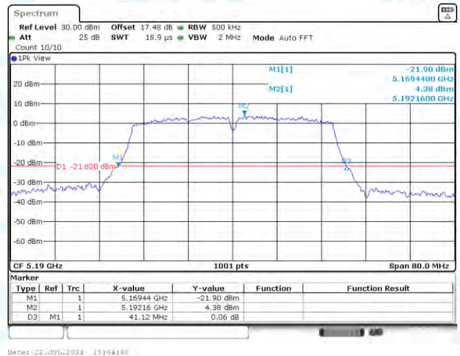
11N40MIMO-Ant2-5190
