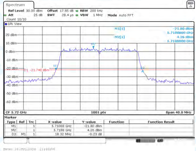
11A-Ant2-5720
