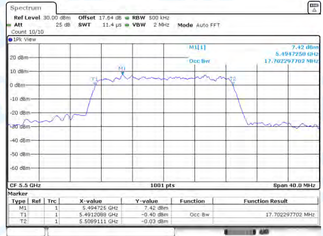
11AC20MIMO-Ant2-5500
