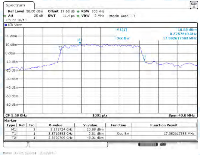
11A-Ant2-5580
