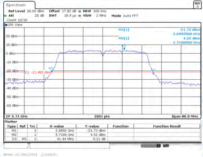
11AC40MIMO-Ant2-5710
