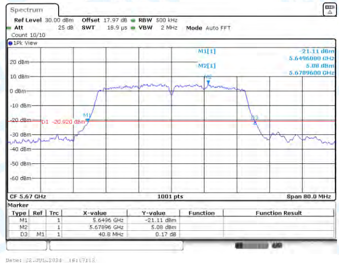
11N40MIMO-Ant2-5670
