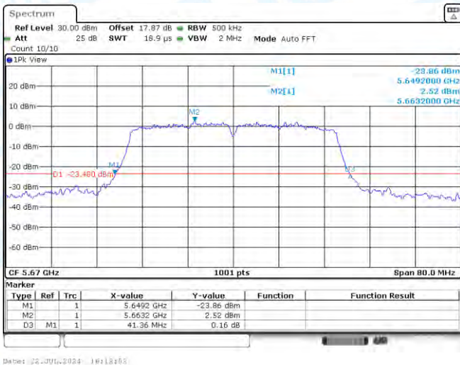
11N40MIMO-Ant1-5670
