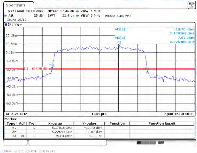
11AC80MIMO-Ant2-5210
