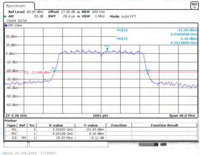
11AC20MIMO-Ant2-5260
