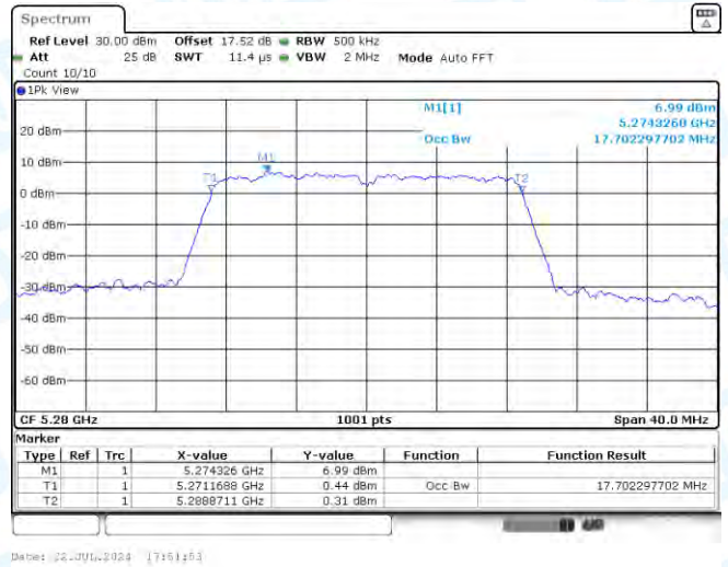
11AC20MIMO-Ant2-5280
