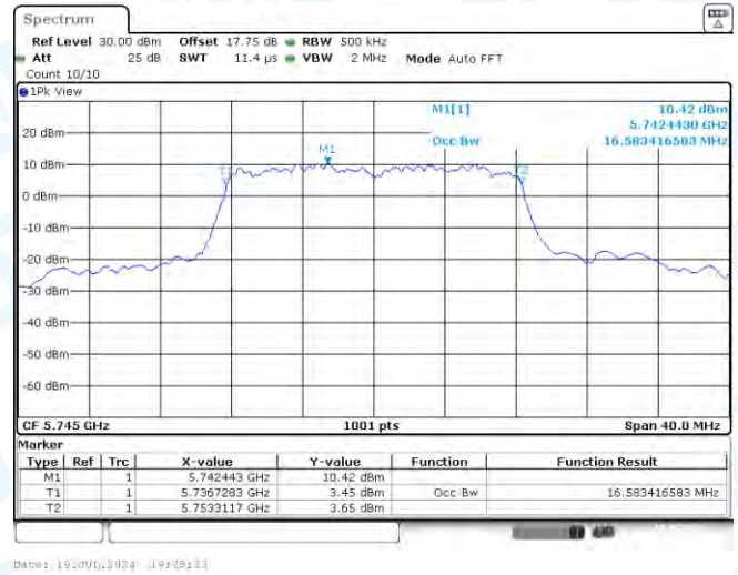
11A-Ant2-5745
