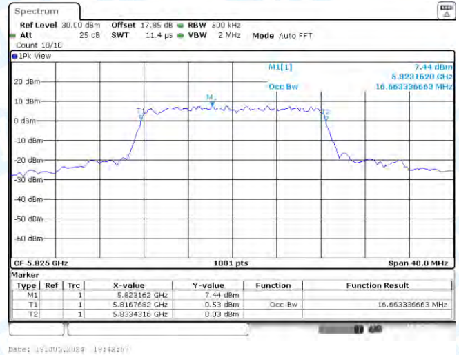
11A-Ant2-5825
