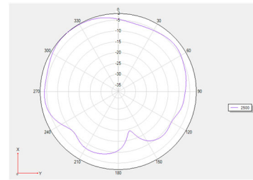
Theta =90 freq=2500MHz
