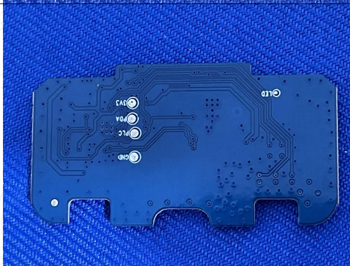
EUT View 22
