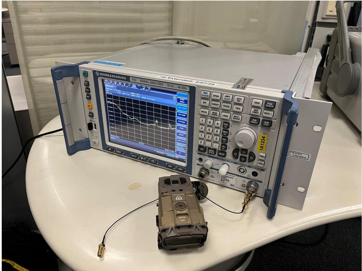
Conducted Antenna Port Tests
