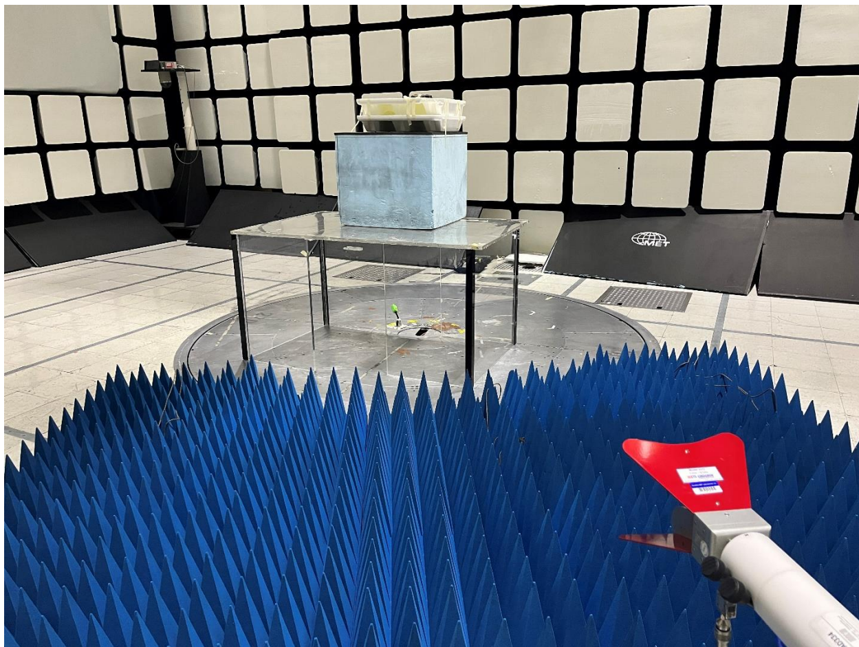
Radiated Emissions Above 1GHz EUT at 1.5m height
