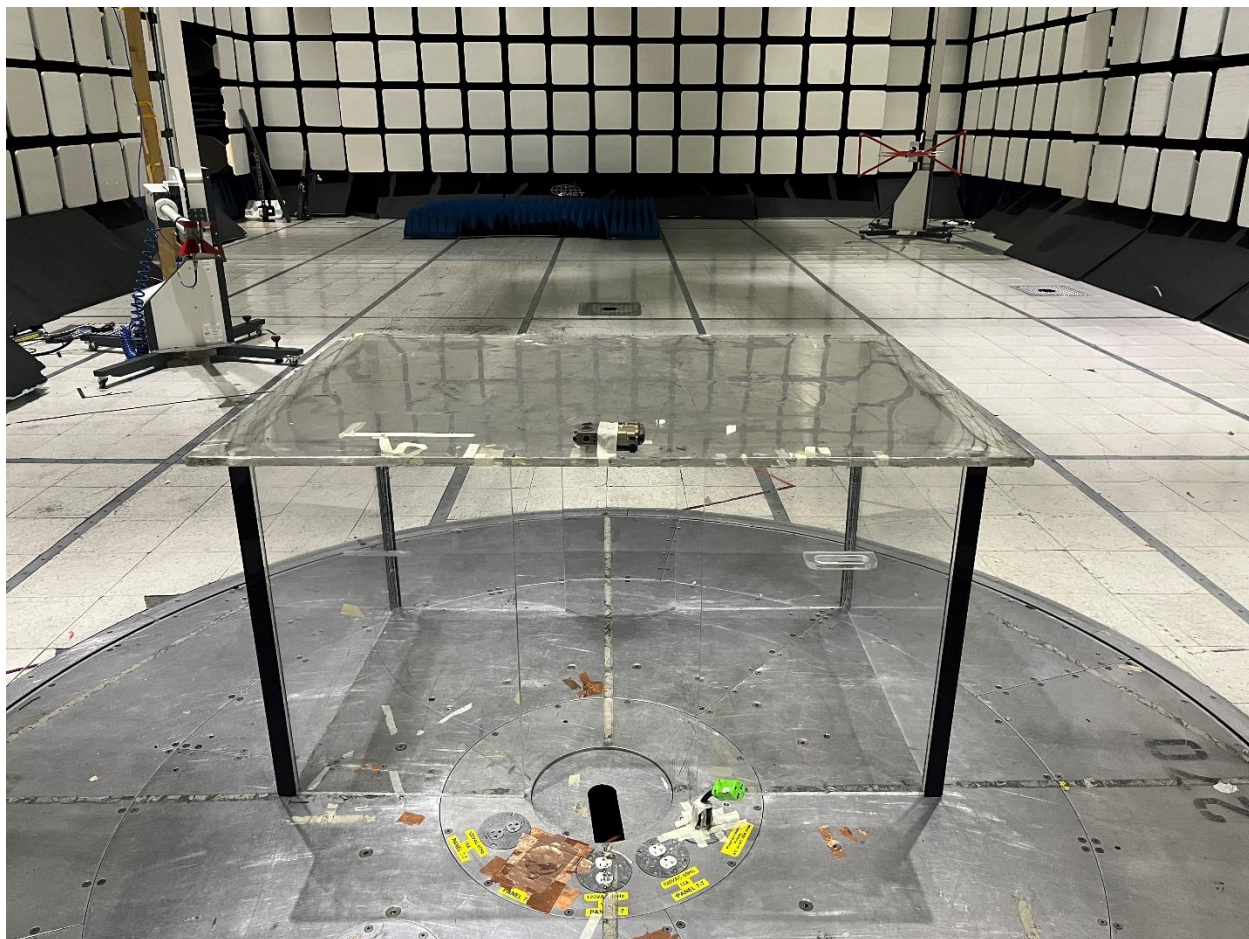
Radiated Emissions 30MHz – 1GHz EUT at 80cm height
