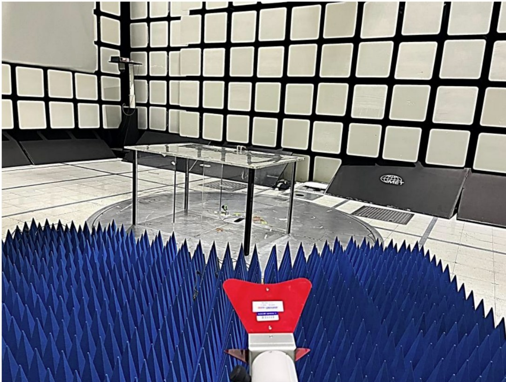
Photograph 6. Radiated Emissions, 2K Standalone, (1 GHz – 18 GHz), Setup Antenna View
