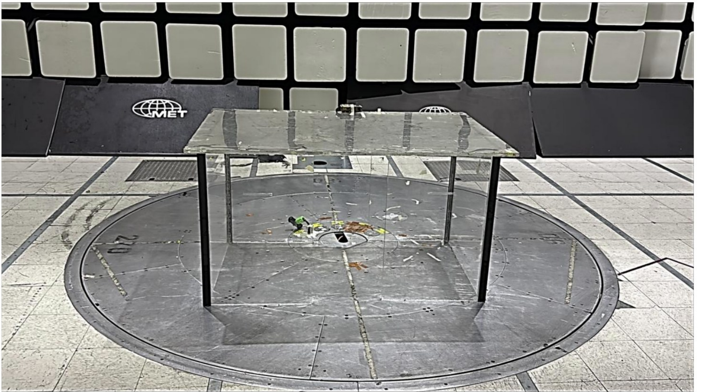
Photograph 1. Radiated Emissions, 2K Standalone, (30 MHz – 1000 MHz), Setup Front View
