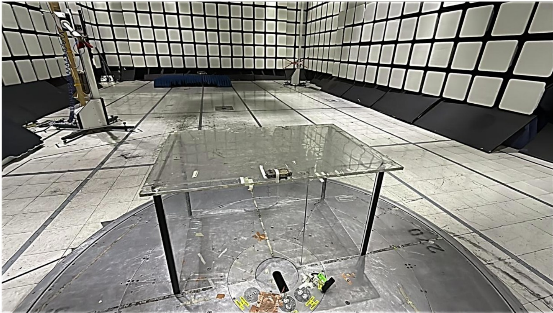
Photograph 2. Radiated Emissions, 2K Standalone, (30 MHz – 1000 MHz), Setup Rear View
