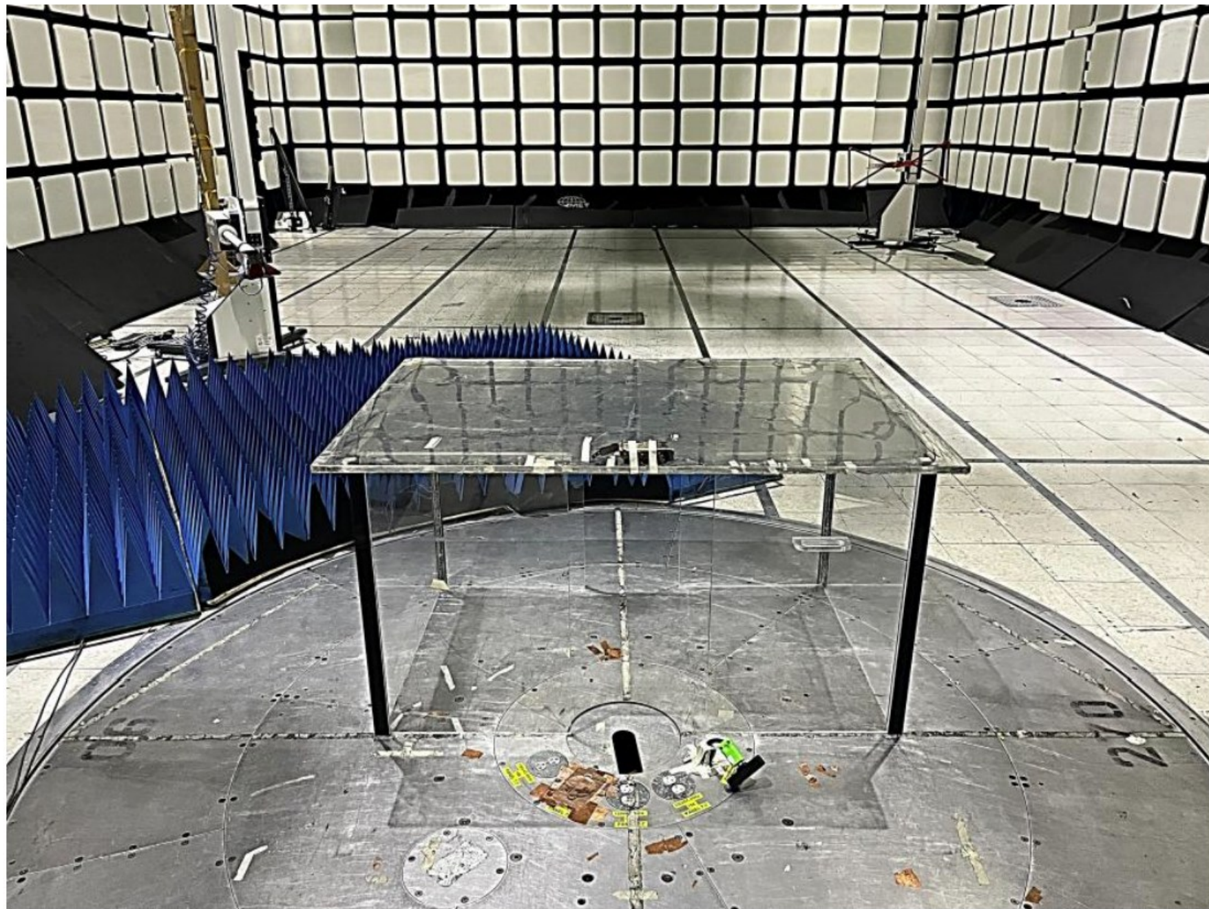
Photograph 5. Radiated Emissions, 2K Standalone, (1 GHz – 18 GHz), Setup Rear View
