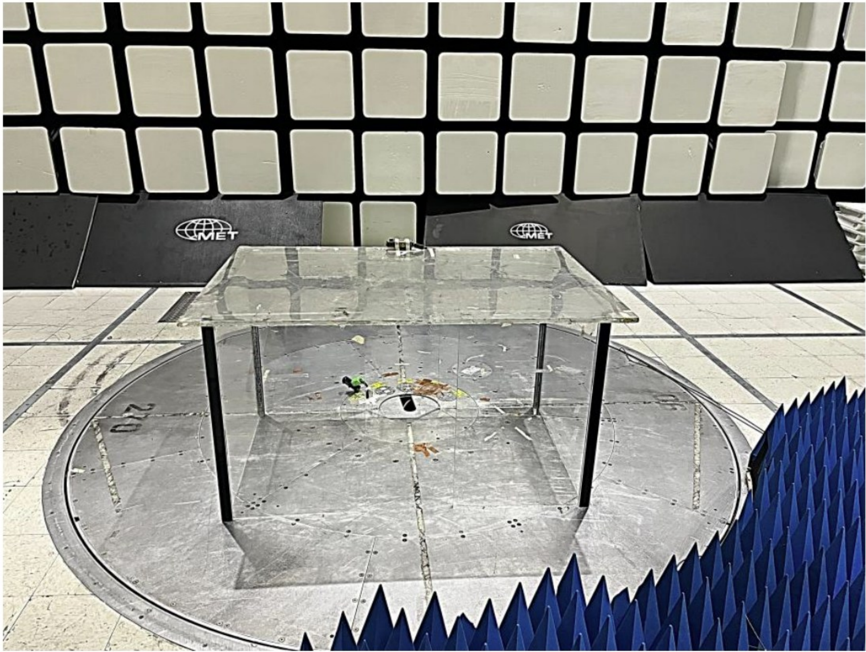
Photograph 4. Radiated Emissions, 2K Standalone, (1 GHz – 18 GHz), Setup Front View
