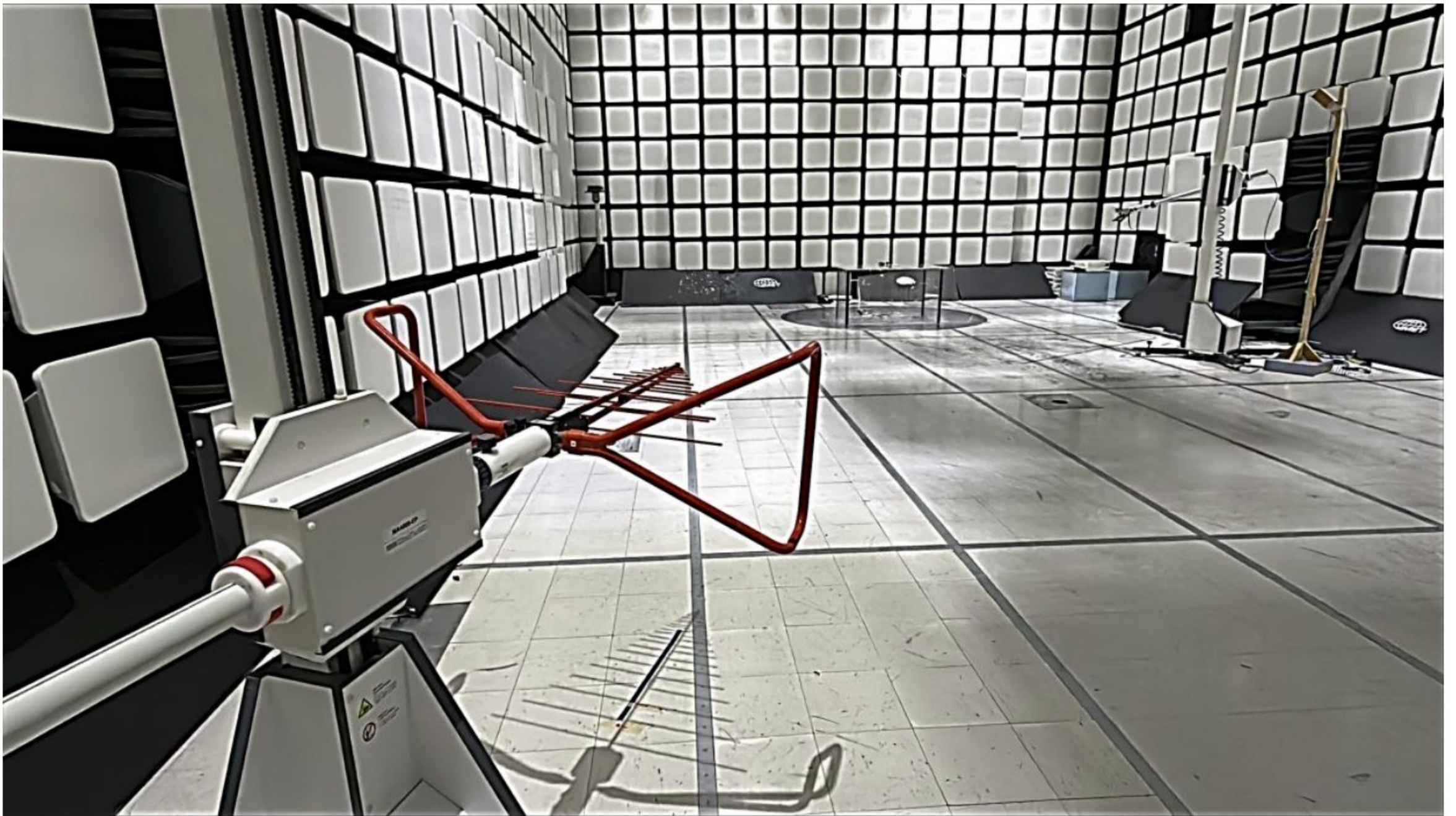
Photograph 3. Radiated Emissions, 2K Standalone, (30 MHz – 1000 MHz), Setup Antenna View
