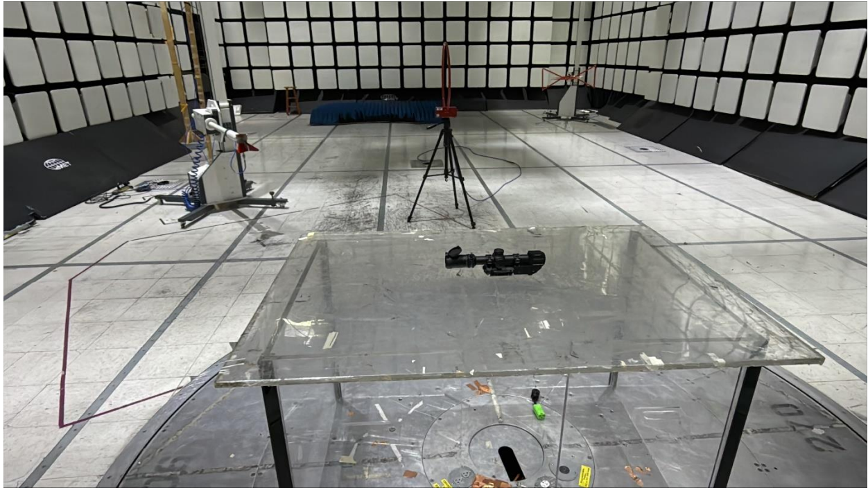
Radiated Emissions 9kHz – 30MHz (EUT View) EUT at 80cm height
