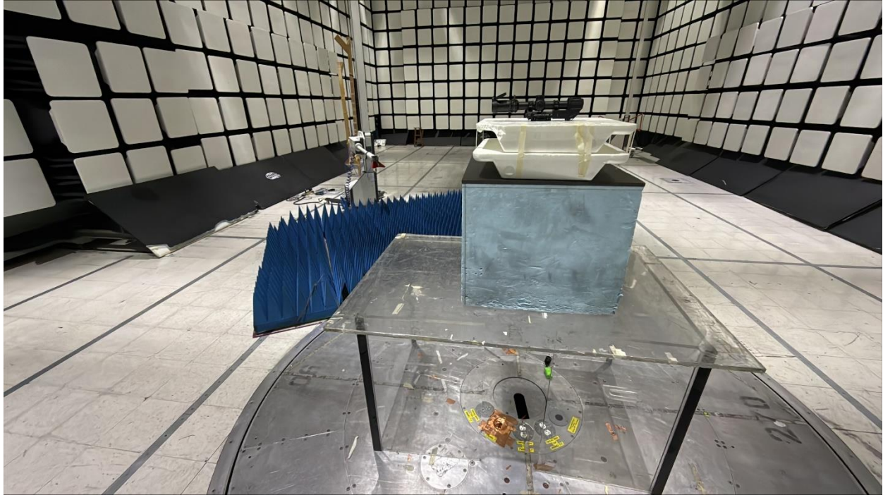
Radiated Emissions Above 1GHz (EUT View) EUT at 1.5m height
