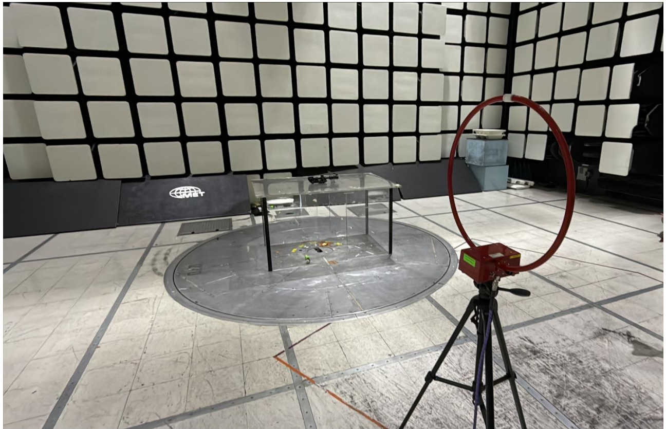
Radiated Emissions 9kHz – 30MHz (Antenna View) EUT at 80cm height
