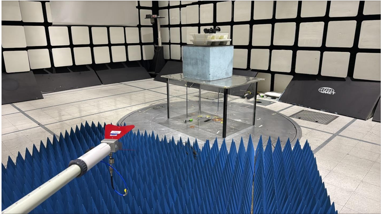
Radiated Emissions Above 1GHz (Antenna View) EUT at 1.5m height
