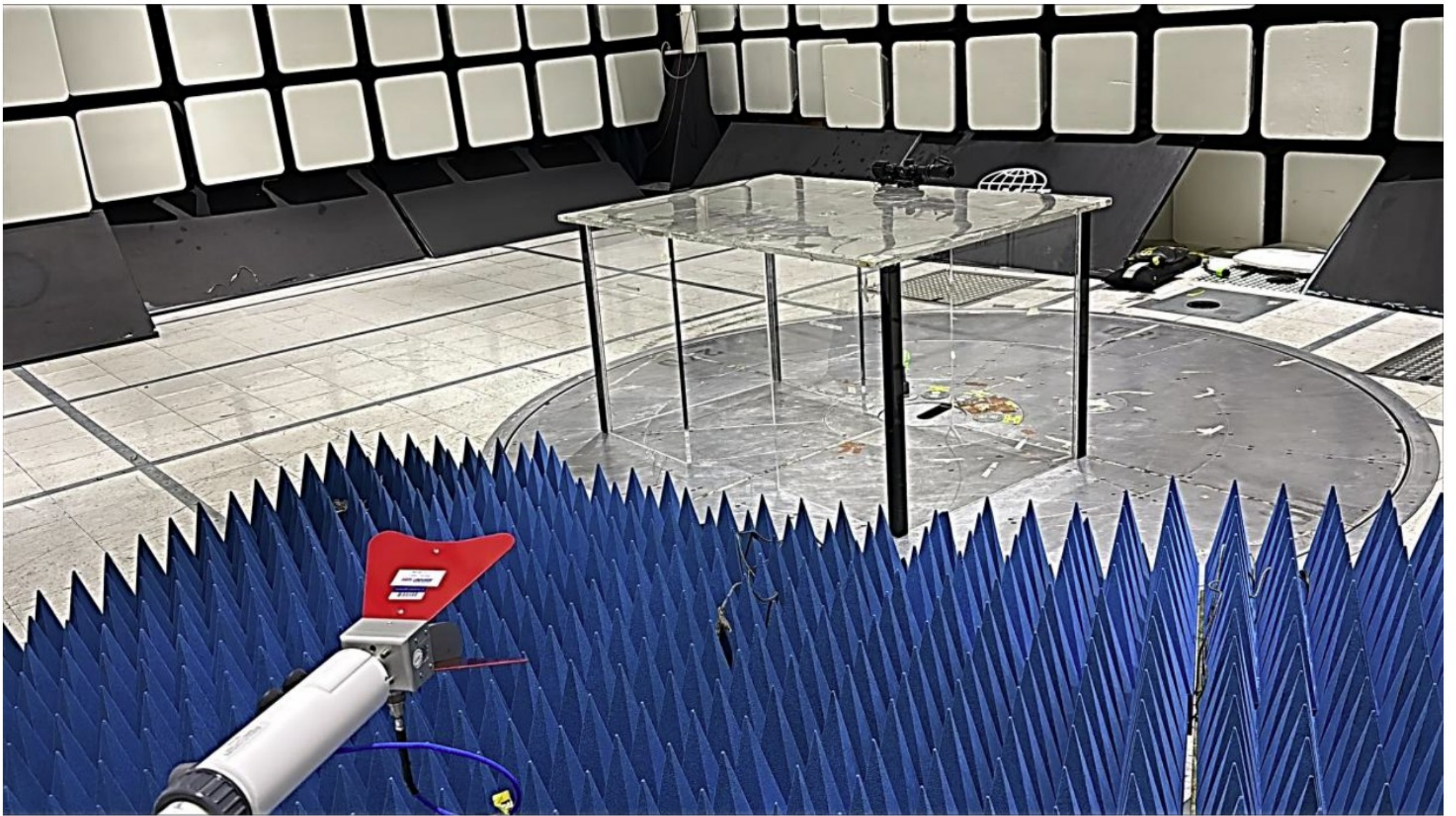
Photograph 6. Radiated Emissions, Lock, (1 GHz – 18 GHz), Setup Antenna View
