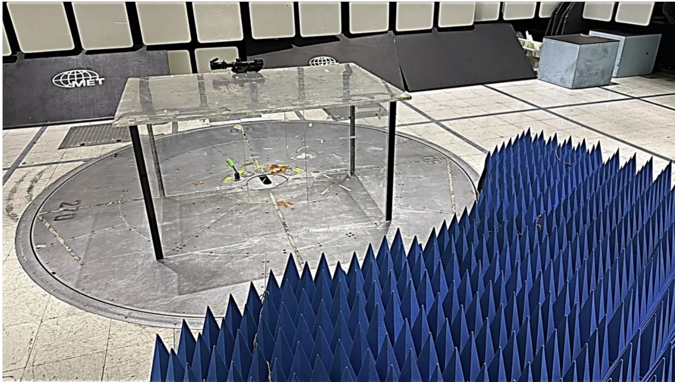
Photograph 7. Radiated Emissions, Lock, (18 GHz - 40 GHz), Setup Front View
