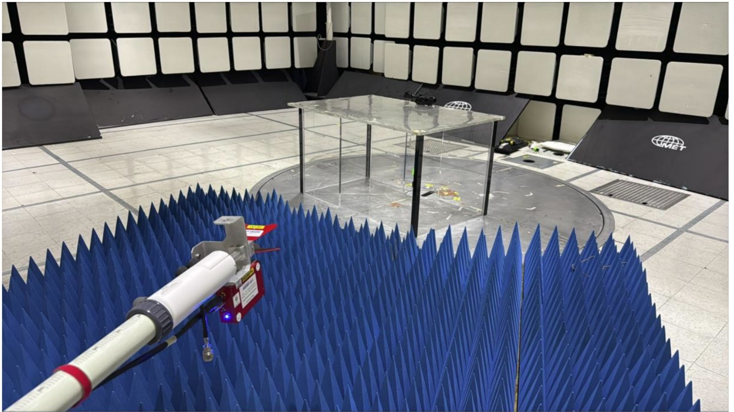
Photograph 9. Radiated Emissions, Lock, (18 GHz - 40 GHz), Setup Antenna View
