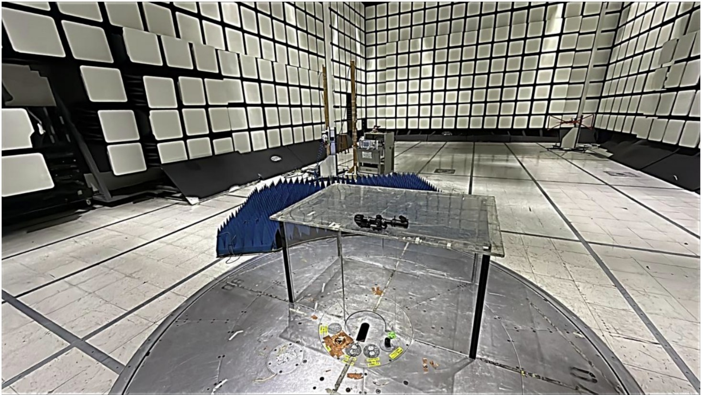
Photograph 8. Radiated Emissions, Lock, (18 GHz - 40 GHz), Setup Rear View
