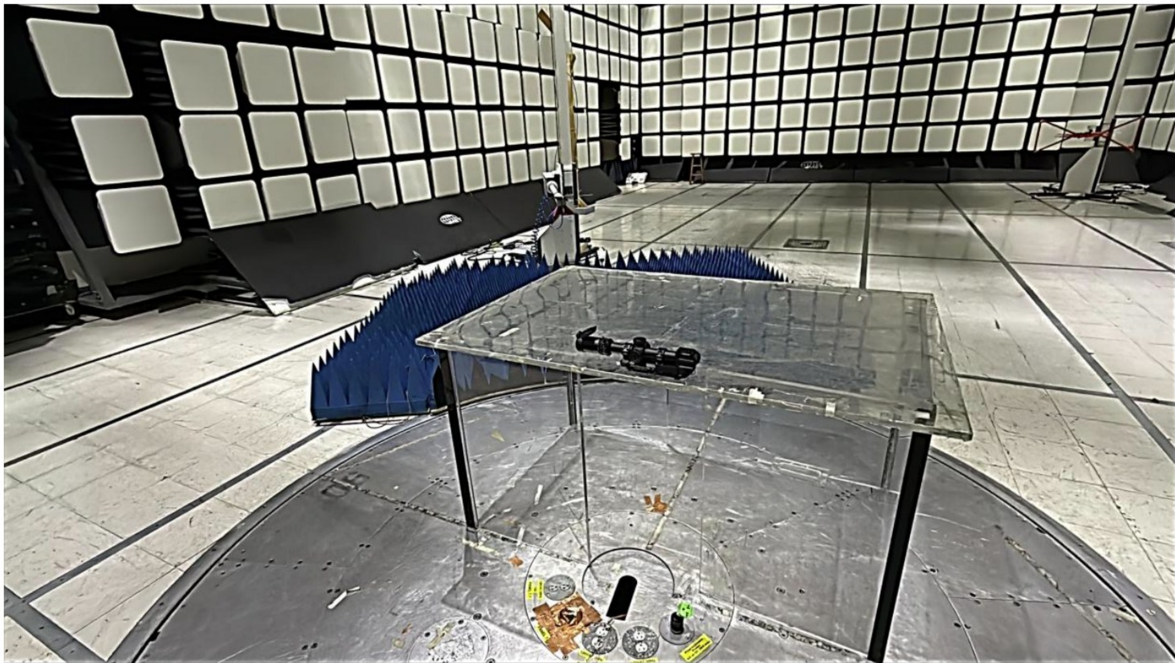
Photograph 5. Radiated Emissions, Lock, (1 GHz – 18 GHz), Setup Rear View
