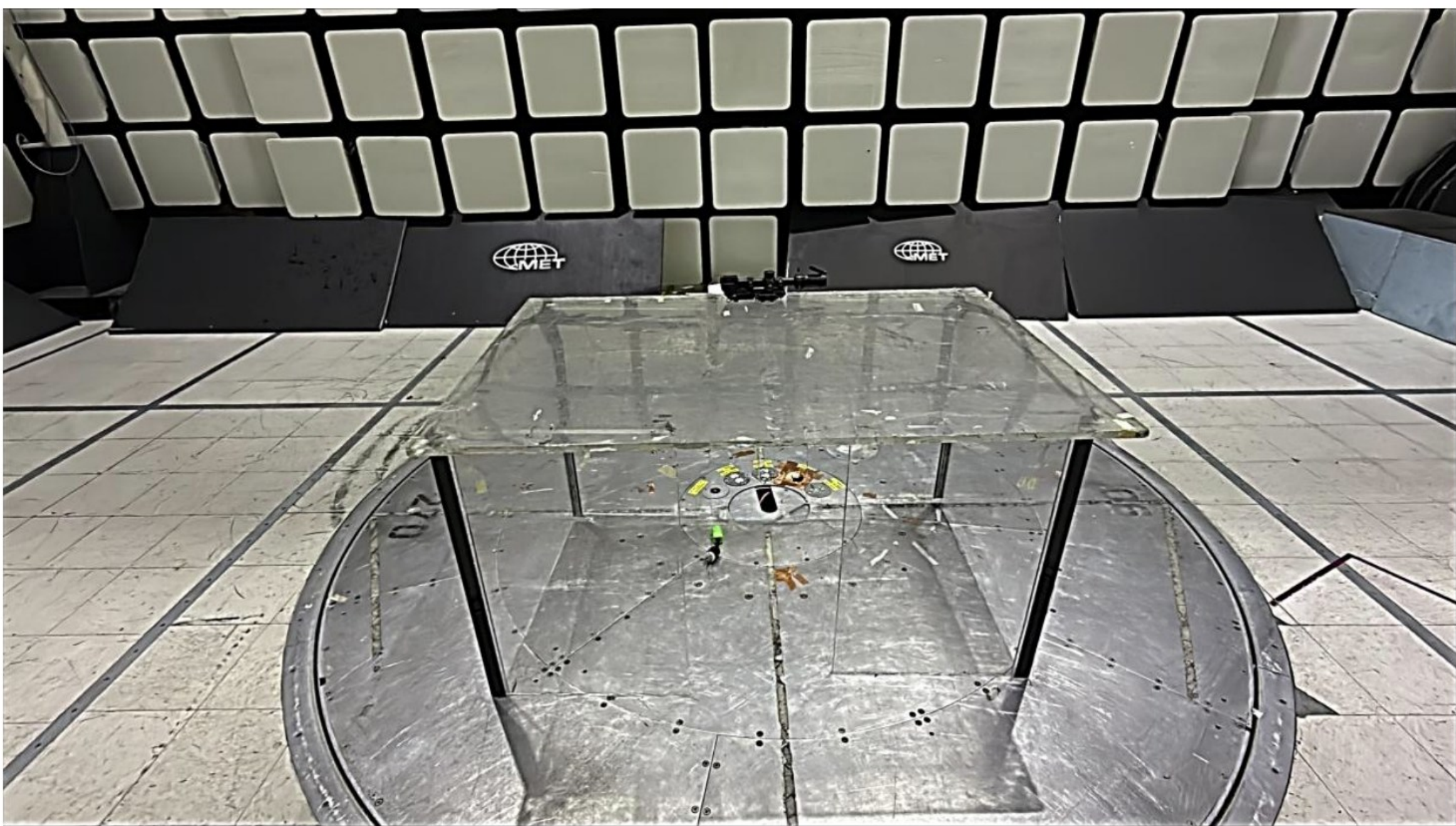
Photograph 1. Radiated Emissions, Lock, (30 MHz – 1000 MHz), Setup Front View
