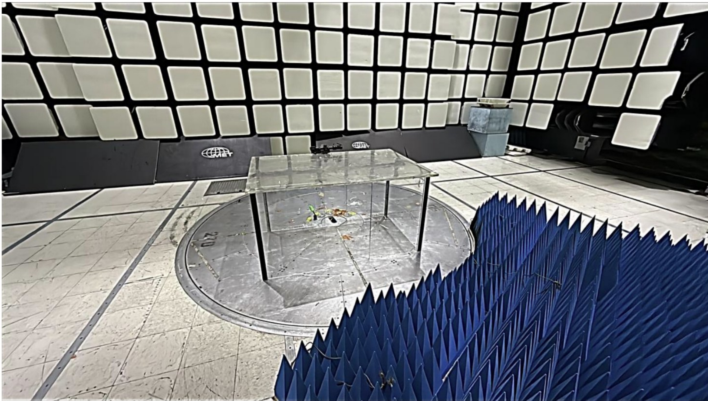
Photograph 4. Radiated Emissions, Lock, (1 GHz – 18 GHz), Setup Front View
