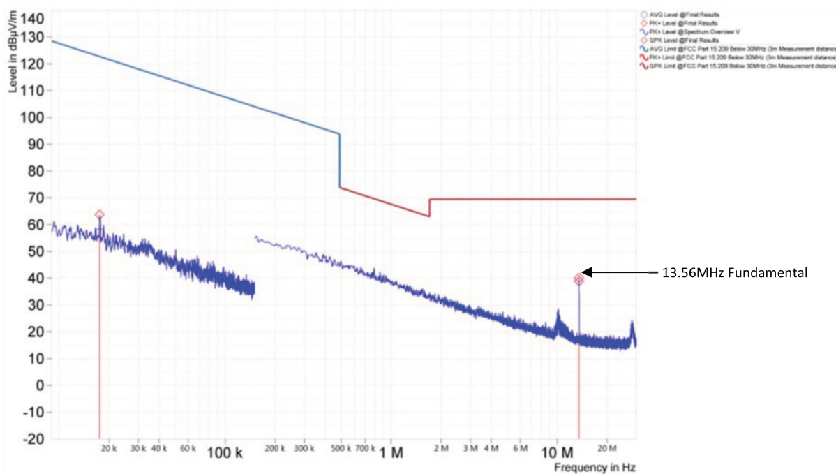
Figure 11. Out of Band Emissions Below 30MHz (Coaxial Loop)
