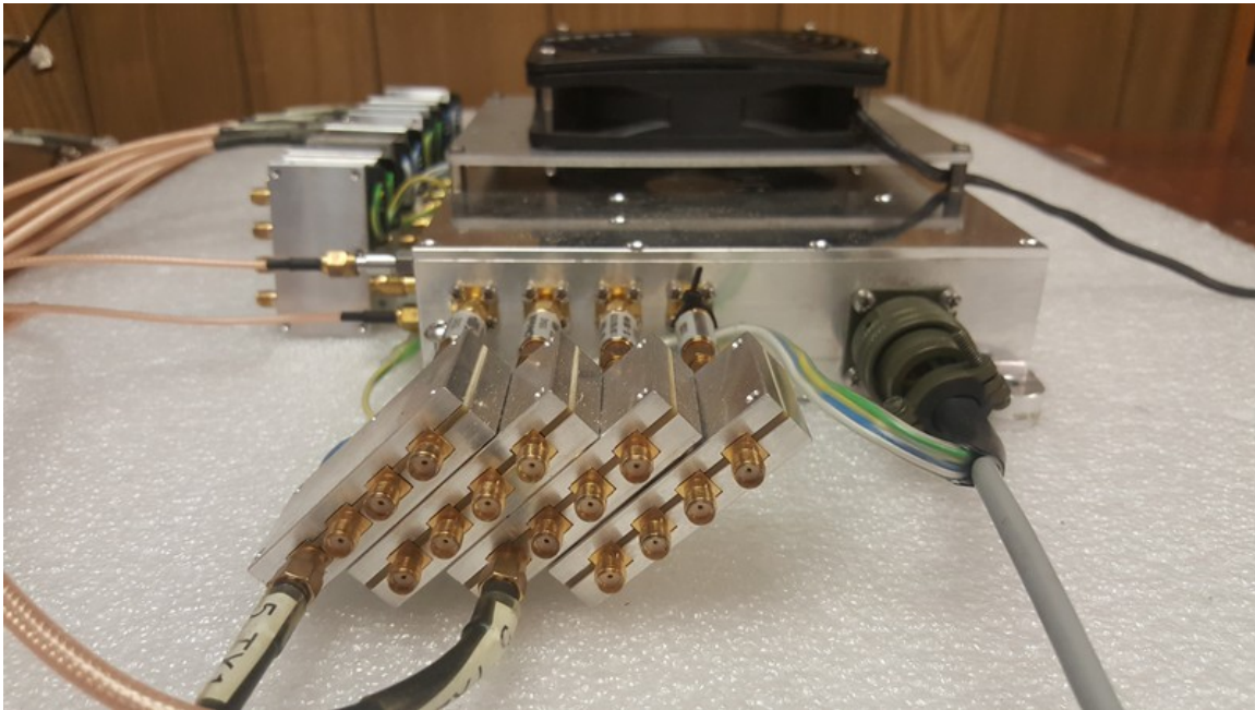
Controller Right Side View
