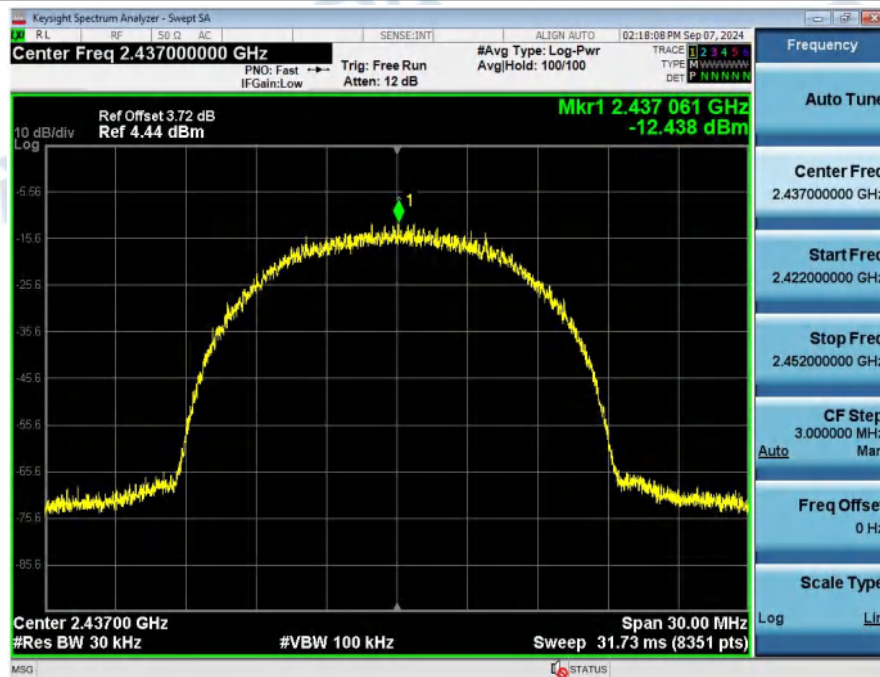
Power_Spectral_Density_NVNT_ANT1_802_11b_2437
