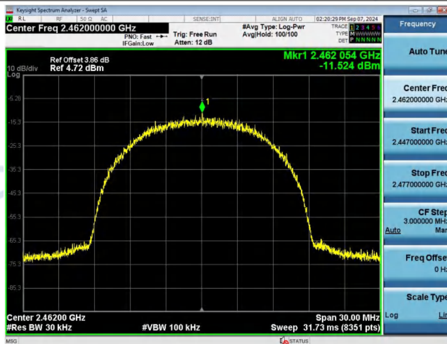
Power_Spectral_Density_NVNT_ANT1_802_11b_2462
