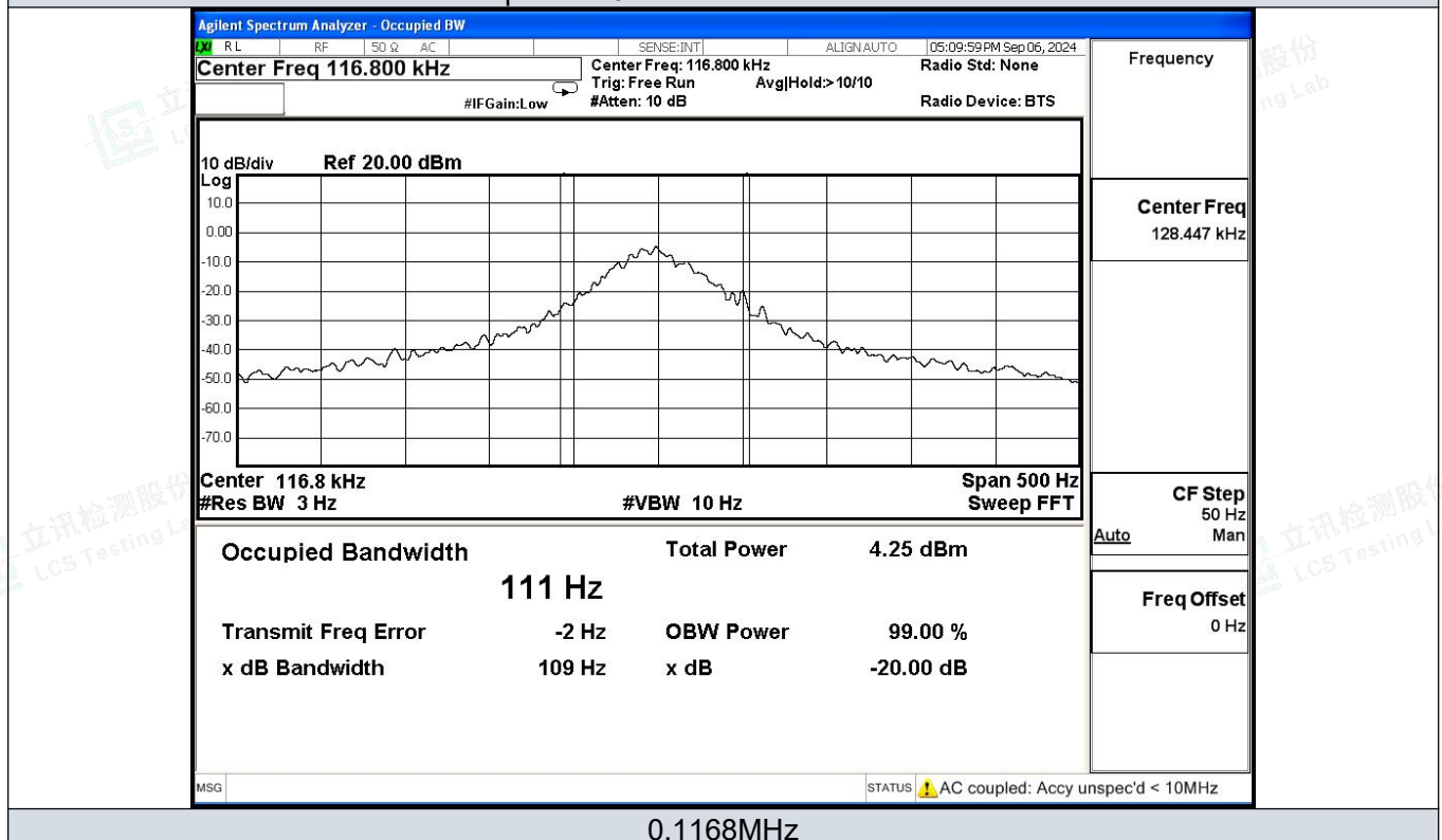
Test plot of 20 dB Bandwidth Measurement
