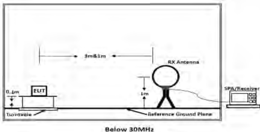
Figure 1. Below 30MHz
