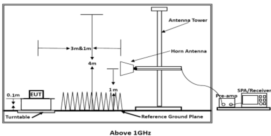
Figure 3. Above 1GHz
