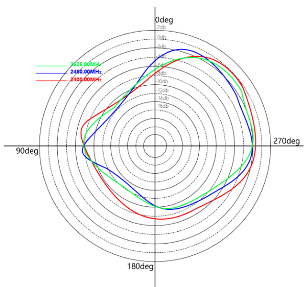
图 6 YOZ 平面天线增益图 Figure 6 Gain of YOZ planar antenna
