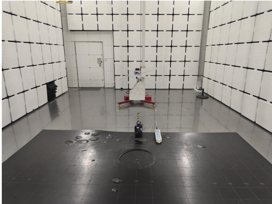
Emissions in Non-restricted Frequency Bands(0.009 MHz – 30MHz)
