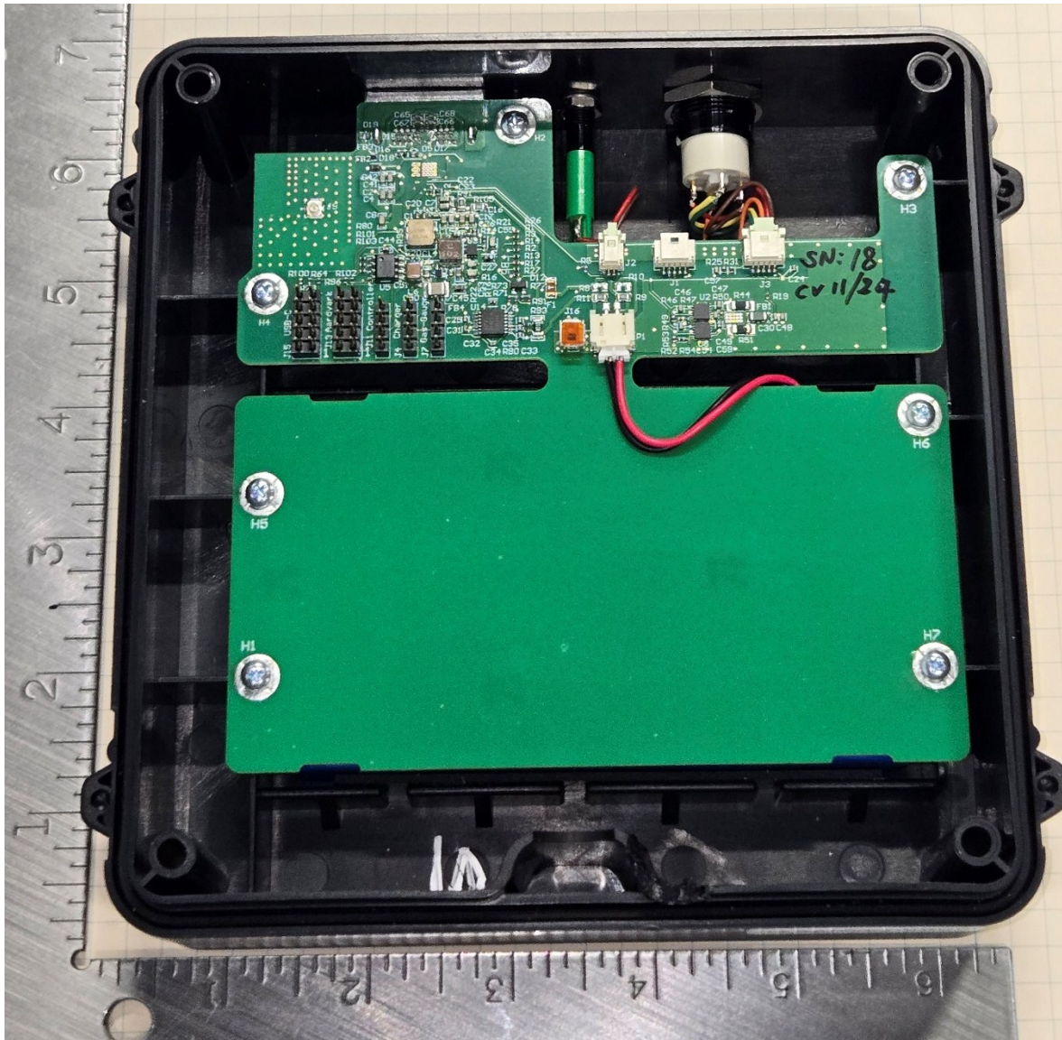
Figure 8: Back Half Internal View
