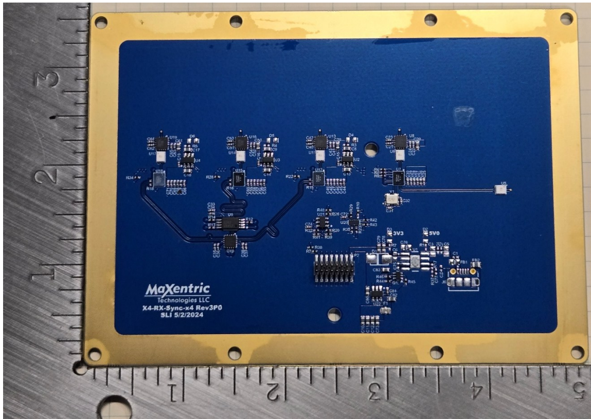
Figure 10: Backside of Antenna Board (higher quality image submitted in attachments)
