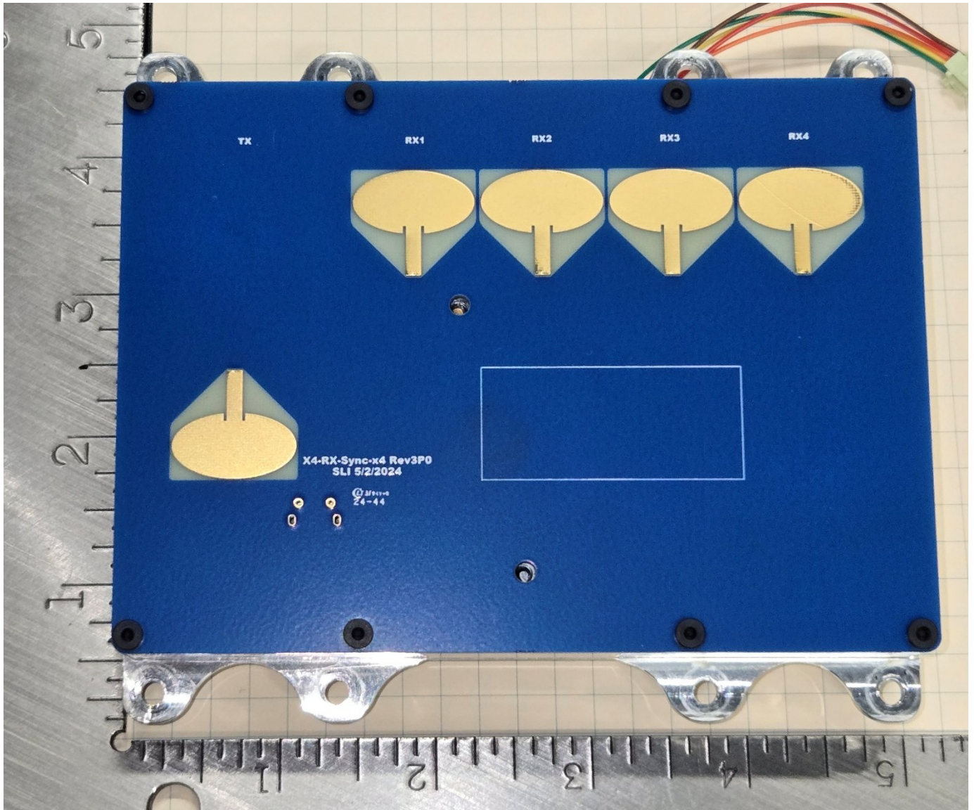
Figure 9: Antenna Board mounted to CNC Shield (higher quality image submitted in attachments)
