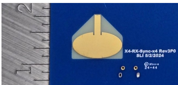
Figure 20: UWB TX Antenna
