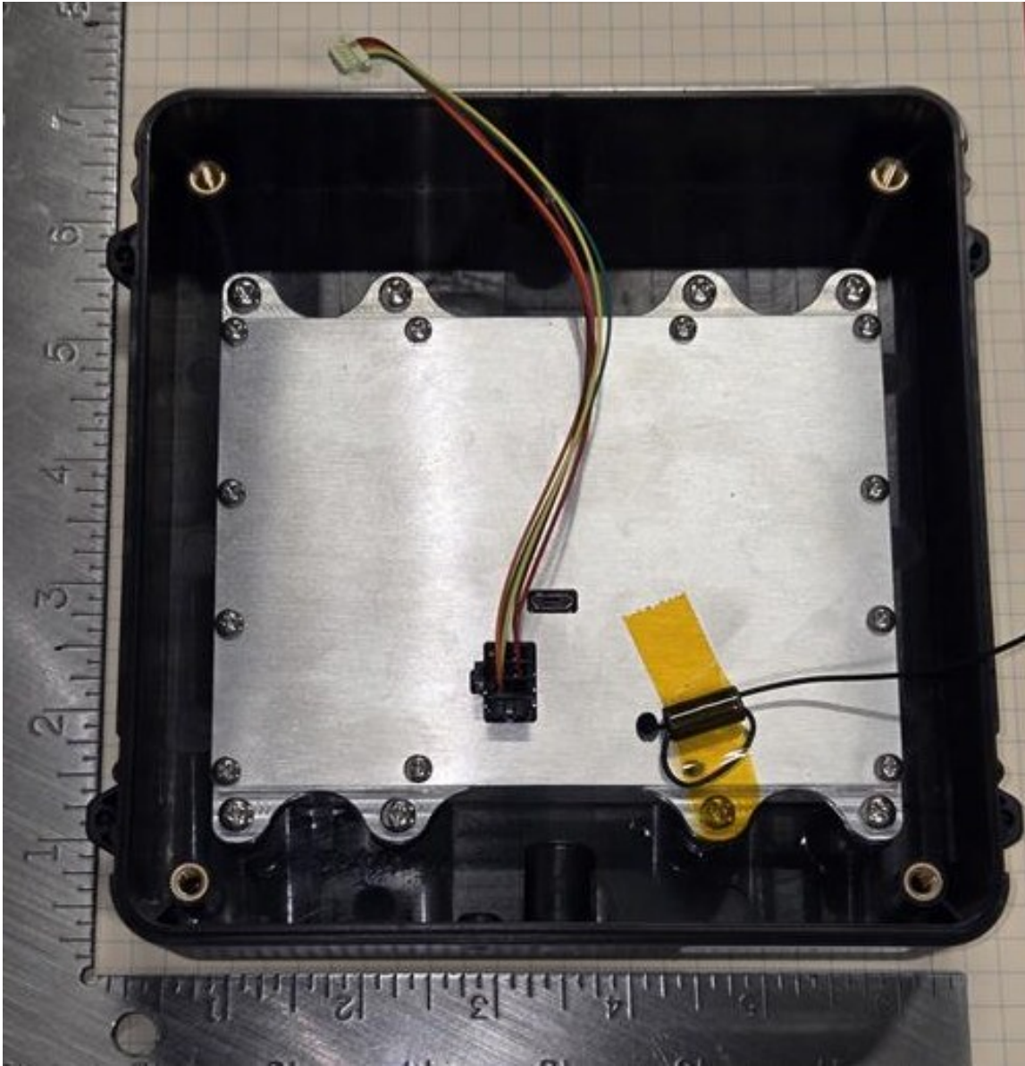
Figure 7: Front Half Internal View
