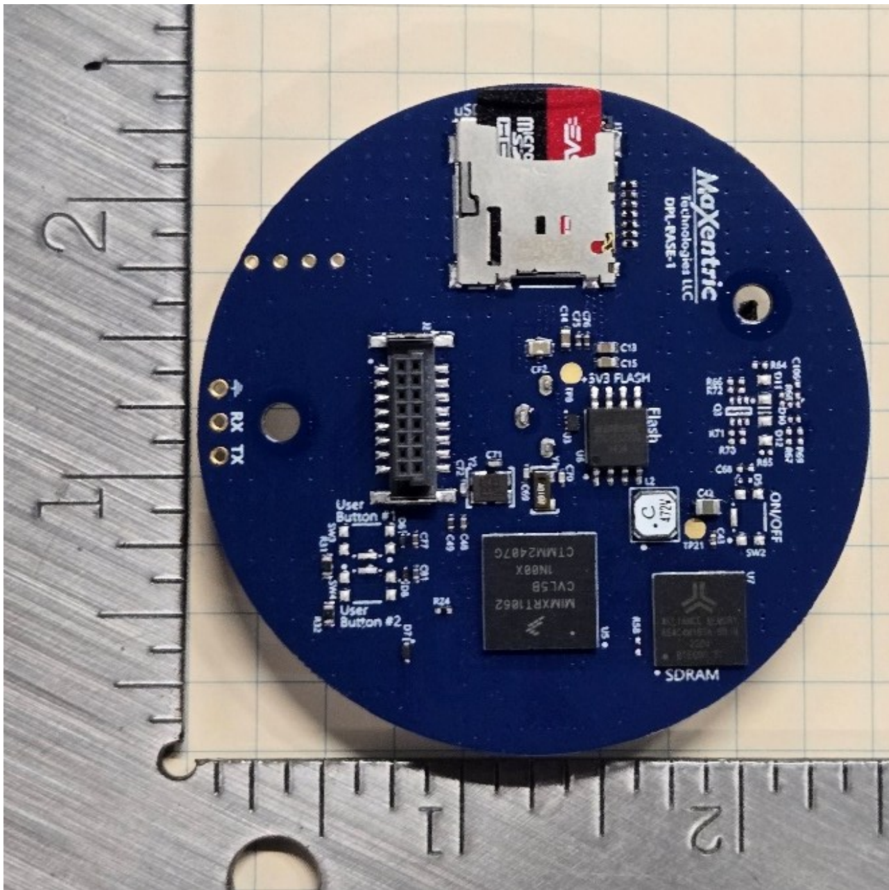
Figure 12: Frontside of Main Board (higher quality image submitted in attachments)
