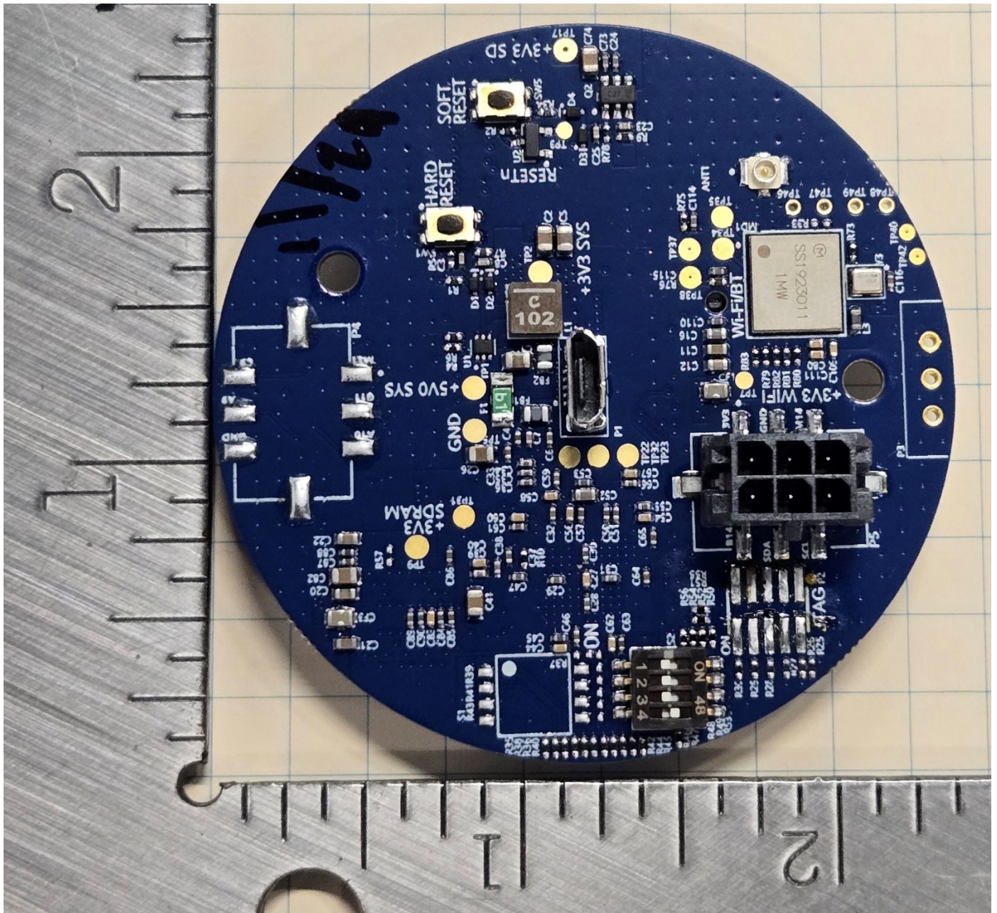
Figure 11: Backside of Main Board (higher quality image submitted in attachments)
