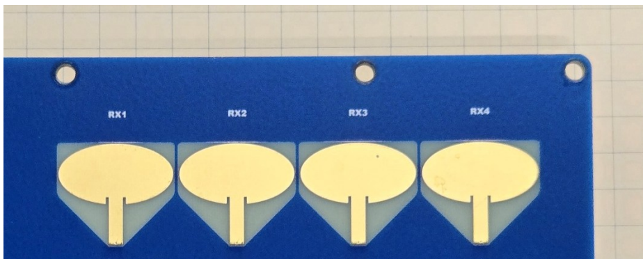
Figure 19: UWB RX Antennas
