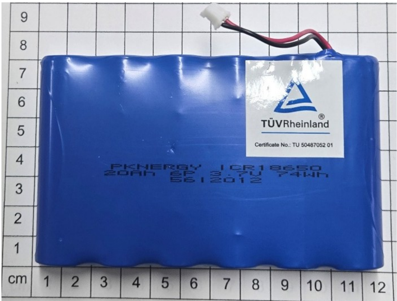
Figure 16: Battery Front
