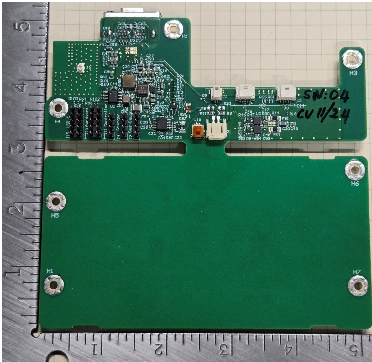
Figure 14: Backside of PSU Board (higher quality image submitted in attachments)
