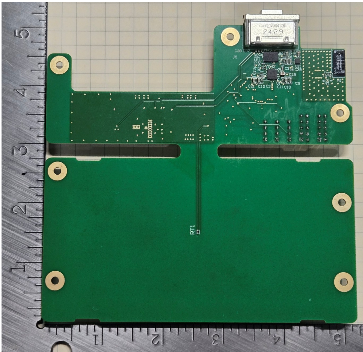
Figure 15: Frontside of PSU Board (higher quality image submitted in attachments)
