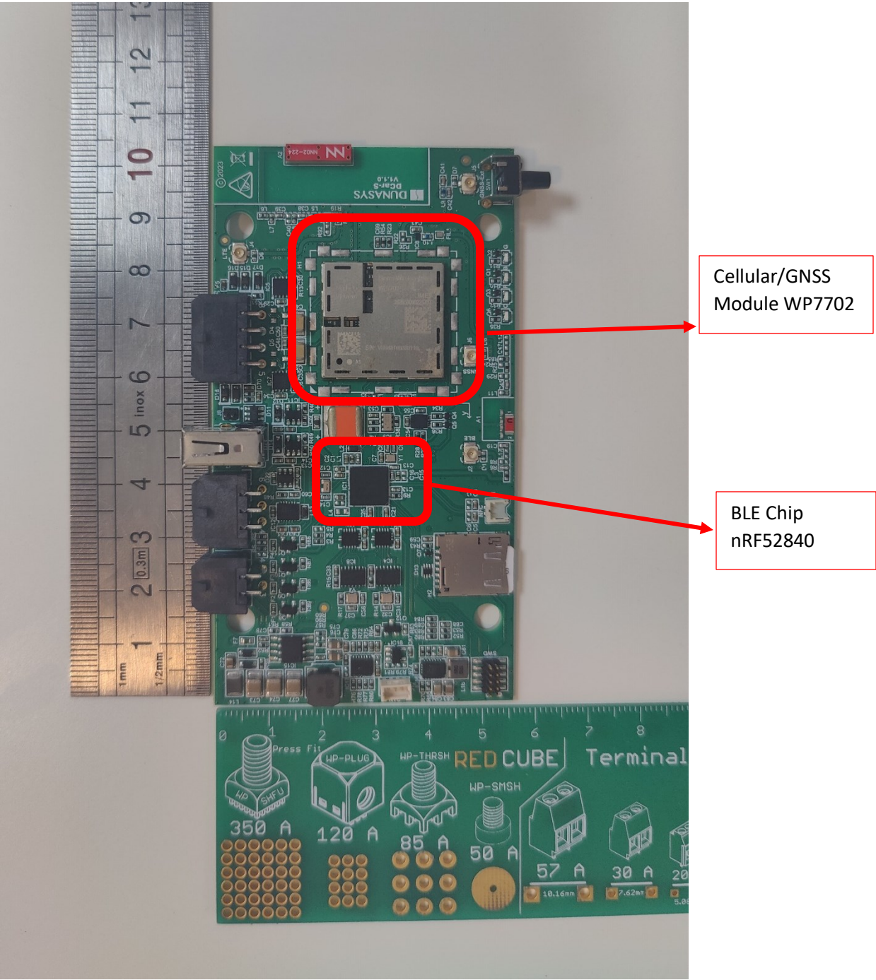
Top View
