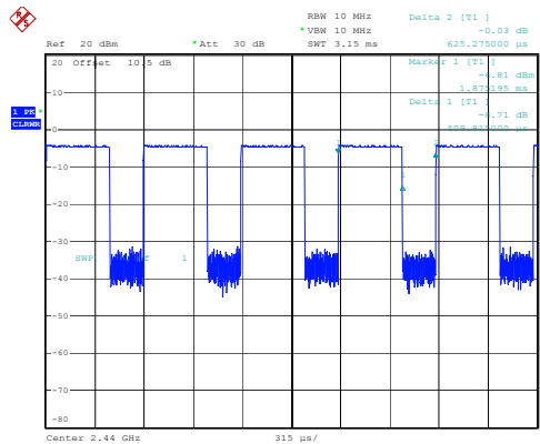
BLE_1M_Middle_Channel
