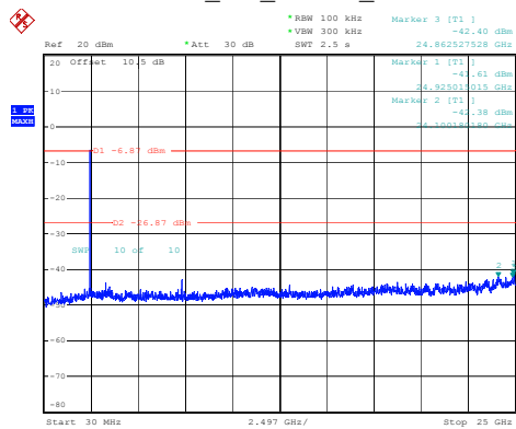
BLE_2M_Middle_Channel
