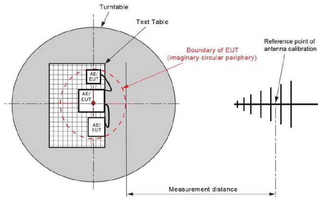
Figure C.1 – Measurement distance
