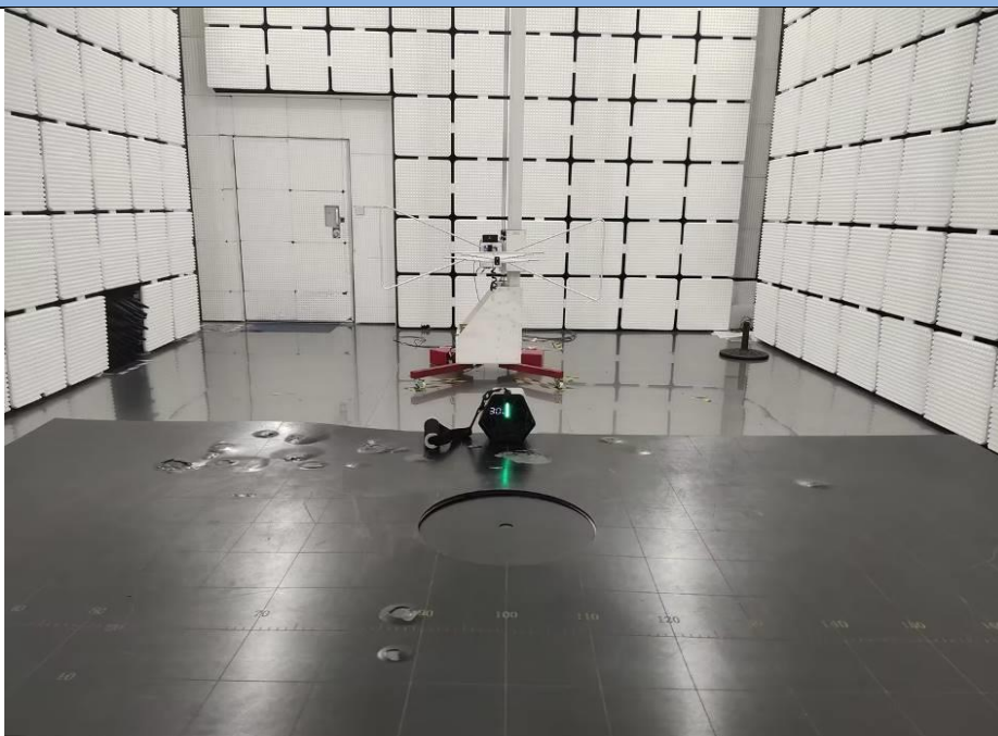
Radiated emissions (Below 1GHz)
