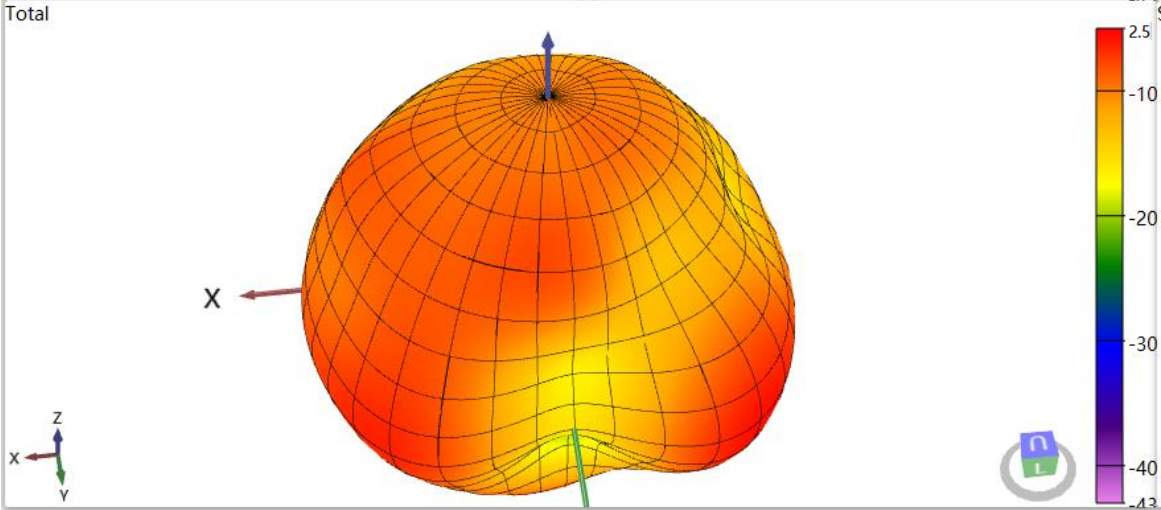
2480MHz 3D-Total Pattern
