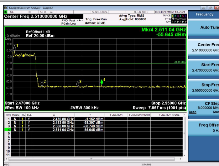
2DH5-Ant1-Hop 2480-PASS
