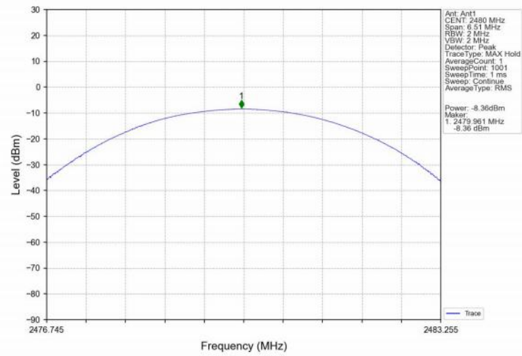
8DPSK_3DH5_HCH_2480MHz_Ant1_NTNV
