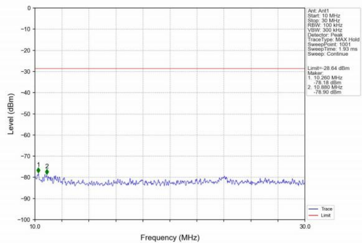
Pi/4DQPSK_2DH5_MCH_2441MHz_Ant1_NTNV
