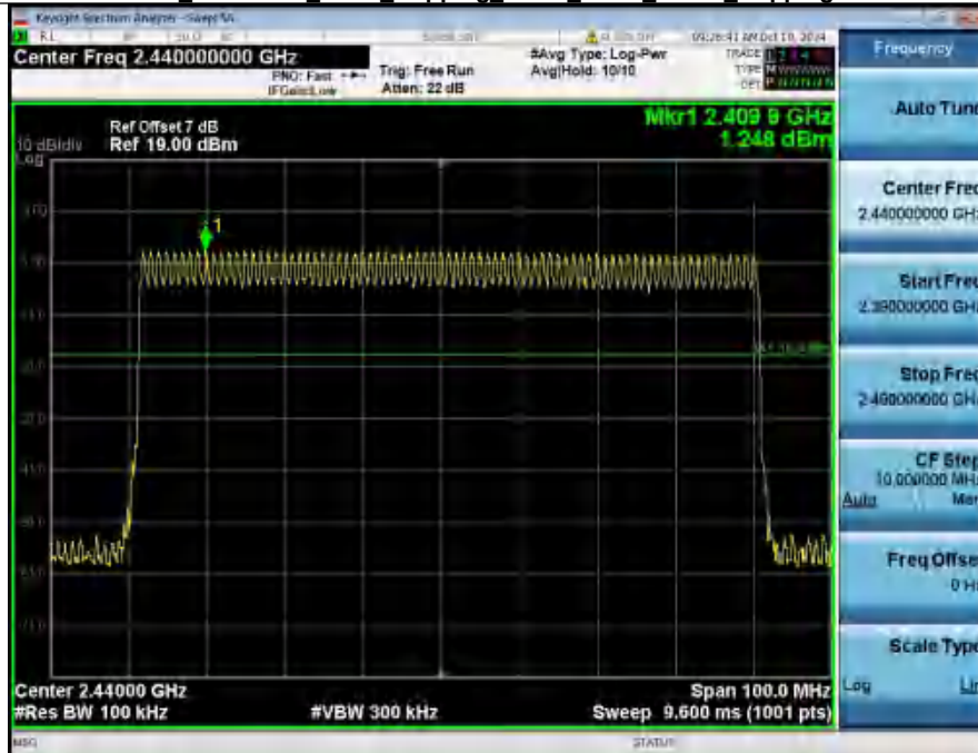
2_Band_Edge_(Hopping)_NVNT_ANT1_2-DH1_Hopping
