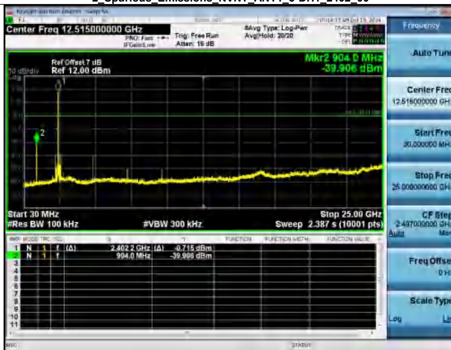
2_Spurious_Emissions_NVNT_ANT1_3-DH1_2402_00
