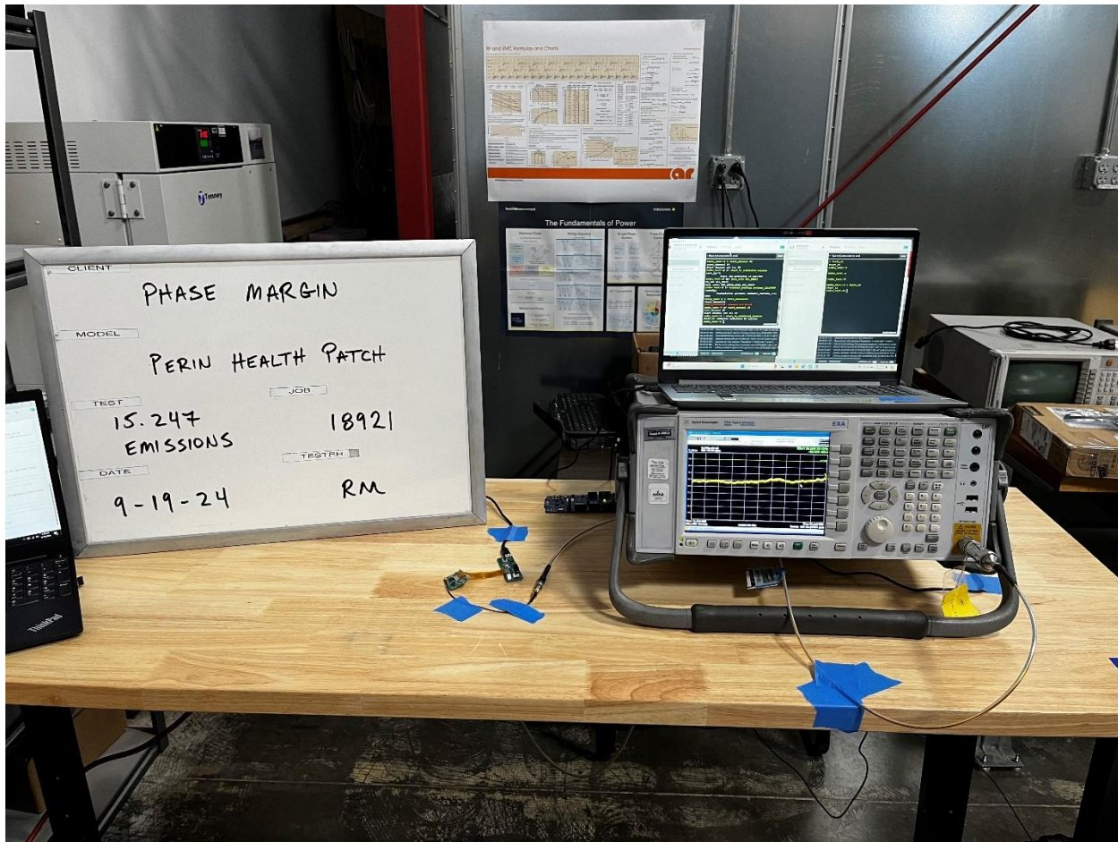
Conducted Emissions, table-top evaluation View 2
