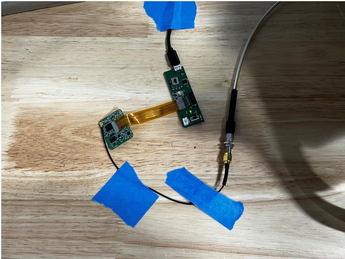
Conducted Emissions, table-top evaluation View 1
