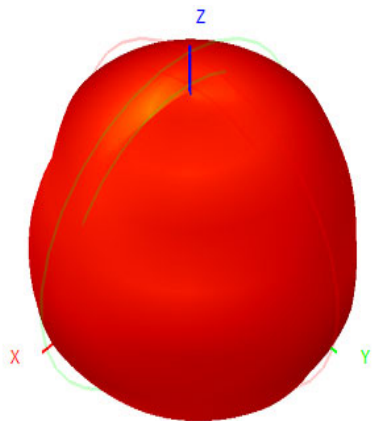
2400.0MHz H+V, Eff: 18.0%
