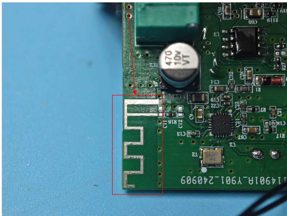
BT Antenna-Only Receiver
