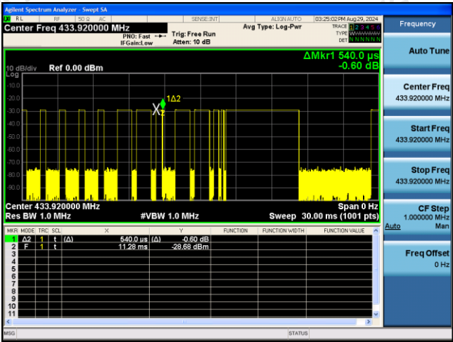
(Time per burst: 0.54ms*4pcs)
