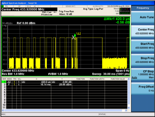
(Time per burst: 0.42 ms*5pcs)
