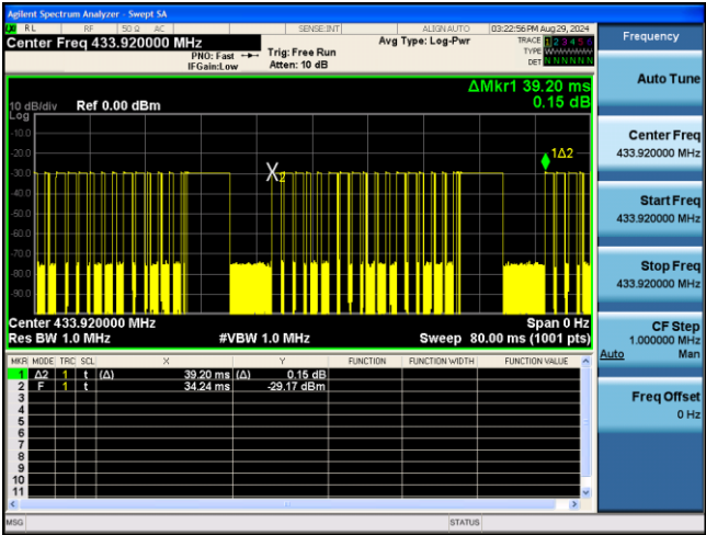
(Transmit cycle 39.20ms)
