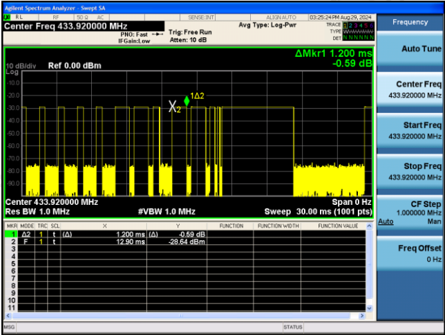
(Time per burst: 1.20 ms*8pcs)
