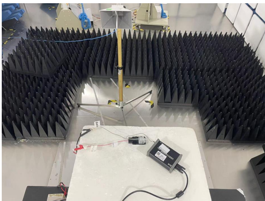
Close-up-UWB-1m
