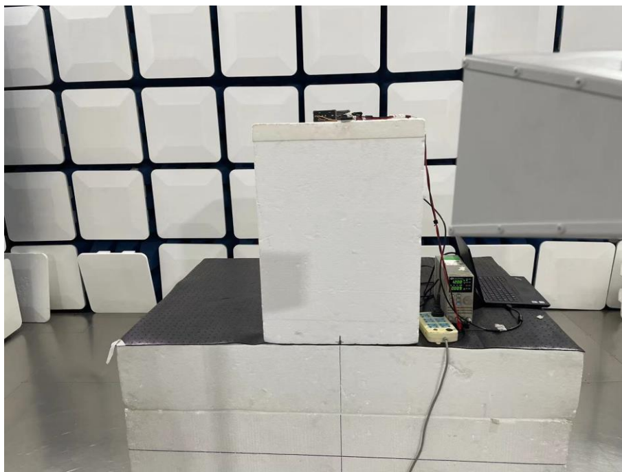
Above 1GHz-UWB-1m
