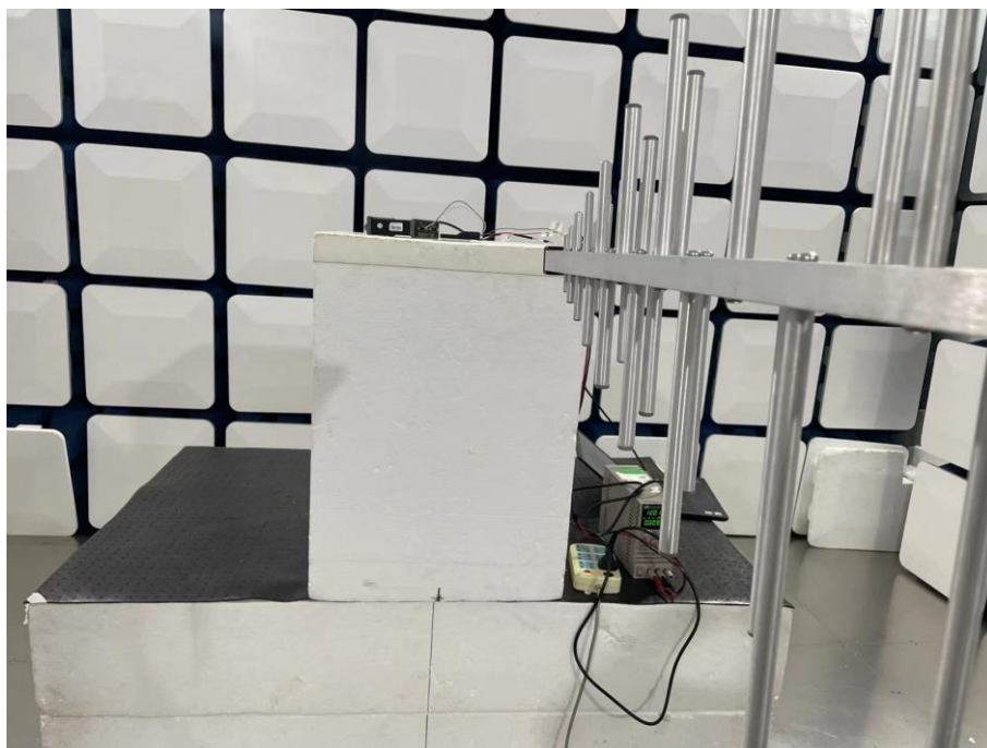
30MHz-1GHz-UWB-1m
