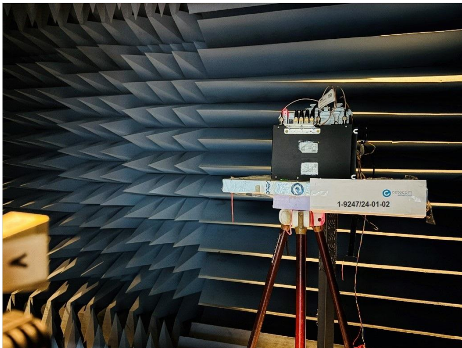
Photograph 4: EUT test setup in the fully anechoic chamber 2, overview_EUT elevation 90°
